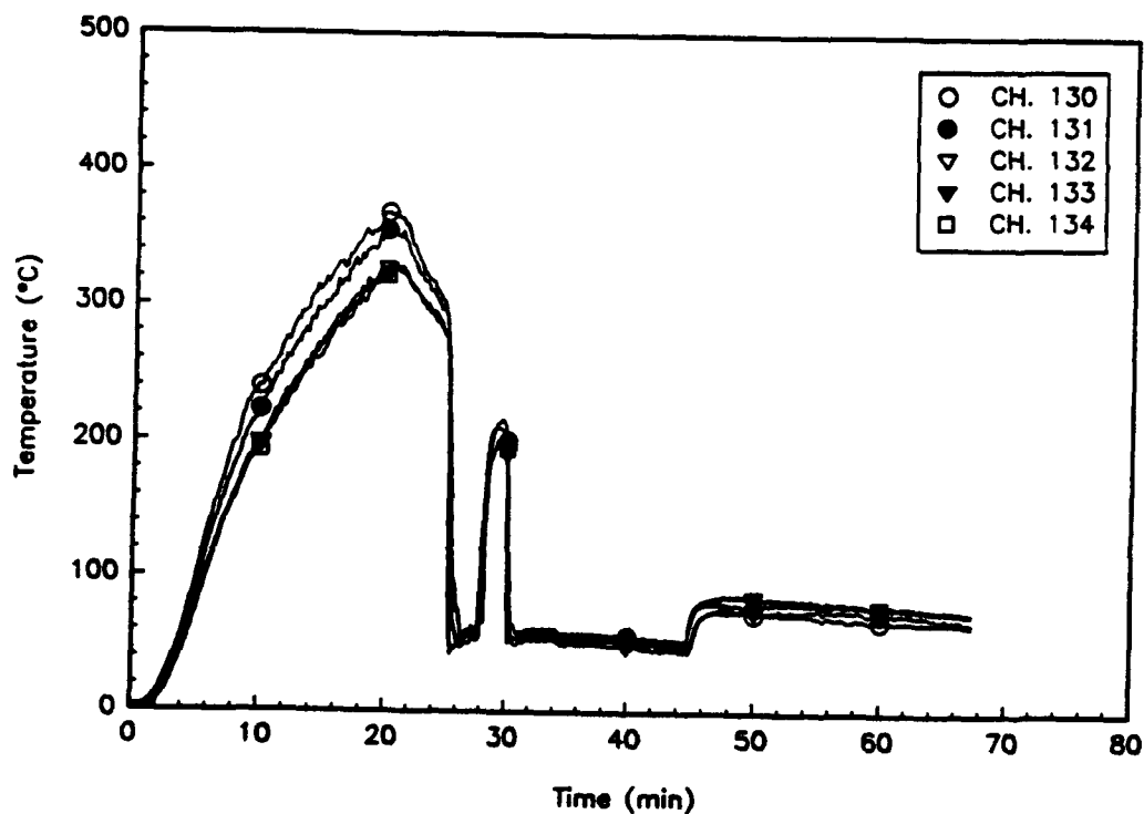
Fig. A173 - RICER 2 air temperature aft, INS_7
