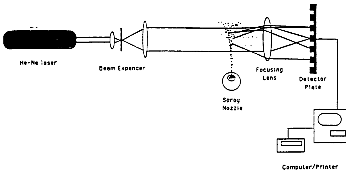
Figure 2 : The basic configuration of the Melvern Droplet and Particle Size Analyser
