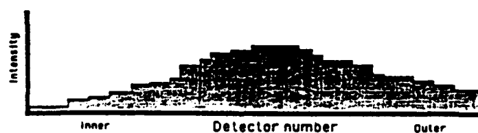
Figure 3c: New distribution after applying correction method described by Dodge and Cerwin
