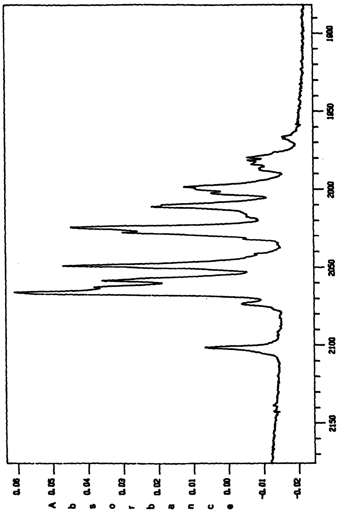
Wavenumber IR SPECTRUM OF COMPOUND I
