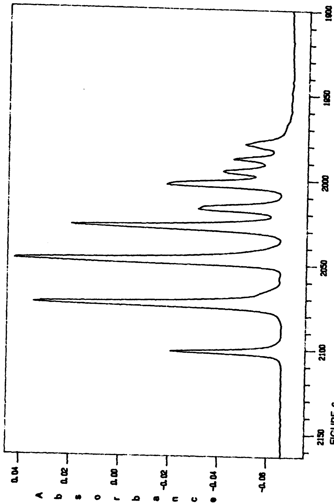
Wavenumber IR SPECTRUM OF COMPOUND III
