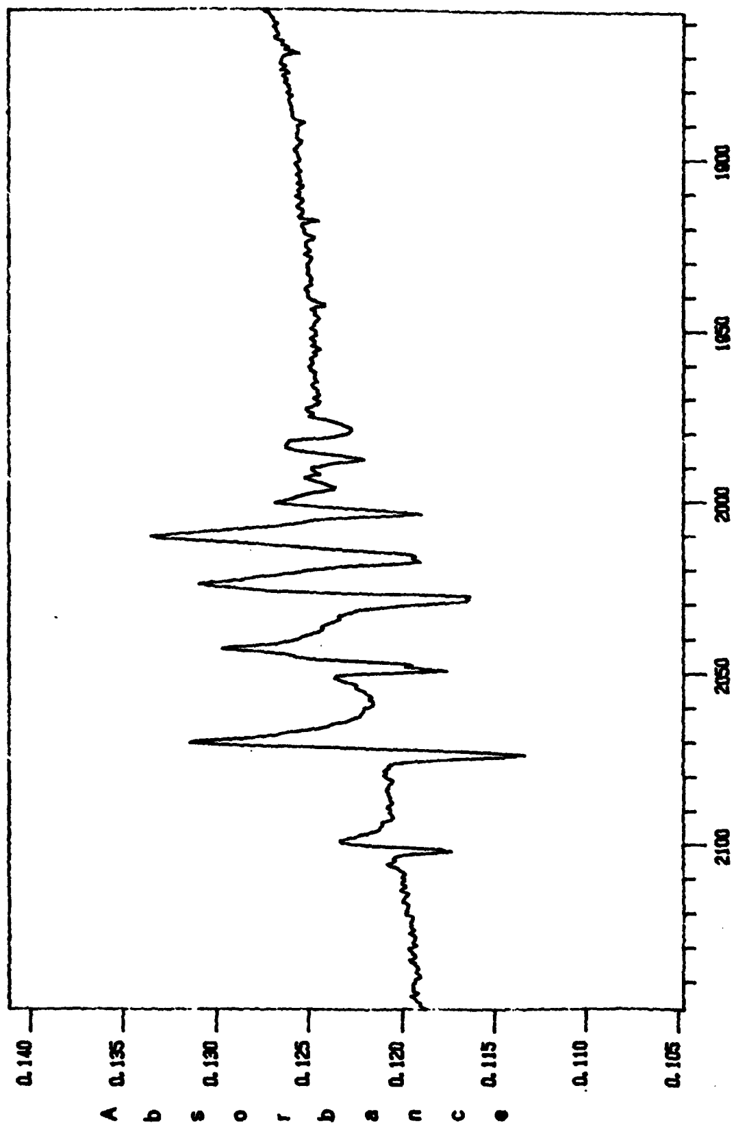
FIGURE 7 DIFFERENCE SPECTRUM OF COMPOUND 16-18 PHOTOLYZED TO GIVE COMPOUND IV
