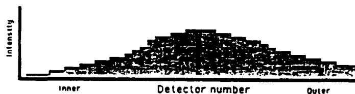
Figure 3a: Normal light scattering intensity signal on detector array, and drop size data.
