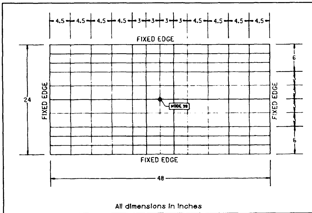
Figure 3.12 COSMOS/M Impact Load Model, a/b = 2.0
