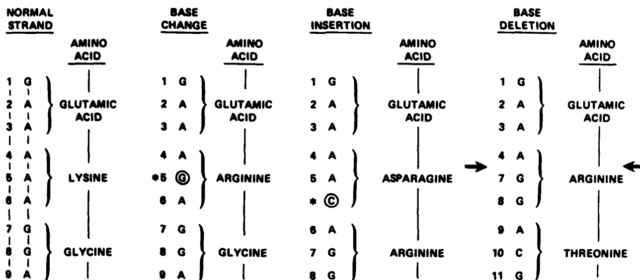
Fig. 9-14. Types of mutations in the gene. One normal strand of DNA (illustrating nine bases within the strand) is shown on the left. These nine bases code for three amino acids within a longer peptide chain. A base change at position 5 from adenine to guanine changes the code for the second amino acid from lysine to arginine. The intercalation of cytosine between positions 5 and 6 changes the codes for the second and third amino acids and for every amino acid in the chain coming after them. Deleting bases 5 and 6 and closing the gap between positions 4 and 7 change the coding for the second and third amino acids and for each amino acid coming after them. Mutations may also occur by inversions (not shown).
