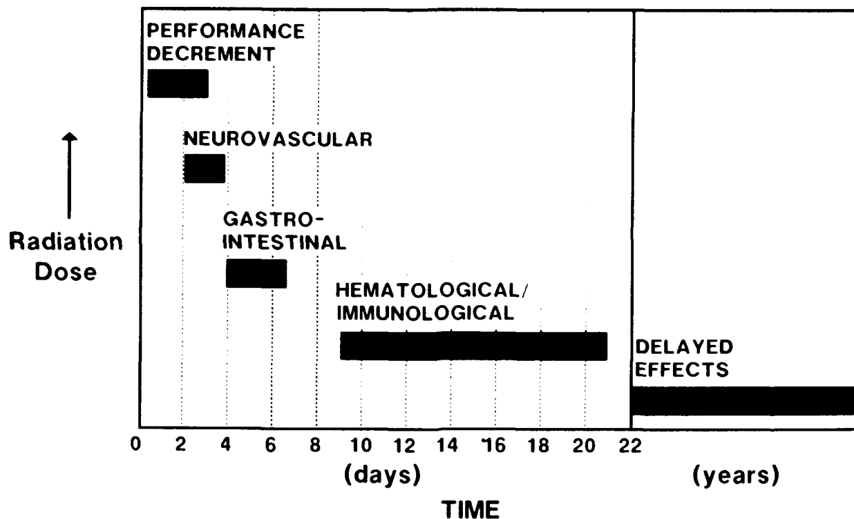
Fig. 2-6. Occurrence of radiation effects in relation to dose and time. As radiation dose increases, time to manifestation of effect decreases.
