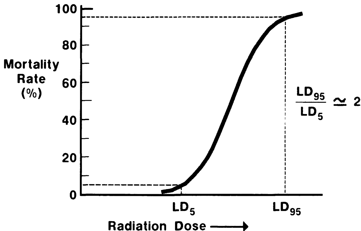
Fig. 2-7. Standard dose-response curve
