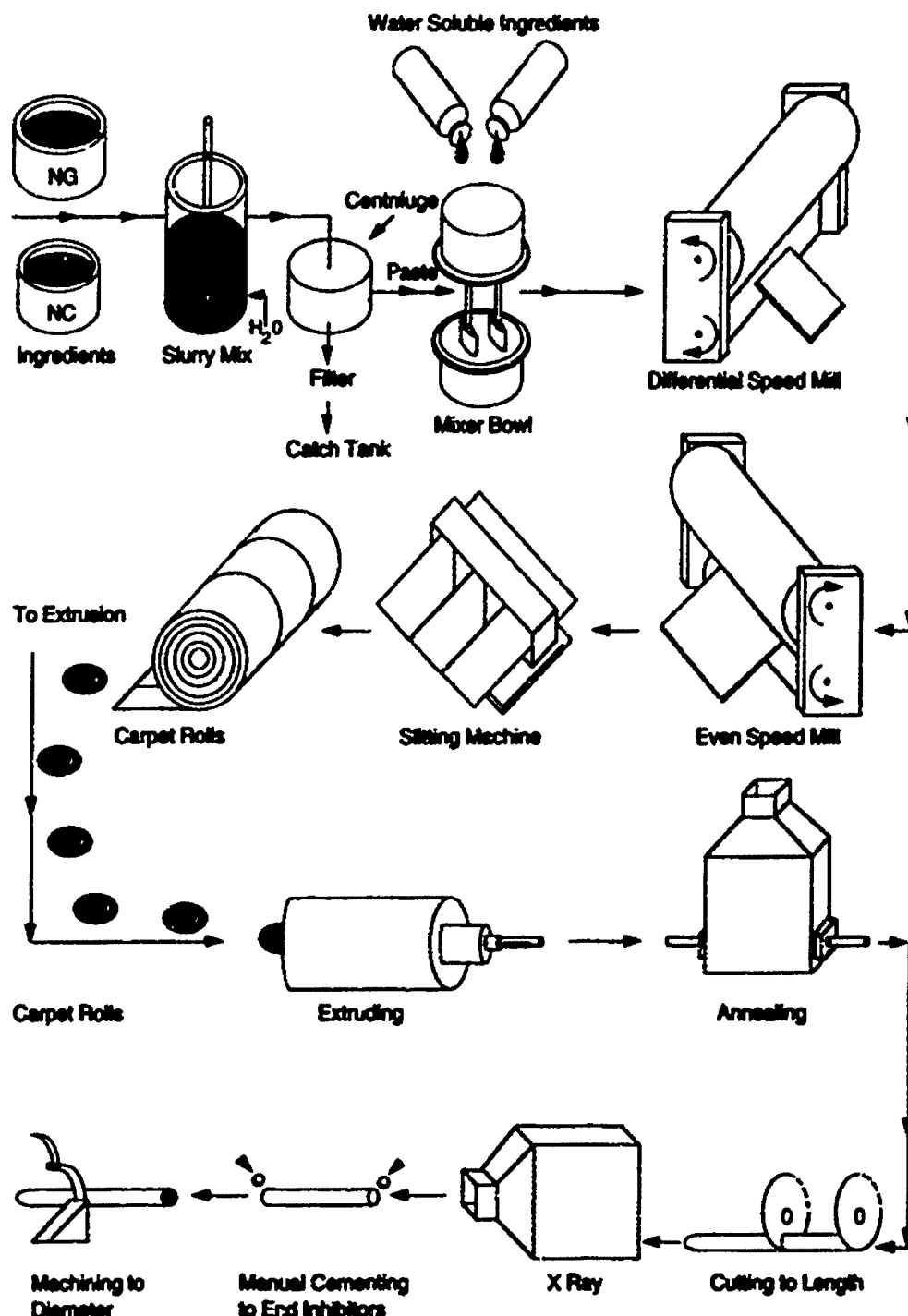
Fig. 9-12. In contrast to the solvent-based process, the solventless process uses no extraneous solvents during mixing. Nitroglycerin (or, less often, another liquid aliphatic nitrate such as EGDN or DEGN) is used to form a colloid with the nitrocellulose. Dissolution does not occur, but rather, the mixing and milling achieve a uniform colloid of the explosives and additives. Milling and extrusion are usually done at warm temperatures, and there is significant exposure potential for inhalation and dermal absorption of nitroglycerin. Reprinted with permission from Chemical Propulsion Information Agency. Gun propellant process operations. In: Hazards of Chemical Rockets and Propellants . Vol 2, Solid Propellants and Ingredients . Laurel, Md: CPIA; 1985: 3-16-3-17. CPIA Publication 394.
