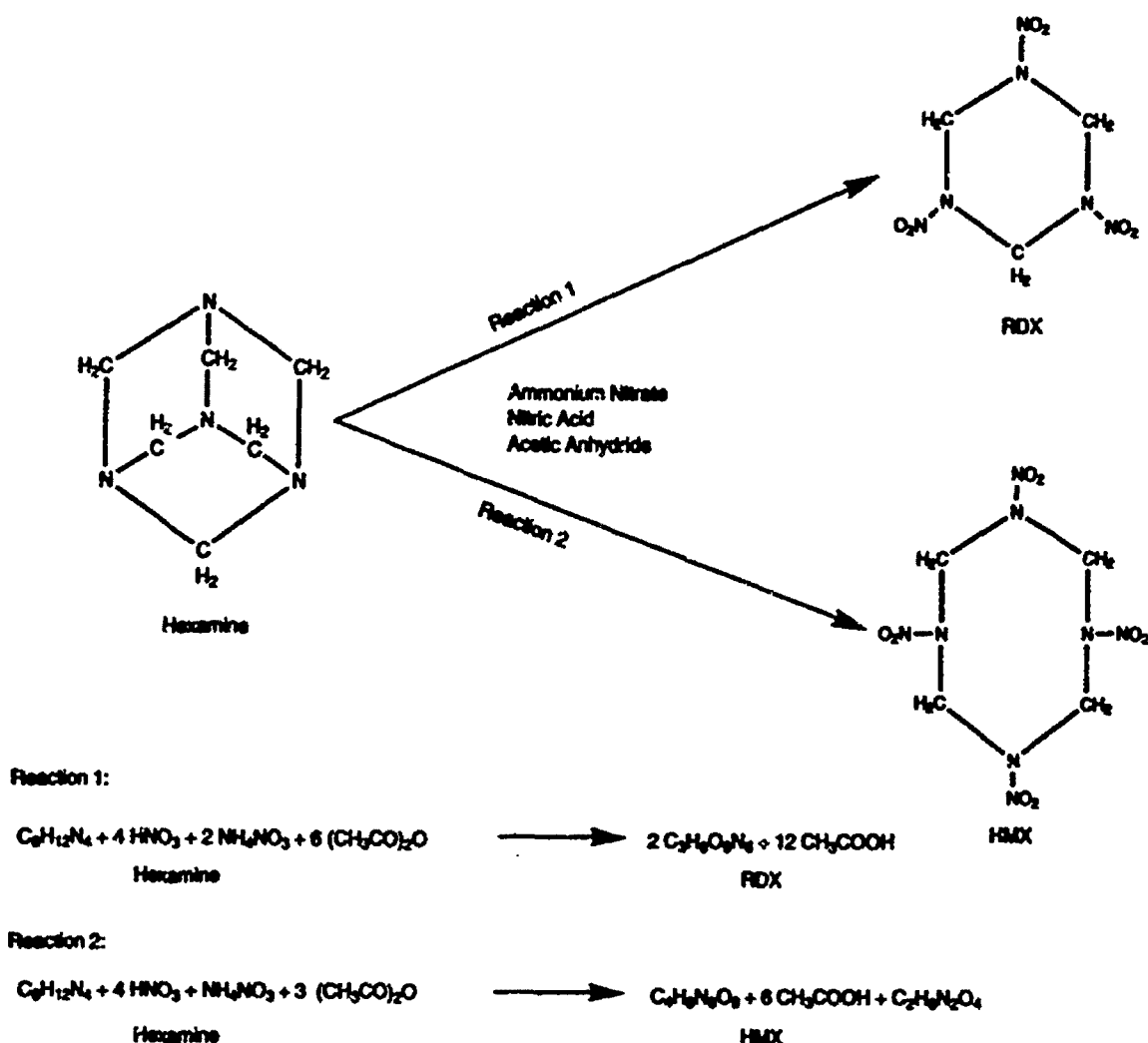
Fig. 9-16. The chemistry of RDX and HMX production. HMX is an unavoidable coproduct of the production of RDX from hexamine. Most RDX preparations contain at least 9% HMX. Reprinted from US Army Environmental Hygiene Agency. Water Pollution Aspects of Explosive Manufacturing . Aberdeen Proving Ground, Md: USAEHA; 1985: 21. USAEHA Technical Guide 140.
