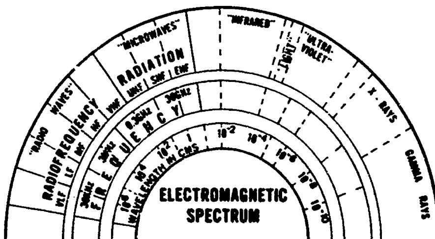
Fig. 15-1. The divisions of the electromagnetic spectrum are arbitrary, overlapping regions on a continuum. The generally accepted divisions are cosmic rays \lambda < 0.005 \text{ \AA} ; gamma rays \lambda 0.005\text{--}1.4 \text{ \AA} ; X rays \lambda 0.1\text{--}100 \text{ \AA} ; ultraviolet (UV) \lambda 40\text{--}400 \text{ nm} ; visible light \lambda 400\text{--}700 \text{ nm} ; infrared (IR) \lambda 700 \text{ nm}\text{--}1 \text{ mm} ; microwave (MW) \lambda 1 \text{ mm}\text{--}1 \text{ m} ; radio-frequency (RF) \lambda > 1 \text{ m} .
