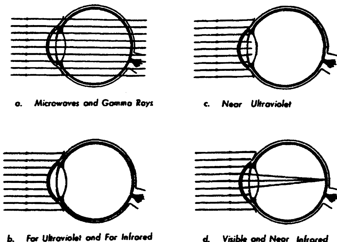
Fig. 15-10. (a) Microwave (MW) and gamma ray radiation can penetrate the human eye with some absorption in all tissues. (b) Far ultraviolet (UV) and far infrared (IR) do not penetrate the eye at all. (c) Near UV penetrates into the anterior portion of the eye, where it can damage the lens and posterior capsule. (d) Visible and near IR are focused by the lens onto the retina, where they can cause retinal damage. Adapted with permission from Slaney DH, Wolbarsht ML. Safety with Lasers & Other Optical Sources . New York: Plenum; 1980.
