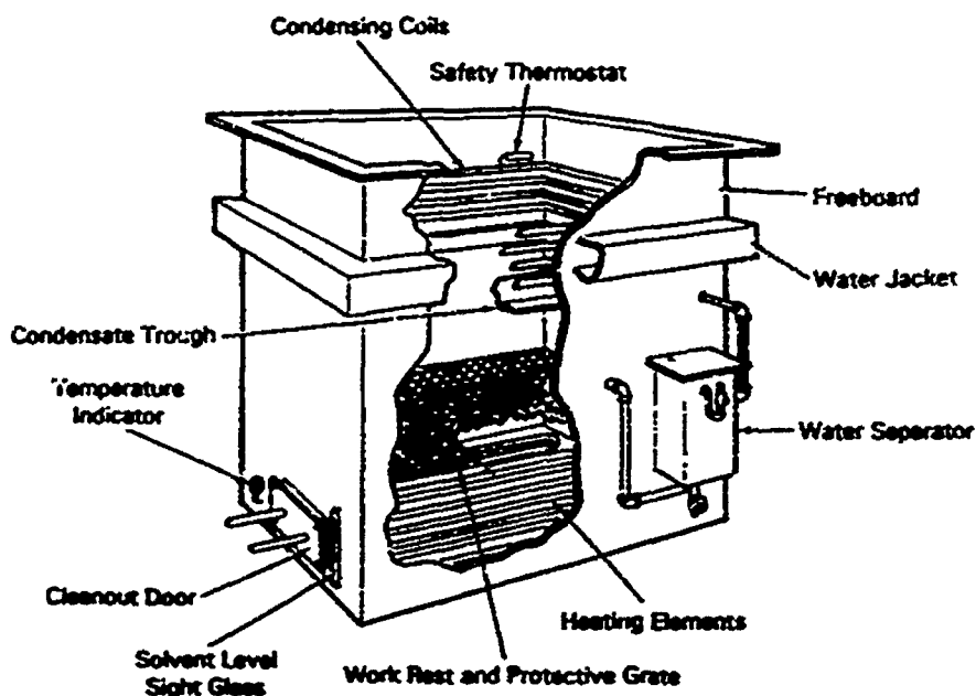
Fig. 13-1. A typical degreasing tank. Vapor degreasing is accomplished by lowering the object to be cleaned into the vapor zone above the liquid solvent. Solvent vapors condense on the cold item and loosen grease and oil, which then collect in the bottom of the tank. Condensing coils located near the top of the tank condense the solvent vapors, which collect in the condensate trough and are returned to the reservoir. The item is held in the vapor zone until the parts reach the temperature of the solvent vapor. At that time, condensation stops and the item is dry.
