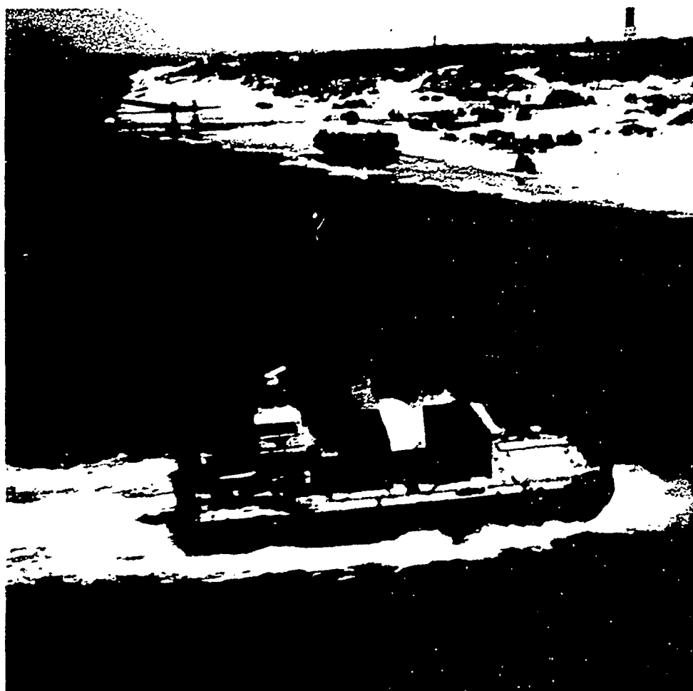
Fig. 6-6. The Lighter Air Cushion Vehicle, 30-Ton Capacity (LACV-30). The LACV-30 is capable of around-the-clock operations regardless of the weather. It easily transports wheeled and tracked vehicles, containers, and bulk cargo on its 1,660 ft 2 deck. Its maximum payload is 75 tons, cruise speed is 45 mph, and endurance is 8 to 10 hours. U.S. Army transportation units received their first production craft in 1982.
