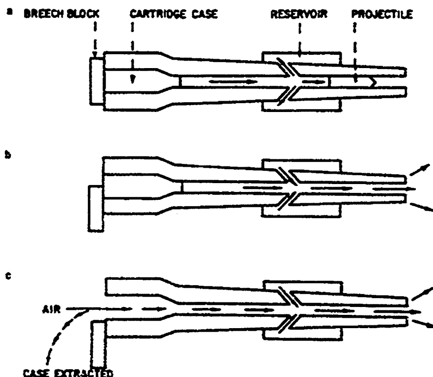
Fig. 10-13. (a) Following the firing of the weapon, gases are drawn into the reservoir as the projectile passes. (b) After the projectile is ejected from the muzzle, the gas previously drawn into the reservoir is expelled from the muzzle. (c) As the breech is opened to eject the cartridge case or reintroduce another round, air from the crew compartment is drawn into the bore and expelled, along with any combustion gas remaining in the reservoir, through the muzzle. Source: Ross RH, Pal BC, Lock S, et al. Problem Definition Study on Techniques and Methodologies for Evaluating the Chemical and Toxicological Properties of Combustion Products of Gun Systems . Vol 1. Oak Ridge, Tenn: Oak Ridge National Laboratory; 1968. Final Report AD-ORNL-6334/V1.
