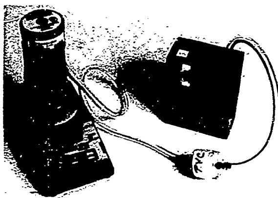
Fig. 4-15. The Gilian Instrument Corporation's Gilibrator Bubble Generator provides an efficient method of determining airflow rates before, during, and after sample collection.
