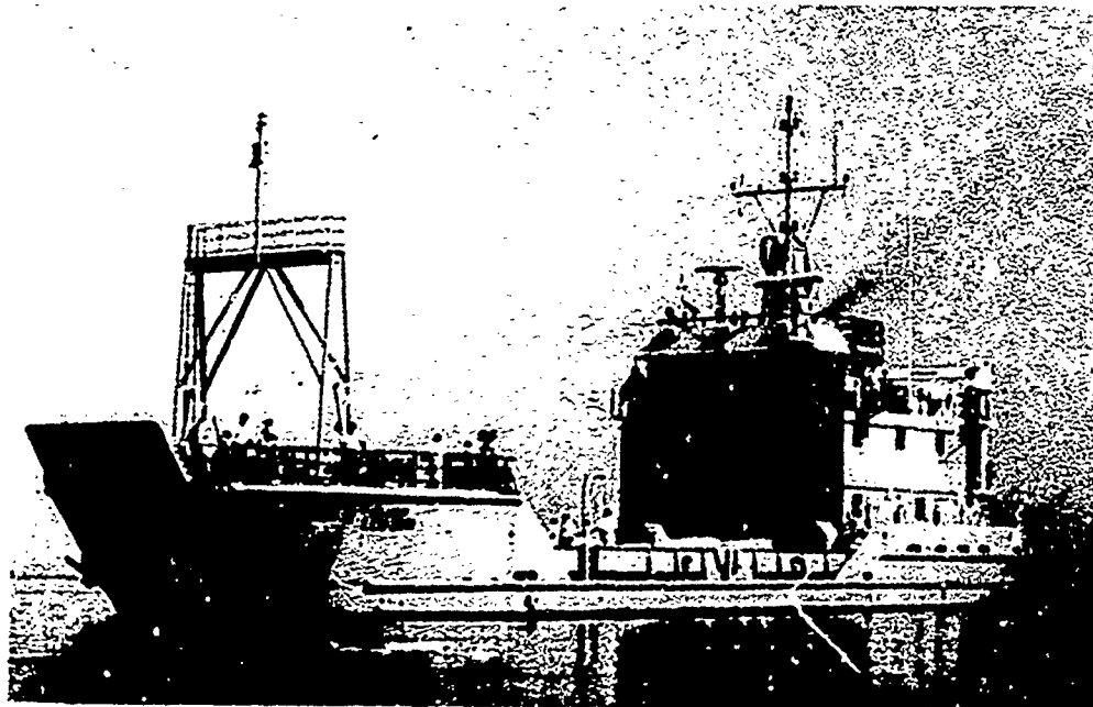
Fig. 6-11. Landing Craft Utility-2000 (LCU-2000). LCU-2000 ships are 174 ft long by 42 ft wide and displace 1,067 tons when fully loaded. Their speed is 12 knots and range is 5,000 miles. The main deck level houses the mess, sick bay, and recreation room. The crew quarters are on the second level; the pilot house is on top. A stern module contains the engine room and associated machinery.
