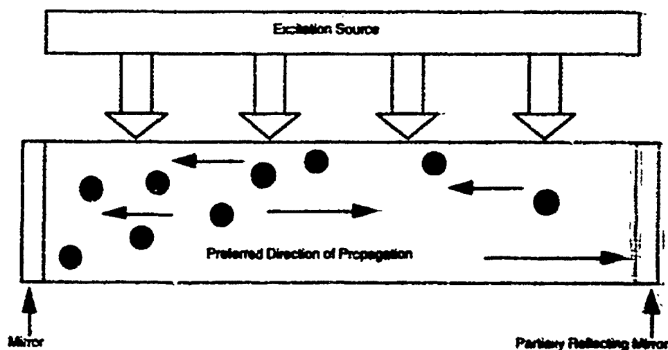
Fig. 15-16. The basic components of a common laser include a lasing medium (or cavity) with a preferred direction of propagation, an excitation source to create a population inversion, and mirrors to amplify the laser beam.
