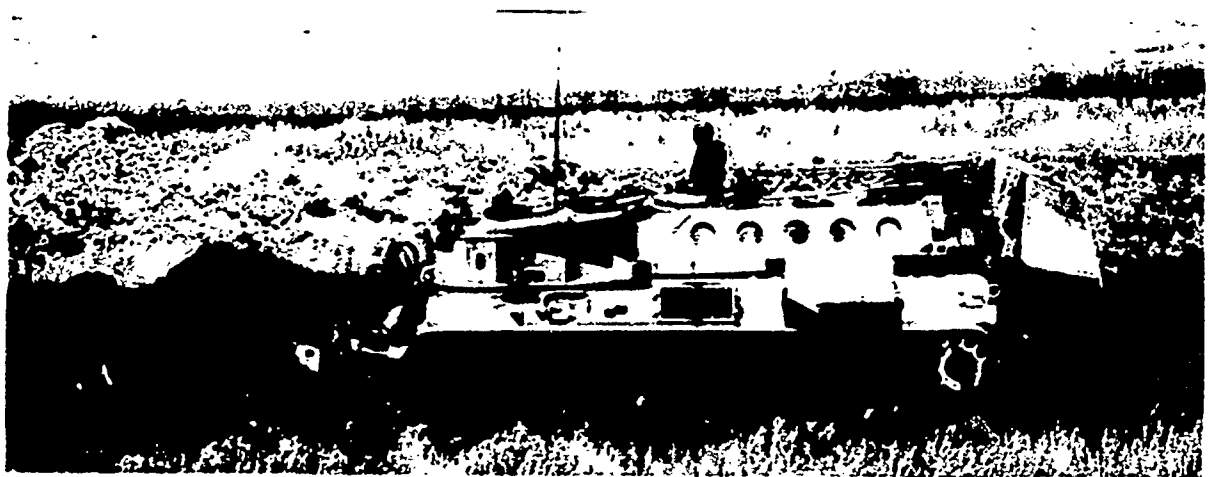
Fig. 6-20. Counterobstacle Vehicle (COV). The prototype COV pictured here is a highly mobile vehicle capable of clearing and creating major obstacles and emplacements. It is equipped with a combination bulldozer/mineplow and two telescopic arms. The arms are normally used with buckets, but can also accept a hammer, auger, lifting hook, grapple, and other attachments. These attachments enable it to move earth, breach minefields, knock down obstacles, dig defilade positions for armored vehicles, and excavate antitank ditches.
