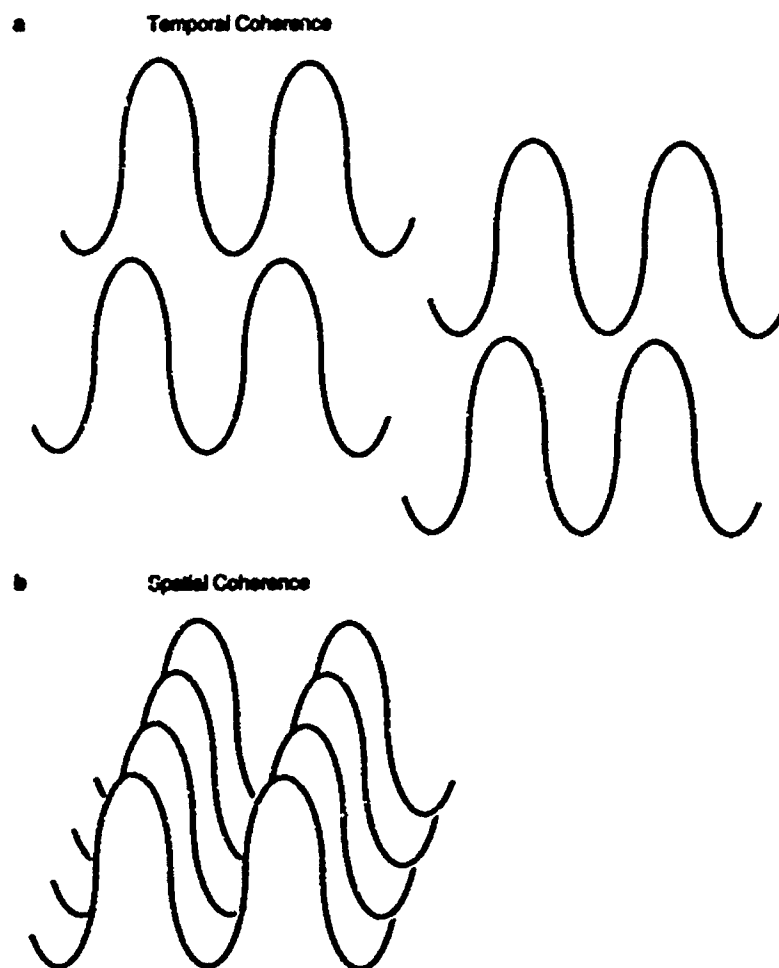
Fig. 15-5. (a) Temporally coherent waves have identical wavelengths, but they are not necessarily in phase (aligned). (b) Spatially coherent waves not only have the same wavelength, they are also all in phase.
