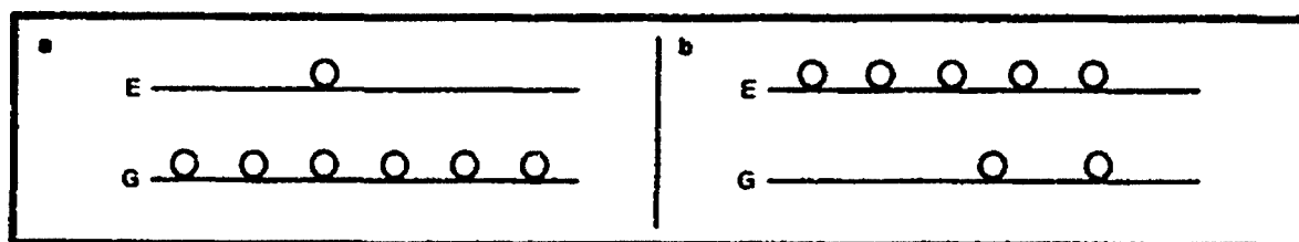
Fig. 15-15. (a) A normal electronic population distribution, where the ground state G is the most populous. (b) An electronic population inversion occurs when the excited state E becomes more populous than the ground state.
