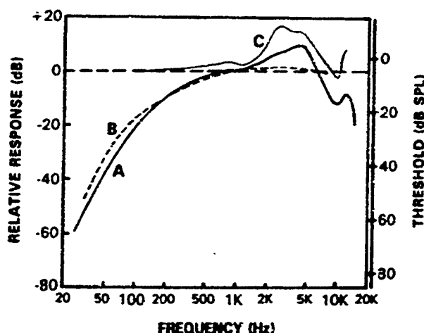
Fig. 7-8. Curve A: Response characteristics of the auditory system. A minimum audibility curve has been inverted as if a frequency-response curve had been "run" on the auditory system (actual thresholds, in dB SPL re 2 \times 10^{-3} N/m 2 , are shown on the right for reference). Curve B: A weighted response curve for sound-level measurement. Curve C: Sound pressure appearing at the eardrum as a function of the pressure in the sound field. Reprinted from Durrant JD. Anatomical and physiologic correlates of the effects of noise on hearing. In: Lipscomb DM, ed. Noise and Audiology . Baltimore: University Park Press; 1978 (out of print). Photograph: Courtesy of John D. Durrant, Philadelphia, Penn.
