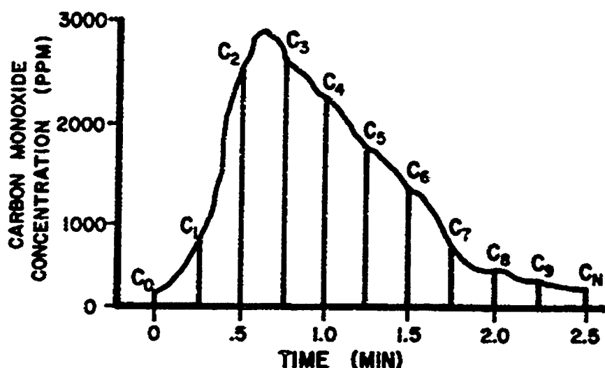
Fig. 10-11. This graphic example, based on actual measurements, shows typical carbon monoxide (CO) concentrations (in ppm) inside the crew compartment of an armored vehicle during a firing mission and the opening of the gun breech. Eleven air samples ( C_0 through C_N ) were obtained at 15-second intervals and analyzed for CO; the data were extrapolated to an expected, continuous concentration curve. The area under the curve may be represented by a definite integral and illustrates the total concentration of CO exposure for a given period of time. Increasing the number of measurement points improves the degree of accuracy in calculating the area. In this example, the firing and environmental conditions resulted in an estimated maximum CO concentration of almost 3,000 ppm at approximately 40 seconds after firing commenced. The ventilation system of the vehicle compartment, and perhaps a breech gas scavenging system, returned the CO concentration to near baseline level in about 2.5 minutes. This example also illustrates high baseline CO levels, exceeding 100 ppm, in the vehicle crew space. During actual field-firing situations, it is not unusual to find several armored vehicles in close proximity with their engines running, executing multiple firing missions. Therefore, high baseline levels may be obtained due to unexhausted CO from an earlier firing mission or CO from a gun muzzle or engine exhaust that has entered the vehicle being studied through an opened hatch or vent. In 1983, CO levels were monitored inside the crew shelters of a battery of M109, 155-mm self-propelled howitzers at Fort Sill, Okla. Firing was conducted with the hatches open; the environmental conditions, especially wind direction and speed, concentrated exhaust products around one particular vehicle in which the carboxyhemoglobin levels in the crew were higher than in crew members of the other vehicles. Sources: (1) Dalton BA, Deeter DP, Gaydos JC. Unpublished data from a field study performed at Fort Sill, Okla, 23-26 April 1983, by the Occupational Medicine Division, USAEHA. (2) US Army Combat Systems Test Activity. US Army Test and Evaluation Command Test Operations Procedure: Toxic Hazards for Vehicles and Other Equipment . Aberdeen Proving Ground, Md: DA; 1984. Report TOP 2-2-614. (3) Lucas TA. Methodology Investigation of Toxic Gas Measurements During Weapons Firings from Vehicles While Moving: Final Report . Aberdeen Proving Ground, Md: US Army Test & Evaluation Command. TECOM Project 7-CO-PB9-AP1-002; 1984. Report APG-MT-5896. (4) Dalton BA. Carbon monoxide in US Army tactical vehicles. Medical Bulletin of the US Army Medical Department . 1988;2:11-13. PB 8-88.
