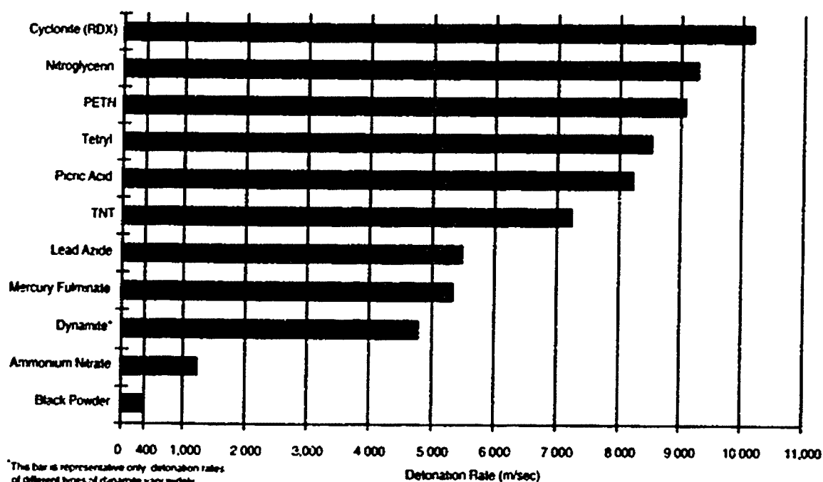
Fig. 9-1. Approximate detonation rates of common military and industrial explosives. Infinite variations on these rates are possible by mixing and by using additives. Both explosive and propellant formulations have taken advantage of these high detonation rates. Adapted with permission from Meidl JH Explosive and Toxic Hazardous Materials . New York: Macmillan Publishing; 1970: 24
