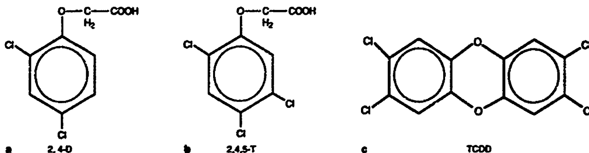
Fig. 14-2. Agent Orange. The chemical structures of the herbicides (a) dichlorophenoxyacetic acid (2,4-D) and (b) 2,4,5-trichlorophenoxyacetic acid (2,4,5-T); (c) represents the structure of the undesirable intermediate dioxin contaminant 2,3,7,8-tetrachlorodibenzo- p -dioxin (TCDD).
