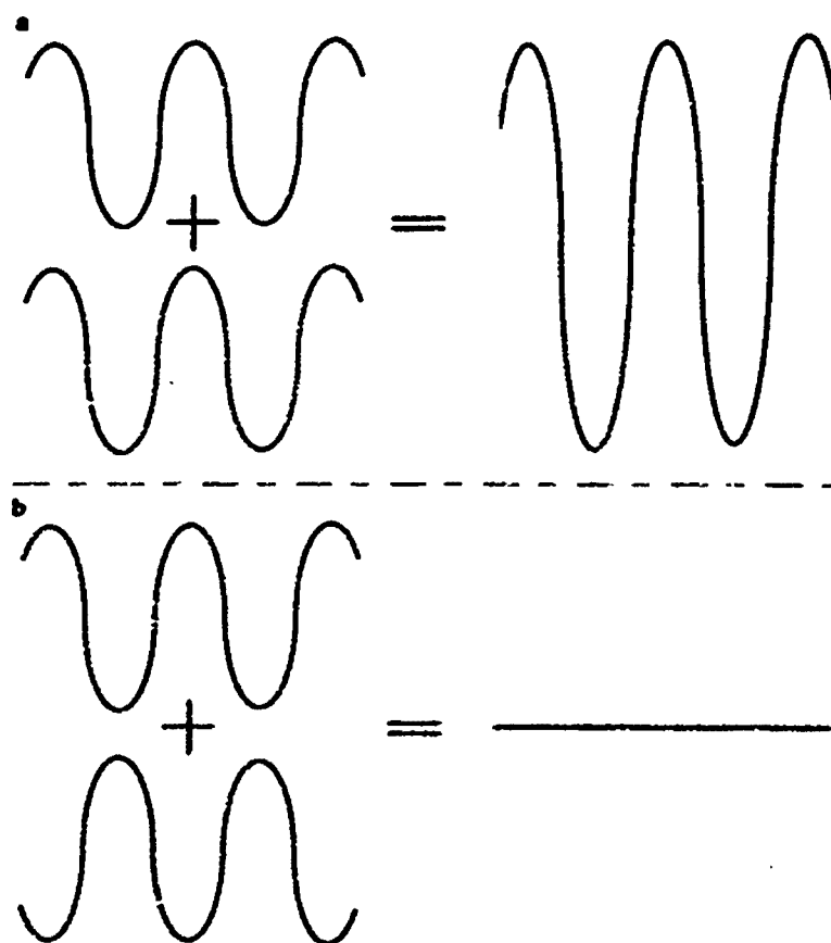
Fig. 15-4. Constructive and destructive interference. (a) Two waves that are in phase, in which peaks match with peaks, can be combined to produce a wave the amplitude of which is the sum of the peaks. (b) Two waves that are out of phase can nullify each other. Note that these waves are precisely in or out of phase. Waves only slightly out of phase will result in other types of waves.
