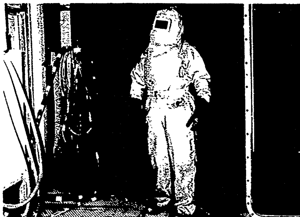
Fig. 12-12. Cumbersome protective gear (including a respirator, hooded chemical-resistant suit, gloves, and boots), worn for prolonged periods of time in sandblasting operations, imposes both physiological and psychological demands on the worker. Excessive physiological demands often manifest as heat stress. The inability to tolerate the psychological demands may manifest as anxiety or claustrophobia. Source: US Army, Anniston Army Depot, Anniston, Ala.
