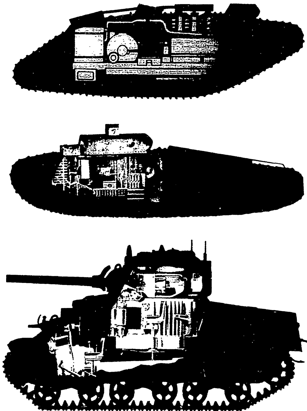
Fig. 1-7. Cutaway drawings of the British Mark IV combat tank of World War I (upper), the British Mark VIII (center), which appeared around the end of World War I, and the Sherman M4 (lower), which was used extensively during World War II. The light areas represent the crew compartments. After only a few years' experience, designers of the Mark VIII placed a bulkhead between the engine and the remainder of the tank interior that, at least theoretically, would reduce crew exposure to engine exhaust products, petrol vapors, engine heat, and engine fires. The concept of a separate engine compartment was incorporated into World War II tanks, but crew exposure to combustion products of weapons continues even to the present. Original drawings by Leon Conjour, USAEHA Illustration Shop.
