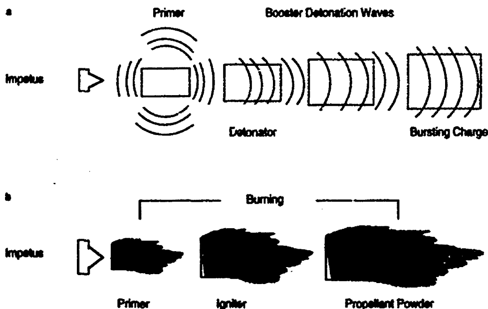
Fig. 9-4. Comparison of explosive train with ignition train. Although significant engineering differences exist between explosive trains (a) and ignition trains (b), in concept they are very similar. In both, a small electrical or mechanical stimulating impetus is magnified via a succession of intermediate charges to achieve optimum initiation of the main charge or propellant grain. The major difference between the two types of chains is in the component charges' rates of reaction. Adapted from US Department of the Army. Military Explosives . Washington, DC: DA; 1985. Technical Manual 9-1300-214, September 1984 with change 1 of 30 November 85.
