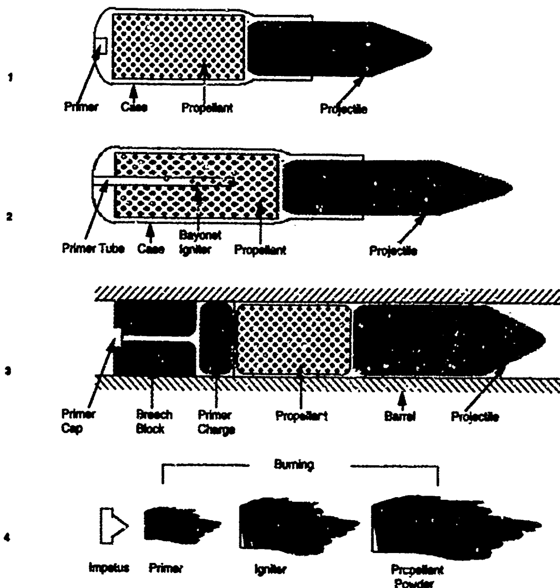
Fig. 10-5. Drawings 1, 2, and 3 show the general configurations of primer, igniter, and propellant mixes in typical ammunition. Drawing 4 is a schematic representation of the firing sequence in typical ammunition, usually referred to as the "explosive train" or the "ignition train." A small electrical and/or mechanical (percussion) stimulating impetus is intensified through a succession of intermediate charges to obtain optimum firing of the main charge, the propellant. The "ignition train" typically consists of four steps: stimulating impetus, primer burning, igniter burning (shown only in drawings 2 and 3) and propellant burning. Igniters are not generally placed in small-caliber ammunition (drawing 1) but are found in the bayonet igniter of tank gun rounds (drawing 2) and in close association with the propellant in artillery rounds (drawing 3). Igniter mixes are generally not used in rocket propulsion motors. Propellants are "low explosives" in that they burn relatively slowly (400 m/sec or slower) at a sustained rate. In contrast, "high explosives" like dynamite detonate at 1,000 to 10,000 m/sec producing a sudden, powerful shock wave. Sources: (1) Farrar CL, Leeming DW. Military Ballistics—A basic manual . Ft. Snelling Weapons Systems and Technology Series, Vol 10. Oxford, England: Brassey's Pub Ltd; 1963. (2) US Department of the Army. Military Explosives . Picatinny Arsenal, NJ: AMCCOM; 1984. Technical Manual 9-1300-214. (3) Ross RH, Pal DC, Lock S, et al. Problem Definition Study on Techniques and Methodologies for Evaluating the Chemical and Toxicological Properties of Combustion Products of Gun Systems . Vol 1. Oak Ridge, Tenn: Oak Ridge National Laboratory; 1988. Final Report AD-ORNL-6334/V1. (4) Ciccone JG. Primers. In: Kaye SM, ed. Encyclopedia of Explosives and Related Items . Vol 8. Dover, NJ: US Armament Research and Development Command; 1976: 372-387.
