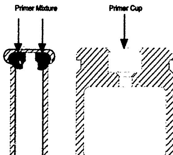
Fig. 10-7. Percussion primers in military ammunition may be either rimfire (left) or centerfire (right). In the rimfire model, the primer energetic material is placed around the rim of the base of the shell casing. The firing pin strikes the rim of the metal casing and the percussion force starts the burning of the primer. Rimfire primers are generally restricted to 0.22-mm caliber ammunition, which is extensively used in commercial sporting ammunition, and is also used by the military to a limited degree for training purposes. In centerfire ammunition, the box or cup containing the primer is located in the center of the base of the shell. The figure above is a representative centerfire box, but there are many varieties of centerfire percussion-box configurations. The metal used to make the cup may be a brass alloy (70% copper and 30% zinc) or some other metal or alloy that will provide the desired sensitivity to the applied percussion force. Adapted from Calzone IQ. Primers. In: Kaye SM, ed. Encyclopedia of Explosives and Related Items . Vol 8. Dover, NJ: US Armament Research and Development Command; 1978: P372-P387.
