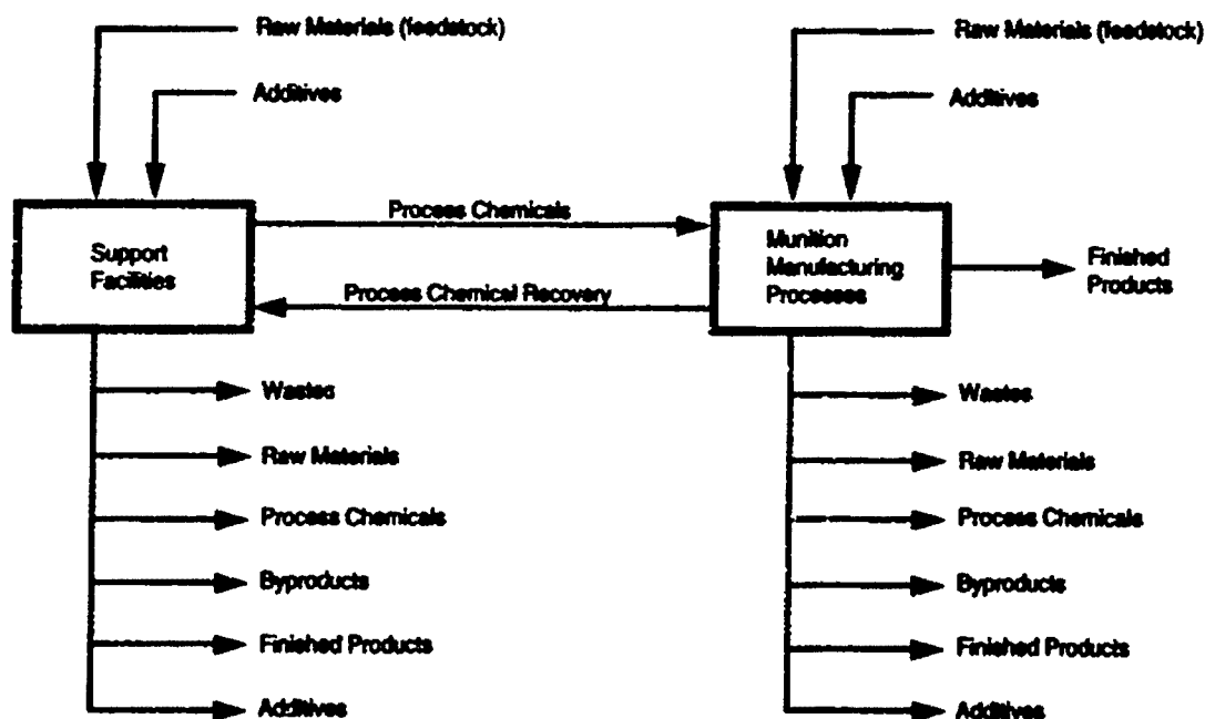
Fig. 9-5. Simplified flow for munition manufacturing processes. Adapted from US Army Environmental Hygiene Agency. Water Pollution Aspects of Explosive Manufacturing . Aberdeen Proving Ground, Md: USAEHA; 1985: 5. USAEHA Technical Guide 140.
