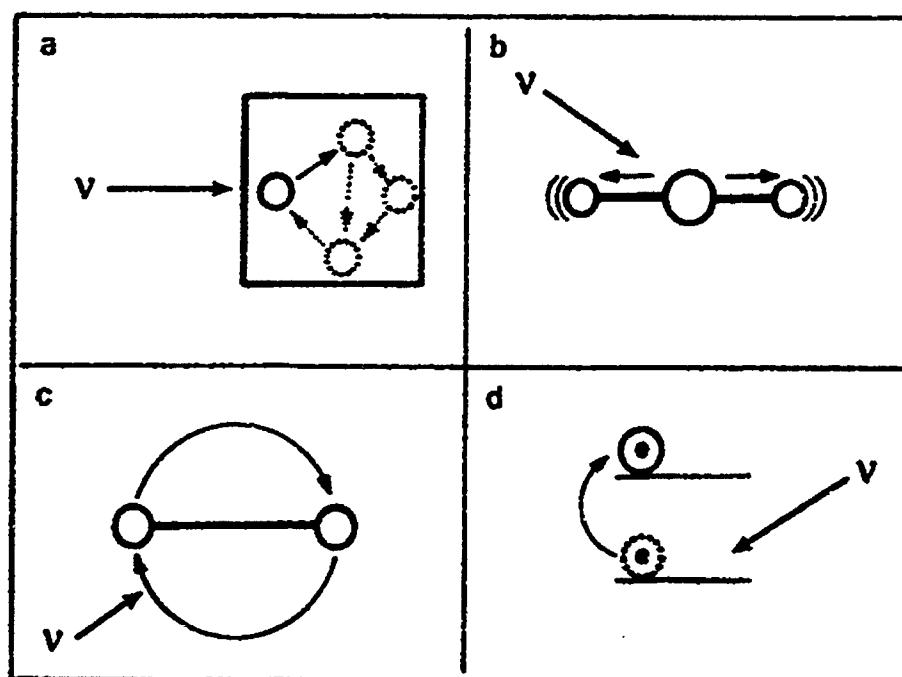
Fig. 15-7. Radiation interacts with matter and its energy is absorbed in several modes; in this drawing, v represents the incident radiation. (a) In the thermal mode, the radiation is absorbed by an atom, which then begins to move about its locus within the molecular lattice of the medium. (b) In the vibrational mode, radiation is absorbed and results in vibrations between neighboring atoms within a molecule. (c) In the rotational mode, energy is absorbed by polar molecules, which reorient themselves relative to local electric fields within the medium, storing energy. (d) In the electronic mode, electromagnetic radiation is absorbed by electrons, raising them to higher orbitals, storing energy that can be reradiated when the electrons return to their original energy state.
