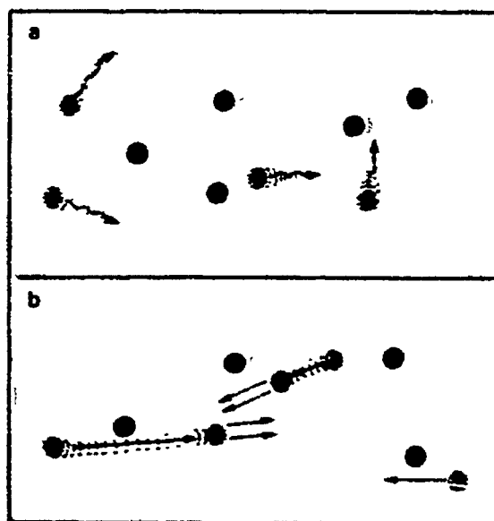
Fig. 15-14. (a) Spontaneous emission occurs when an excited system drops to a lower energy state and emits a photon. This process occurs by itself and the departing photon has no preferred direction. (b) Stimulated emission occurs after collision with a photon. The two emitted photons leave in exactly the same direction and with the same energy.
