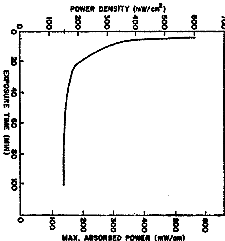
Fig. 15-9. Using 2450 MHz of radio-frequency radiation, the minimum power density required to induce a cataract in the eye of the rabbit is greater than 100 mW/cm 2 (the specific absorption rate is 4.0 W/kg). Reprinted with permission from Guy AW, et al. Effects of 2450 MHz radiation on the rabbit eye. IEEE Transactions on Microwave Theory and Techniques . T-MTT, 1975;23(6):495. © 1975 IEEE.
