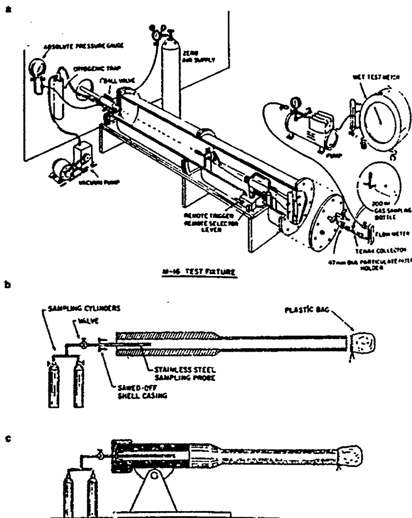
Fig. 10-8. Laboratory sampling systems for identifying propellant combustion products. The enclosure for studying emissions from the M16 rifle, shown in (a), was 6 ft x 11.75 in and contained 133 L. The chamber was Teflon coated to minimize gas absorption and was kept tight with O-ring seals and valves. After firing, chamber contents were evacuated and analyzed. The tank gun system was constructed in a bunker. A manifold for collecting specimens was connected to an adapter, which was a sawed-off shell casing. After firing, the end of the firing tube was covered, the spent shell casing was removed, and the sawed-off shell casing with manifold collection tube was inserted. In (b), the collection device is being inserted; in (c) it is fully inserted. Specimens were collected in the sampling cylinders. Source: Ase P, Eisenberg W, Gordon S, Taylor K, and Snelson A. Propellant combustion product analyses on an M16 rifle and 105-mm caliber gun. J Environ. Sci Health . 1985;A20(3):337-368.
