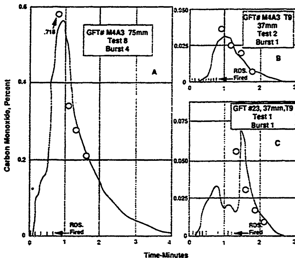
Fig. 11-3. Carbon monoxide concentrations are measured by means of a continuous recorder (—) and grab samples (o) after firing five rounds from the 75-mm gun, A, or ten rounds from the 37-mm gun, B, of the M3A4 tank. (Note that these graphs, which were originally published in 1945, contain an apparent misprint: the tank is identified as an M4A3. Because the data refer to both 37-mm and 75-mm guns, however, we know that the correct designation would be M3A4. The GFT seen in the test-identification boxes may have stood for gas firing test.) In both these graphs, the recorder did not show the true peak as measured by the grab samples. This is due to the relatively slow response time inherent in real-time monitors, which results in an "averaging" effect, and is to be expected. Source: Adapted from Nelson N. NDRC Infra-Red Gas Analyzer for Carbon Monoxide . Fort Knox, Ky: Armored Medical Research Laboratory, 1945. Provided by Alexandria, Va: Defense Technical Information Center. Report AD 655578.
