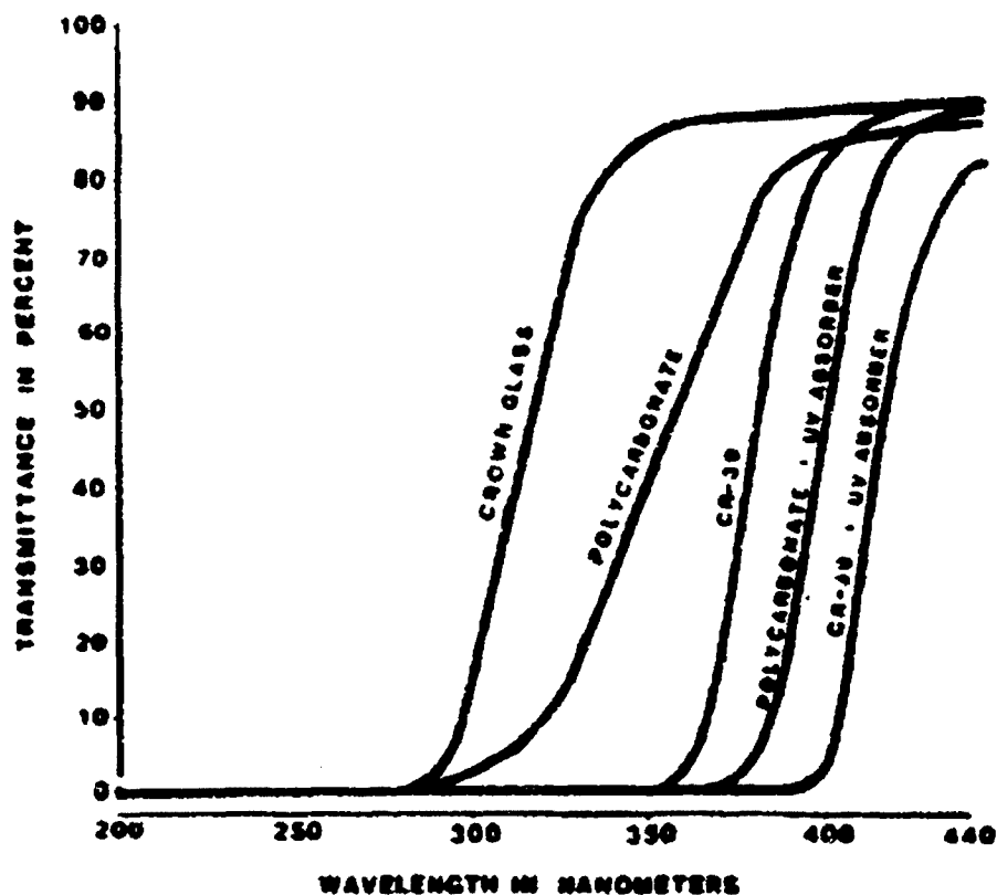
Fig. 8-34. Transmittances of different optical materials used to manufacture spectacle lenses. Source: Pitts DG. Ultraviolet protection, when and why? Prob in Optom. 1990;2(1):95-115.
