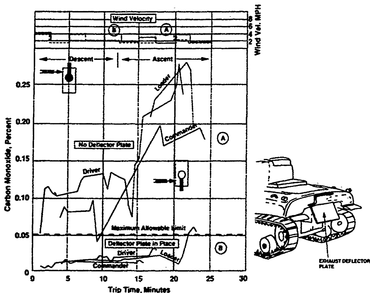
Fig. 11-4. Carbon monoxide was measured at three crew locations when a tank was towed by an M32B1 recovery vehicle with and without an exhaust deflector, and using a towing bar on a 4% grade. Placing an exhaust deflector (small drawing), as a product improvement on the towing vehicle, reduced the concentration of carbon monoxide within the tank. This graph conveys some of the complexity of making field determinations of carbon monoxide exposures. Many variables, if not controlled, must at least be accounted for (eg, wind direction and speed, engine speed, degree of surface grade, duration of the experiment, the location of the monitoring instruments within the tank, the reliability of the instruments). The increased concentration of carbon monoxide seen during observation A may be due to a combination of engine speed, the 4% grade, and the elapsed time. The missing tracing at the loader position in observation A may be due to equipment malfunction. What this graph clearly demonstrates, however, is that attaching an exhaust deflector plate to the rear of the towing vehicle—a seemingly minor modification made for observation B—significantly lowers the concentration of carbon monoxide at the crew positions. Source: adapted from Nelson N. NDRC Infra-Red Gas Analyzer for Carbon Monoxide . Fort Knox, Ky: Armored Medical Research Laboratory; 1945. Provided by Alexandria, Va: Defense Technical Information Center Report AD 655578.
