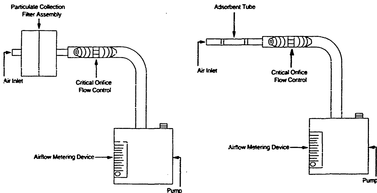
Fig. 4-9 Both these sampling trains for chemical collection use an air-sampling pump without constant flow capability. Flow control can be accomplished with valves or critical air-flow orifices. Control is required to ensure that the exact volume of air collected can be calculated. Without precise flow control, clogged collection devices or variable air pump speed caused by voltage fluctuations could cause a large measurement error. Air pumps are necessary to power the sampling train. Flow from the pump must be calibrated with the entire unit connected as if it were in actual use. This arrangement allows the system to be adjusted to overcome the resistance to air flow found in each separate component of the sampling train. A constant flow pump that uses electronic flow devices can be seen in Figure 4-11.
