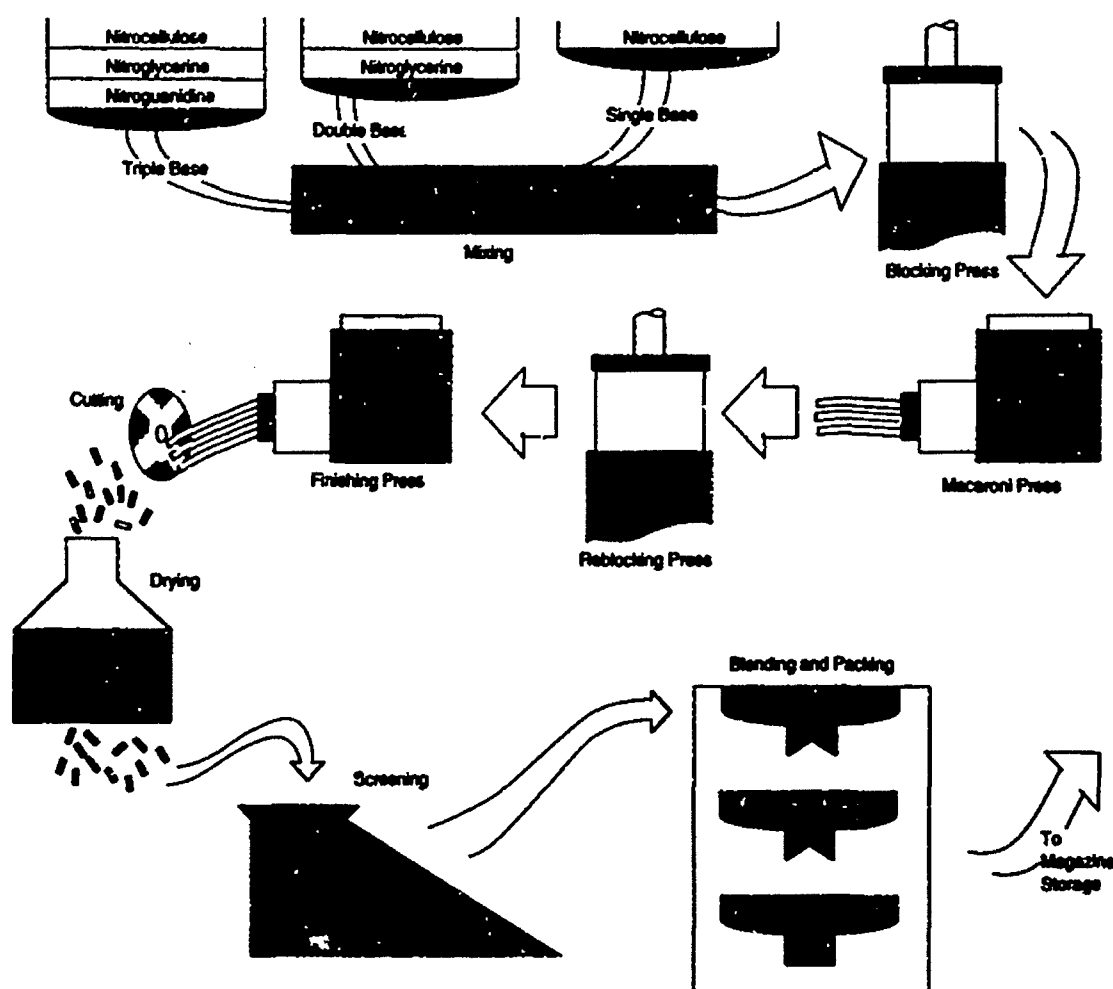
Fig. 9-11. In the solvent-based process of propellant production, the initial mixing is conducted in an alcohol-ether solution, which is then removed via the series of presses. Most production plants prepare these propellants in batches, and utilize manual labor at each step. Reprinted with permission from Chemical Propulsion Information Agency. Gun propellant process operations. In: Hazards of Chemical Rockets and Propellants . Vol 2, Solid Propellants and Ingredients . Laurel, Md: CPIA; 1965: 3-15. CPIA Publication 394.
