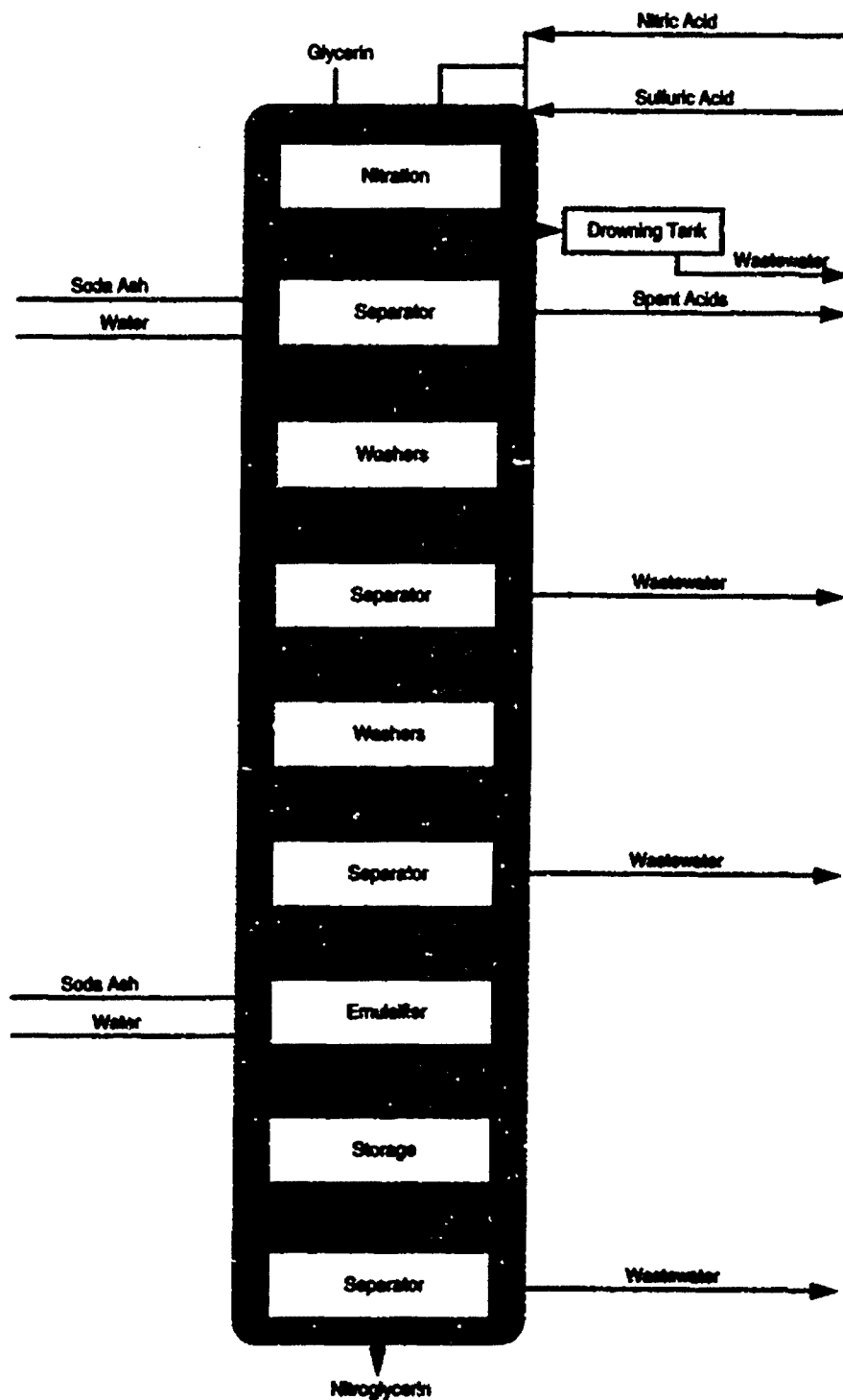
Fig. 9-18. In the Biazzini (continuous-flow) method of manufacturing nitroglycerin, all processes except the drowning tank are completely enclosed within stainless steel reaction vessels, which are connected by stainless steel pipes. Remote control is accomplished via gauges and closed-circuit television. Even the raw materials, wastewater, and nitroglycerin are piped into and out of the process, further limiting potential exposures of the workers. Adapted from US Army Environmental Hygiene Agency. Water Pollution Aspects of Explosive Manufacturing . Aberdeen Proving Ground, Md: USAEHA; 1985: 42. USAEHA Technical Guide 140.
