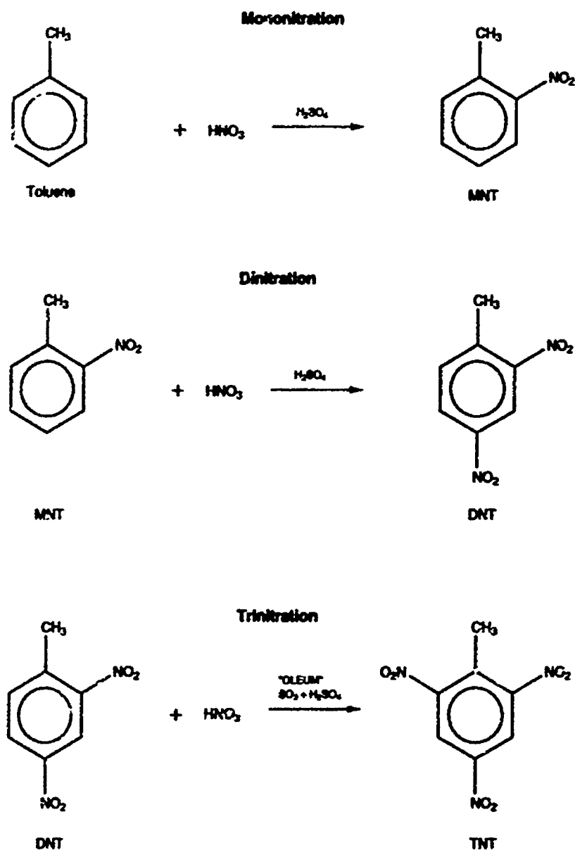
Fig. 9-14. The trinitration of toluene: (a) chemical synthesis and (b) industrial (enclosed) process stream. In the manufacture of TNT, toluene is first reacted with nitric acid to form mononitrotoluene (MNT), which is then pumped to another area, where it is reacted with nitric acid (under different reaction conditions) to form dinitrotoluene (DNT). The DNT is then pumped to yet another area where it is reacted with oleum (a solution of sulfur trioxide dissolved in sulfuric acid) to form TNT.
