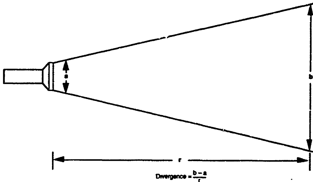
Fig. 15-2. Divergence can be measured as the change in the diameter of the beam divided by the distance of propagation.
