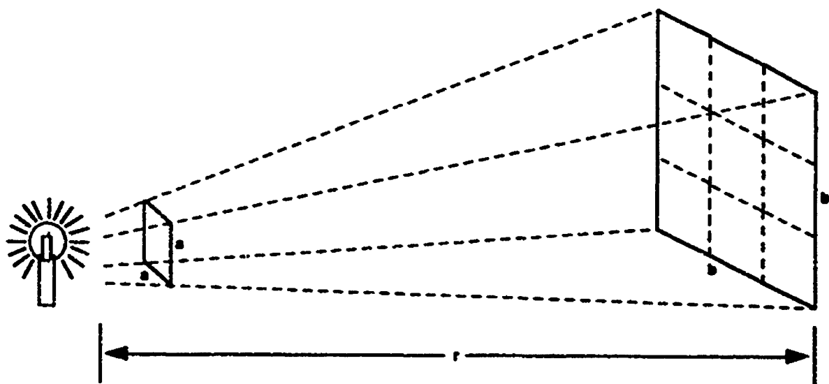
Fig. 15-3. When the distance from an isotropic em. increases by 3-fold, the light fills a 9-fold greater area. Inversely, the amount of light falling on a given area decreases by \frac{1}{9} (the Inverse Square law).
