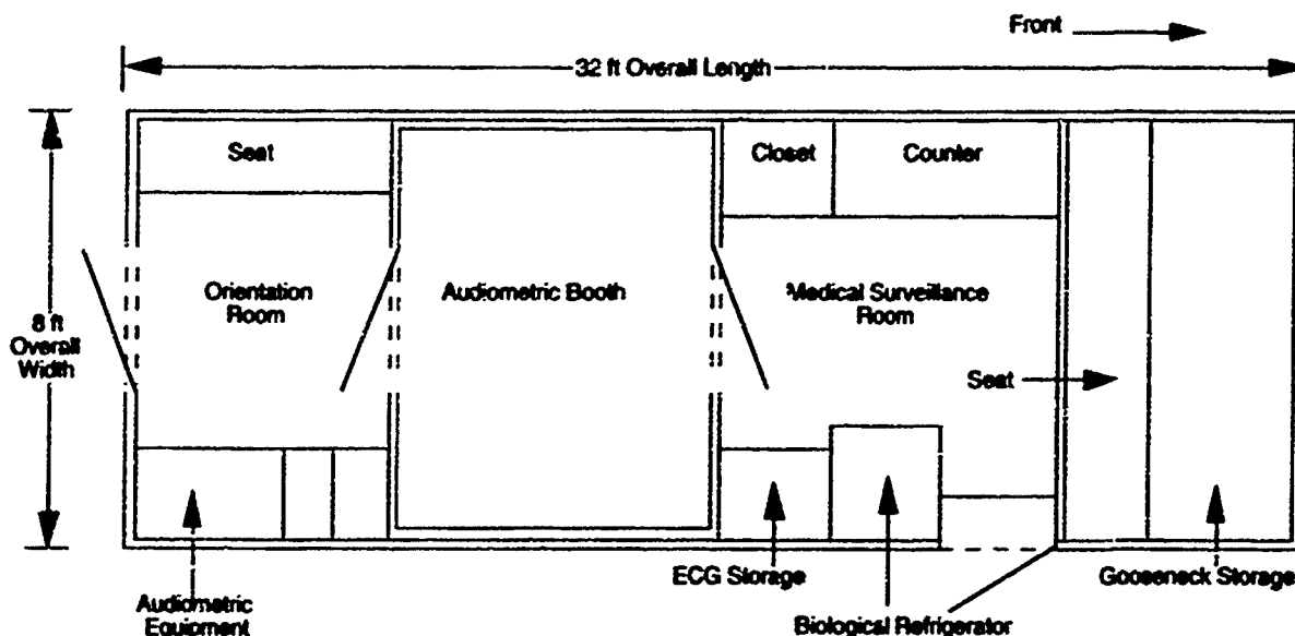
Fig. 7-27. An aerial view of the floor plan for the Military Occupational Health Vehicle (MOHV). When the MOHV is used exclusively for audiometric monitoring, six people can occupy the audiometric booth. Six others can be fitted with earplugs and briefed on hearing-conservation measures in the orientation room. Photograph... Courtesy of the US Army Environmental Hygiene Agency, Aberdeen Proving Ground, Md, 1991.
