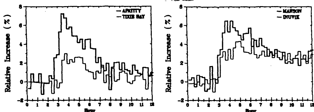
Figure 1. The 11 June 1991 GLE as observed by selected high latitude neutron monitors. Left: Apatity, Russia (forward viewing) and Tixie Bay, Russia (reverse viewing). Right: Mawson, Antarctica (forward viewing) and Inuvik, Canada (reverse viewing).
