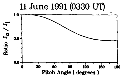
Figure 4. Solar particle flux pitch angle distribution necessary to produce the observed variation in the high energy solar proton flux at high latitude neutron monitors at the 0330 UT maximum of the 11 June 1991 GLE.
