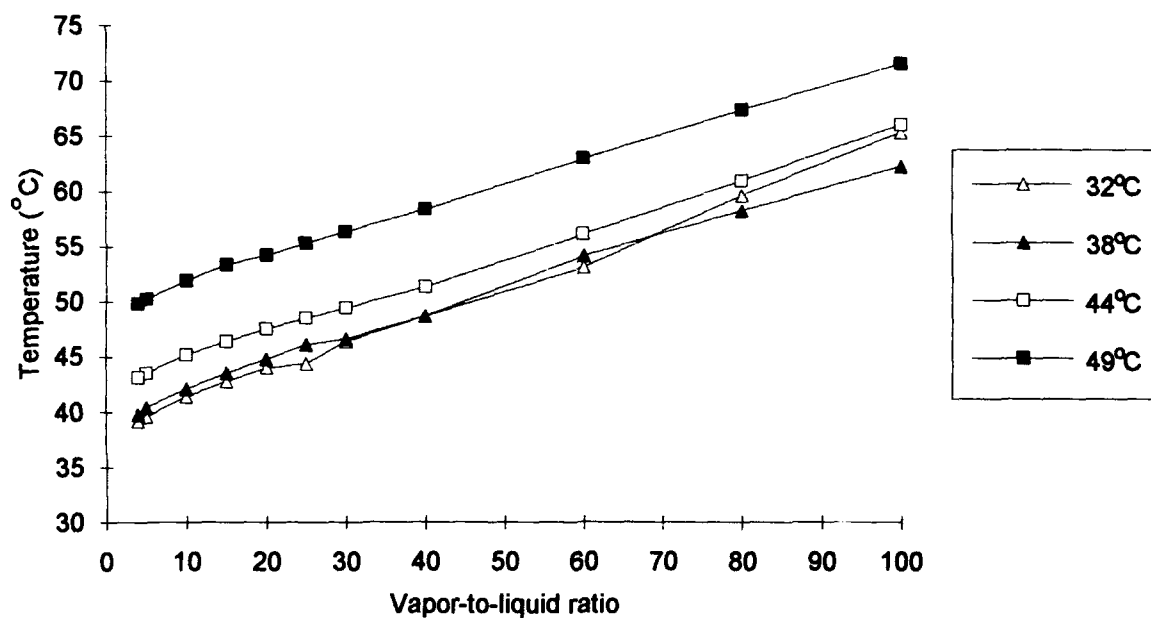
Figure 2.1.5. Vapor-to-Liquid Ratio as a Function of Tank Temperature.
