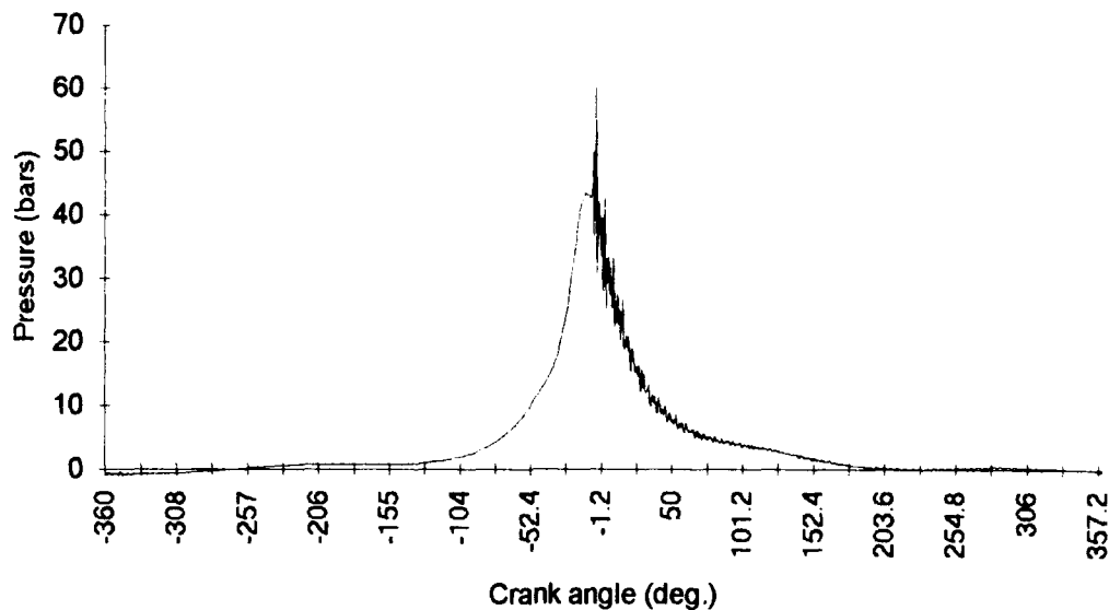
Figure 2.4.5. Pressure Trace Showing Heavy Detonation.
