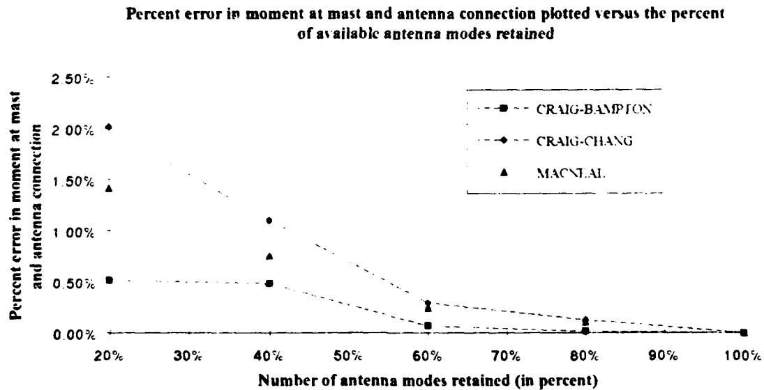
Figure 21: Percent error in moment at mast and antenna connection plotted versus the percent of available antenna modes retained. (Forcing Frequency: 47.26 Hz)
