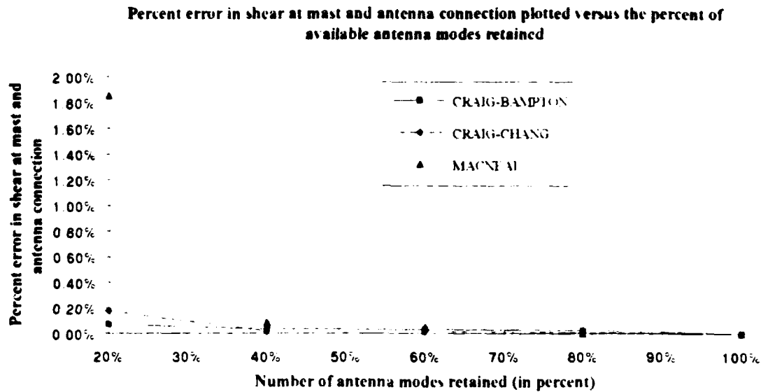
Figure 10: Percent error in shear at mast and antenna connection plotted versus the percent of available antenna modes retained. (Forcing Frequency: 8.95 Hz)
