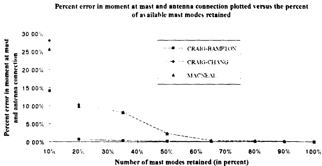
Figure 19: Percent error in moment at mast and antenna connection versus the percent of available mast modes retained. (Forcing Frequency: 47.26 Hz)
