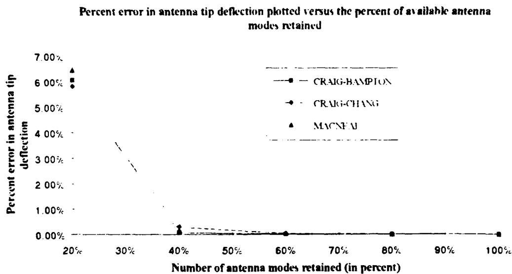
Figure 7: Percent error in antenna tip deflection plotted versus the percent of available antenna modes retained. (Forcing Frequency: 219 Hz)
