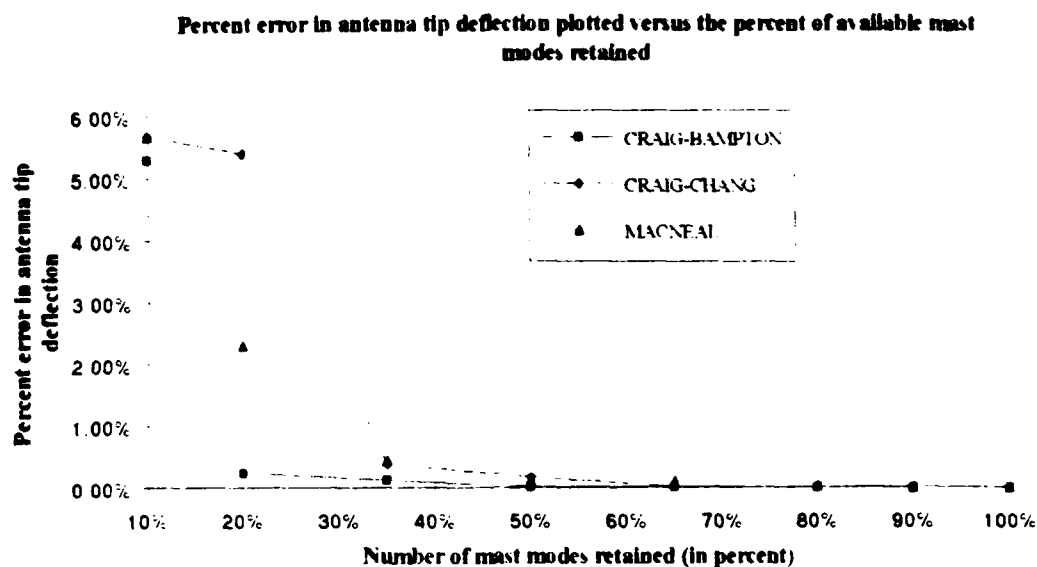
Figure 6: Percent error in antenna tip deflection plotted versus the percent of available mast modes retained. (Forcing Frequency: 219 Hz)
