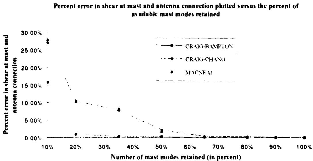
Figure 18: Percent error in shear at mast and antenna connection plotted versus the percent of available mast modes retained. (Forcing Frequency: 47.26 Hz)
