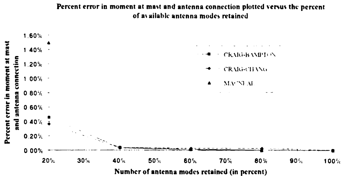
Figure 11: Percent error in moment at mast and antenna connection plotted versus the percent of available antenna modes retained. (Forcing Frequency: 8.95 Hz)
