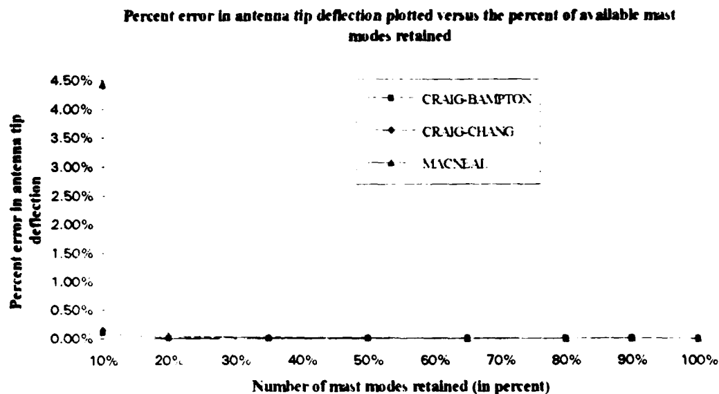
Figure 4: Percent error in antenna tip deflection plotted versus the percent of available mast modes retained. (Forcing frequency: 8.95 Hz)
