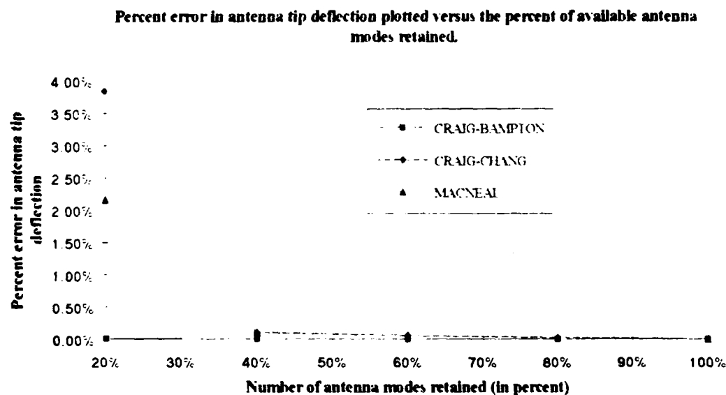
Figure 5: Percent error in antenna tip deflection plotted versus the percent of available antenna modes retained. (Forcing Frequency: 8.95 Hz)
