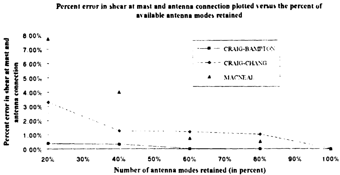
Figure 20: Percent error in shear at mast and antenna connection plotted versus the percent of available antenna modes retained. (Forcing Frequency: 47.26 Hz)
