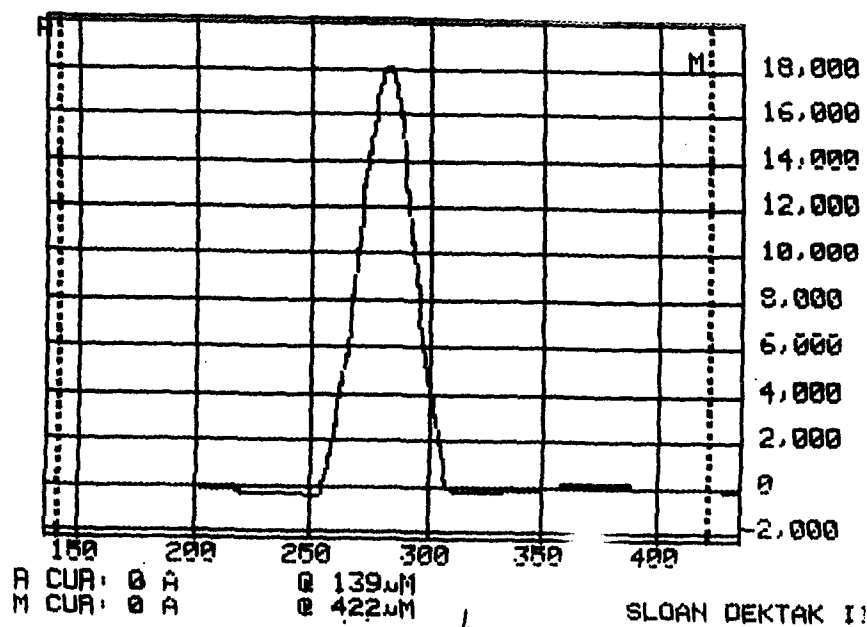
Figure 13: Dektak profile of a deposited spot using focussed LMCIS beam after a gold etch of 2000 Å. The vertical scale is in Å and horizontal scale is in microns.
