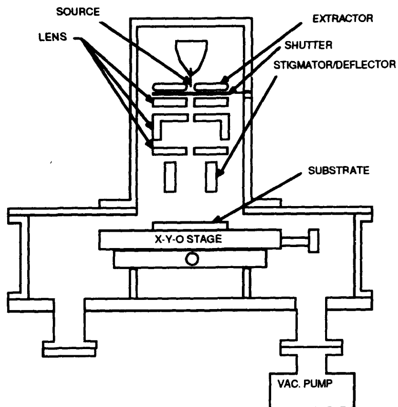
Figure 7: A schematic of LMCIS column. An asymmetric Einzel lens is used for focussing.
