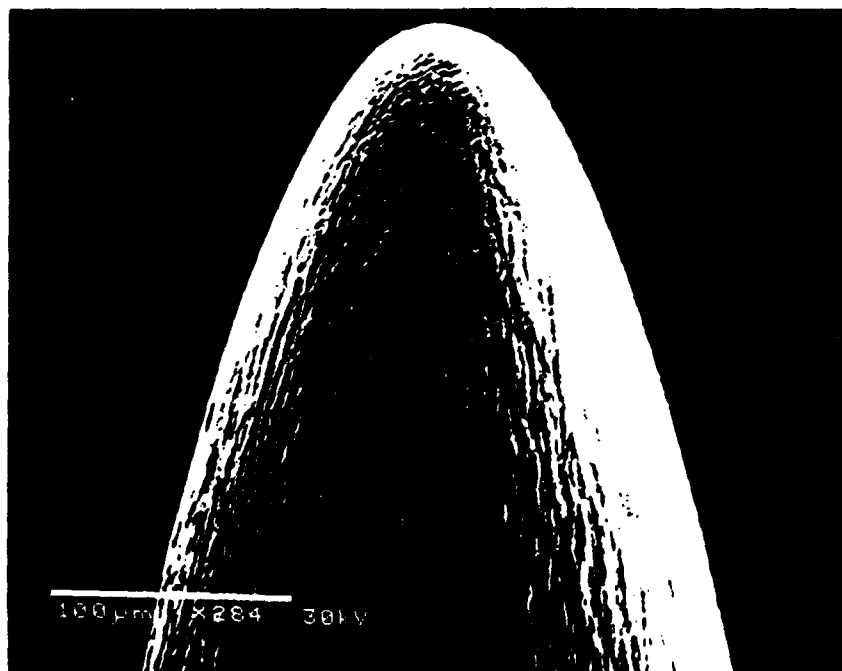
Figure 2: Tip profile of the tungsten needle of an LMCIS fabricated by electro chemical polishing. This rounded tip geometry of 40\text{ }\mu\text{m} tip radius produced desired emission properties. The surface roughness is desired for better flow of material to the tip.
