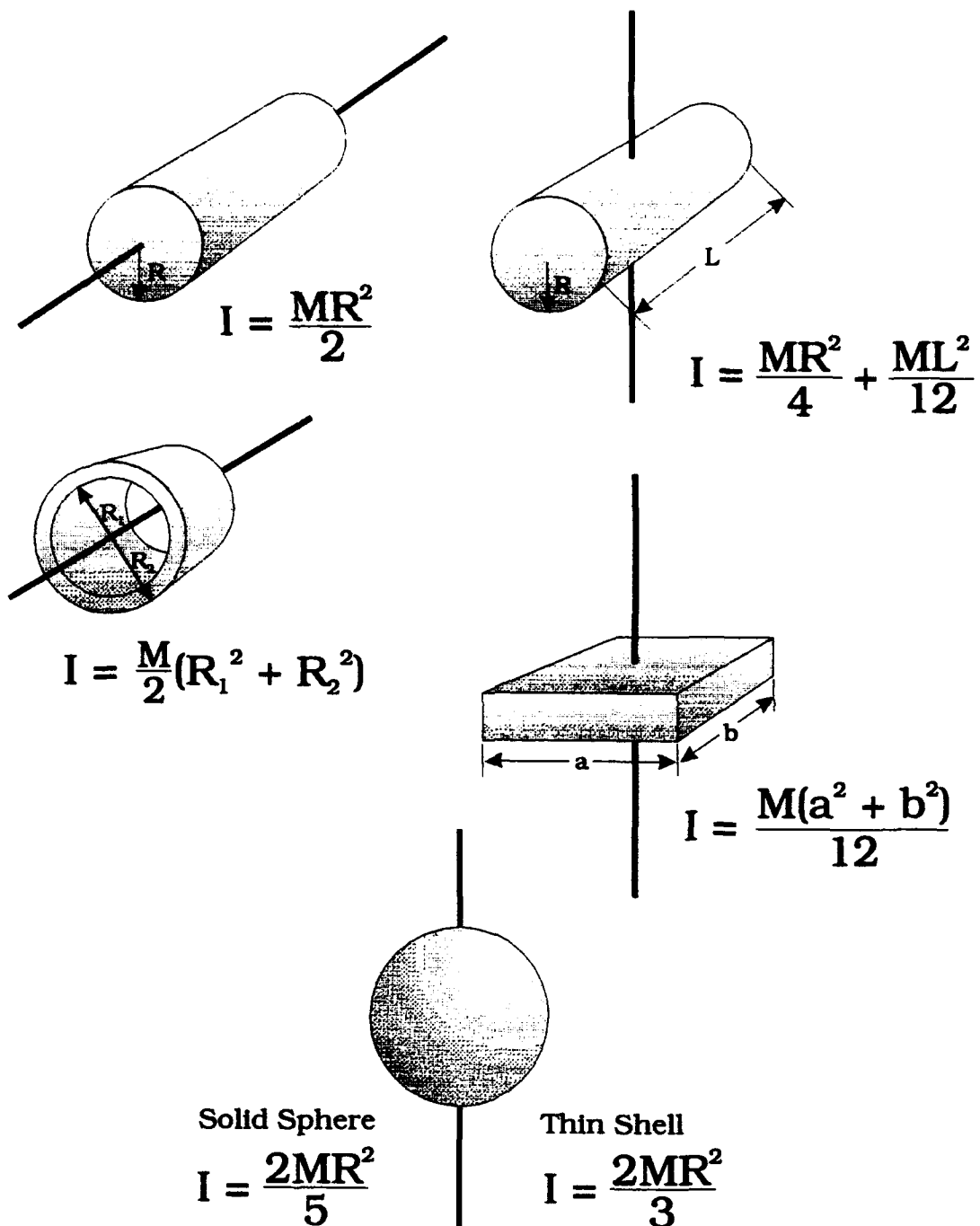
Figure 2.6 Rotational Inertia
