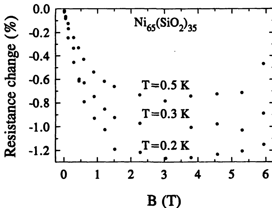
Fig. 11: Magnetoresistance of a granular Ni_{65}(SiO_2)_{35} film as a function of temperature and applied magnetic field.
