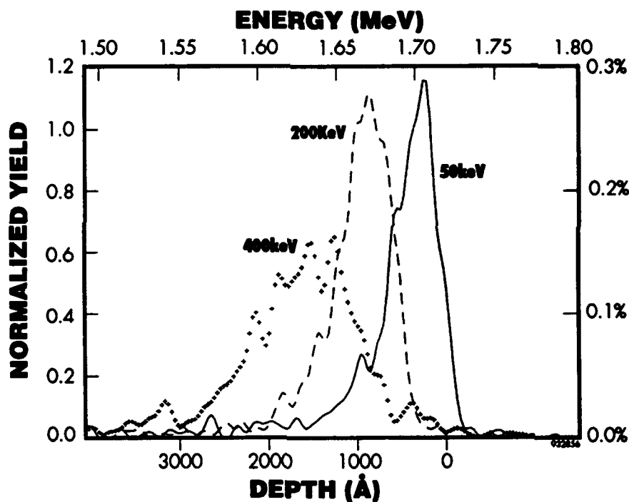
Figure 13 Concentration depth profile, as determined by RBS measurements, of Er implanted with a dose of 10^{15}/\text{cm}^2 at 50, 200, and 400 keV into porous Si.
