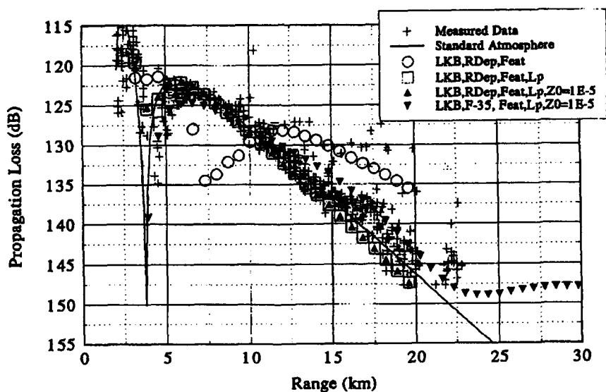
Figure 34. Comparisons of the measured (crosses) to the predicted propagation loss derived from the LKB (and variants) surface layer model for the run from 12:06 to 12:48 PST made on 5 December 1991.
