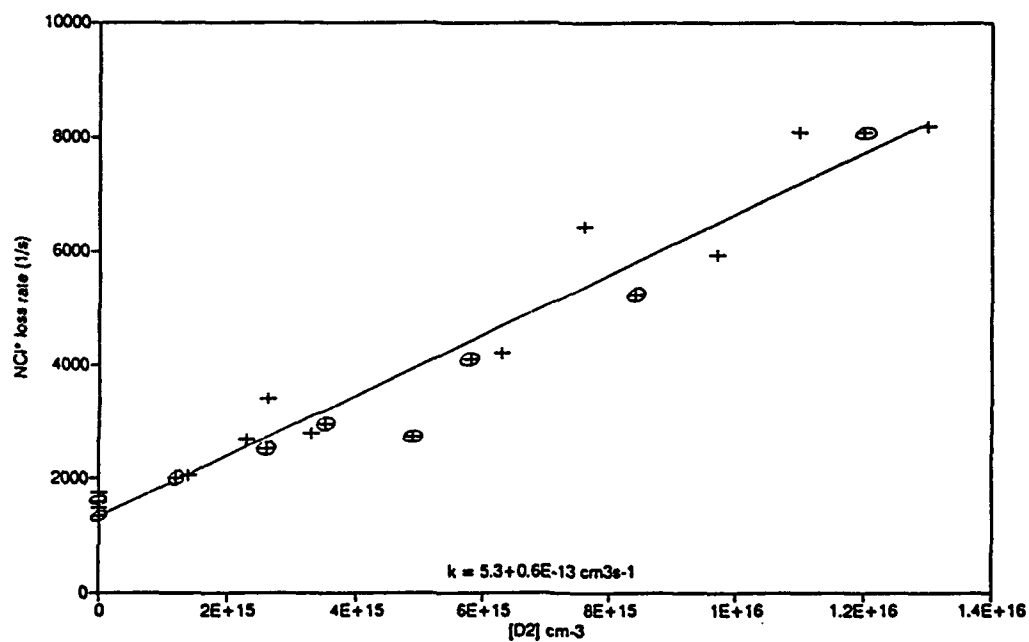
Figure 5. Plots of the exponential decay rates of \text{NCl} a \rightarrow X emission in the presence of \text{H}_2 and \text{D}_2 . Solid lines are least-squares fits to the data.
