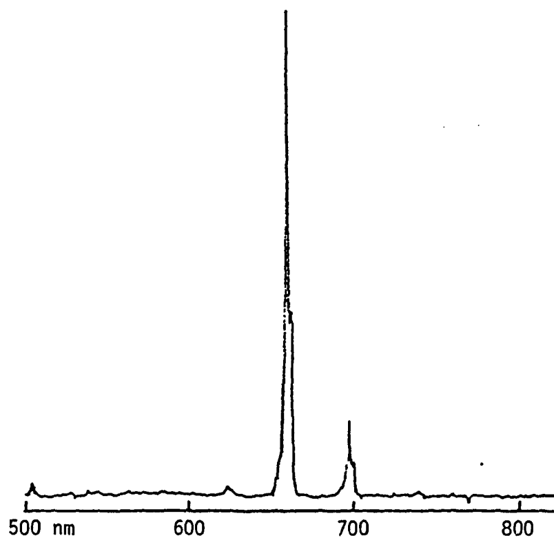
Figure 12. Spectra recorded of chemiluminescence generated in the transverse flow reactor. a) IR spectrum showing \text{NCl } a \rightarrow X emission. b) Visible spectrum showing \text{NCl } b \rightarrow X emission.
