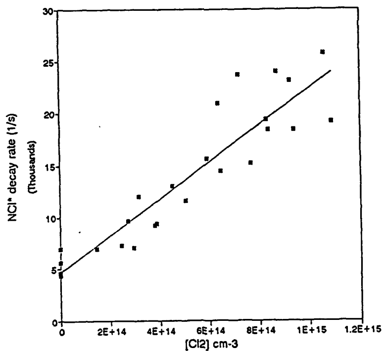
Figure 7. Plots of the exponential decay rates of NCl a \rightarrow X emission in the presence of O_2 and Cl_2 . Solid lines are least-squares fits to the data.
