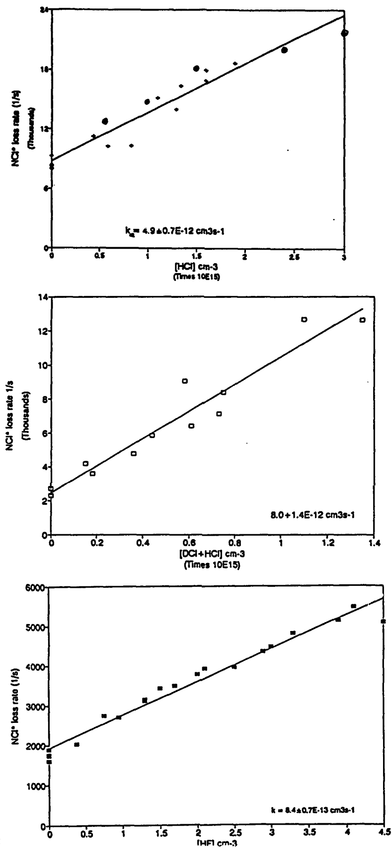
Figure 6. Plots of the exponential decay rates of NCl \alpha \rightarrow X emission in the presence of HCl, DCI, and HF. Solid lines are least-squares fits to the data.
