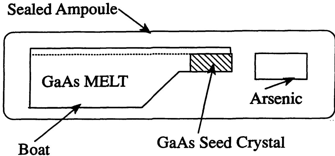
Figure 1.4: GaAs Growth by Horizontal Bridgeman Method.
