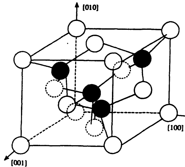
Figure 1.1: Conventional Unit Cell of GaAs.
