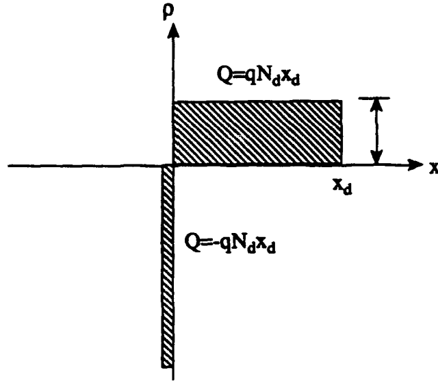
Figure 2.3: Charge Distribution in Metal Semiconductor Junction.
