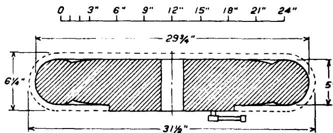
30 by 5 disk wheel and low-pressure tire. 30 by 5 disk wheel and 32 by 6 high-pressure tire. (dotted) Drag = 5.9 lb. (30 by 5) at 80 m.p.h. Drag = 6.9 lb. (32 by 6) at 80 m.p.h.
