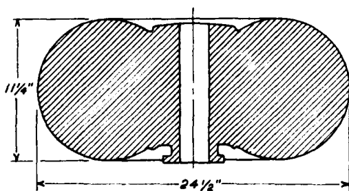
25 by 11 1/4 extra-low pressure wheel and tire. Drag = 7.1 lb. at 80 m.p.h.
