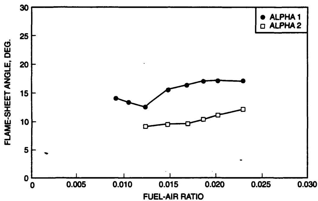
Figure 28b. Flame Angles Developed Using Convolved Splitter, B4A1, W_{pri}/W_{sec} \approx 0.76
