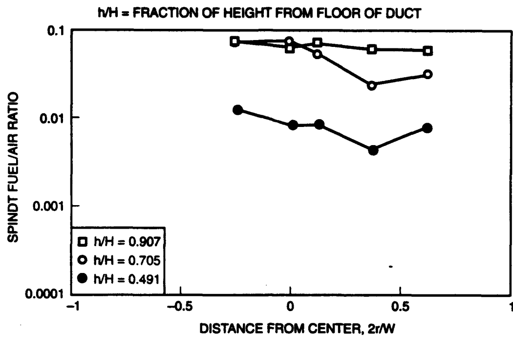
Figure 24b. Fuel/Air Ratio: Baseline 4/Alt. 1 — W_p/W_s = 0.30
