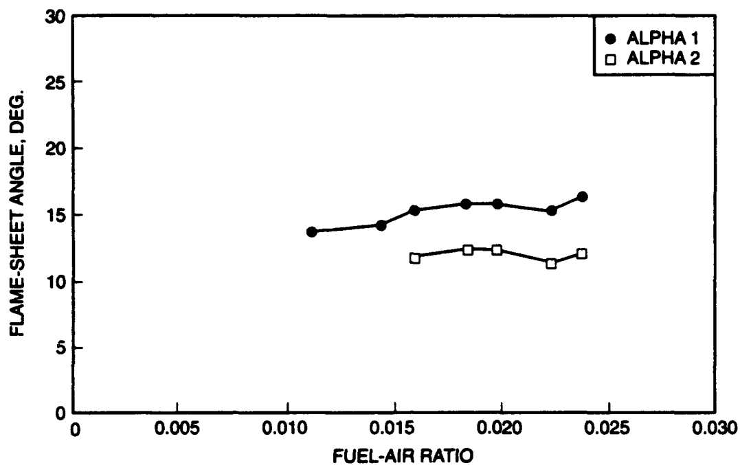
Figure 28a. Flame Angles Developed Using Convolute Splitter, B4A1, W_{prt}/W_{sec} = 0.27
