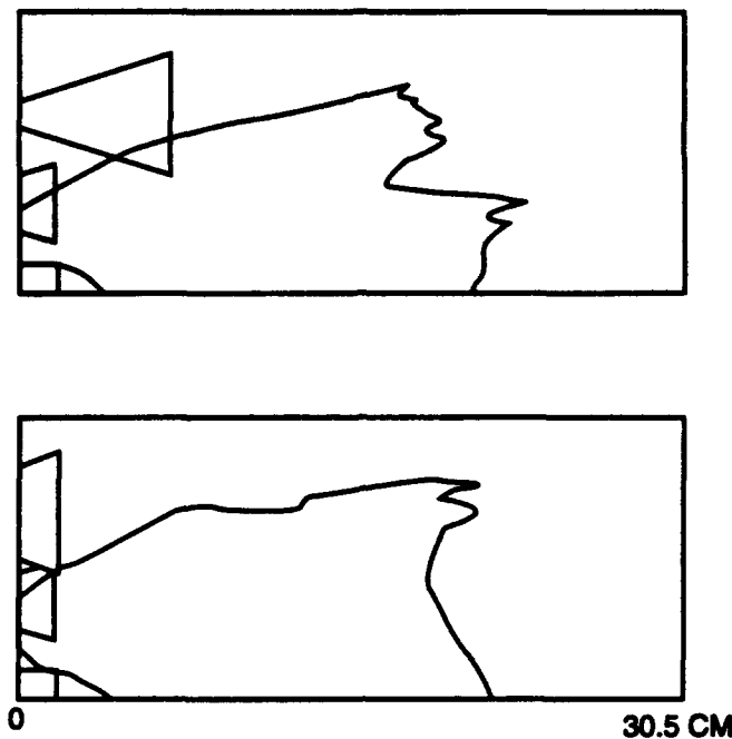
Figure C-6. Comparison of Flame Shapes Produced by Convoluted Splitters B4 (Top) and B4A1 (Bottom) — Overall F/A = 0.01 , W_{pri}/W_{sec} = 0.27
