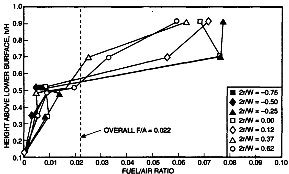
Figure 30. Vertical Fuel-Air Ratio Distribution for Convoluted Splitter, B4A1 at 27.3 cm from Step. W_{pr}/W_{sec} = 0.3
