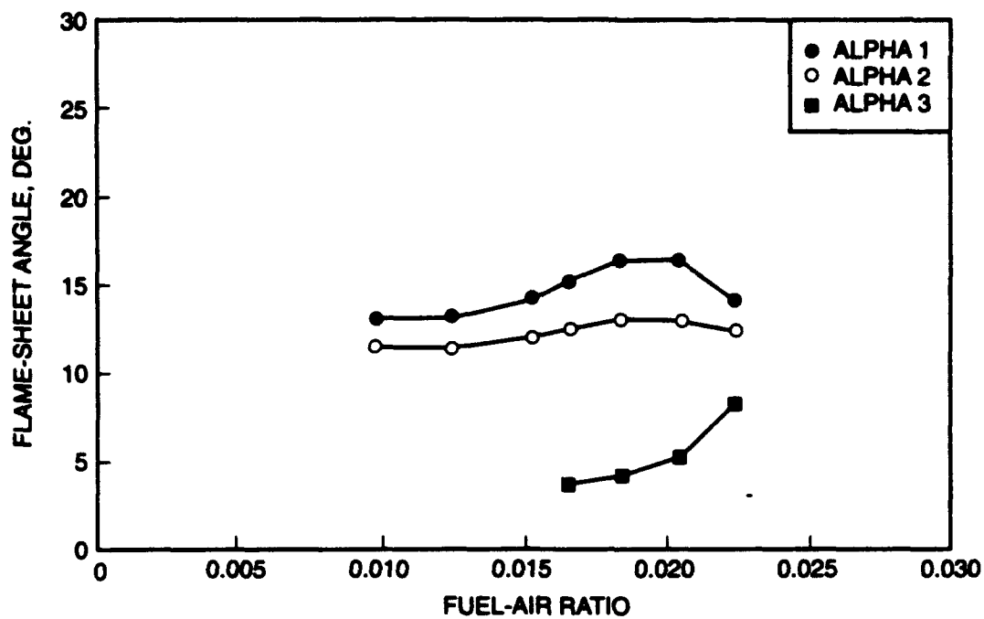
Figure 27a. Flame Angles Developed Using Convolved Splitter, B4, W_{pr}/W_{sec} = 0.26
