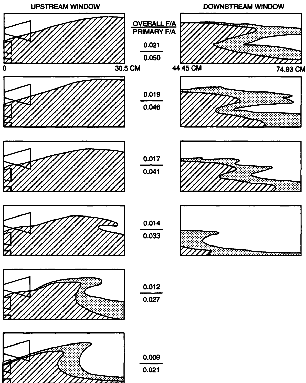
Figure C-2. Flame Shapes Produced by Convolted Splitter Baseline 4 at Indicated Fuel-Air Ratios. W_{pr}/W_{sec} = 0.73
