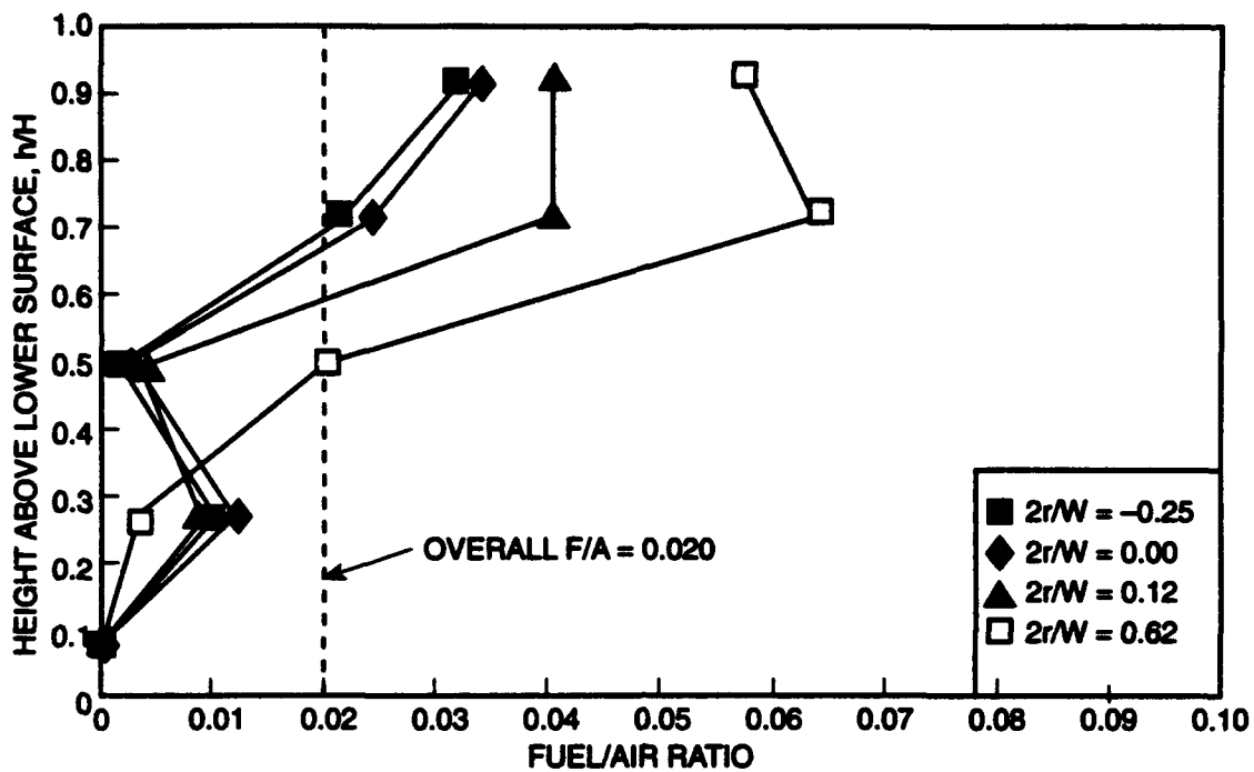
Figure 29. Vertical Fuel-Air Ratio Distribution for Convolutional Splitter, B4 at 27.3 cm from Step. W_{prt}/W_{sec} = 0.7
