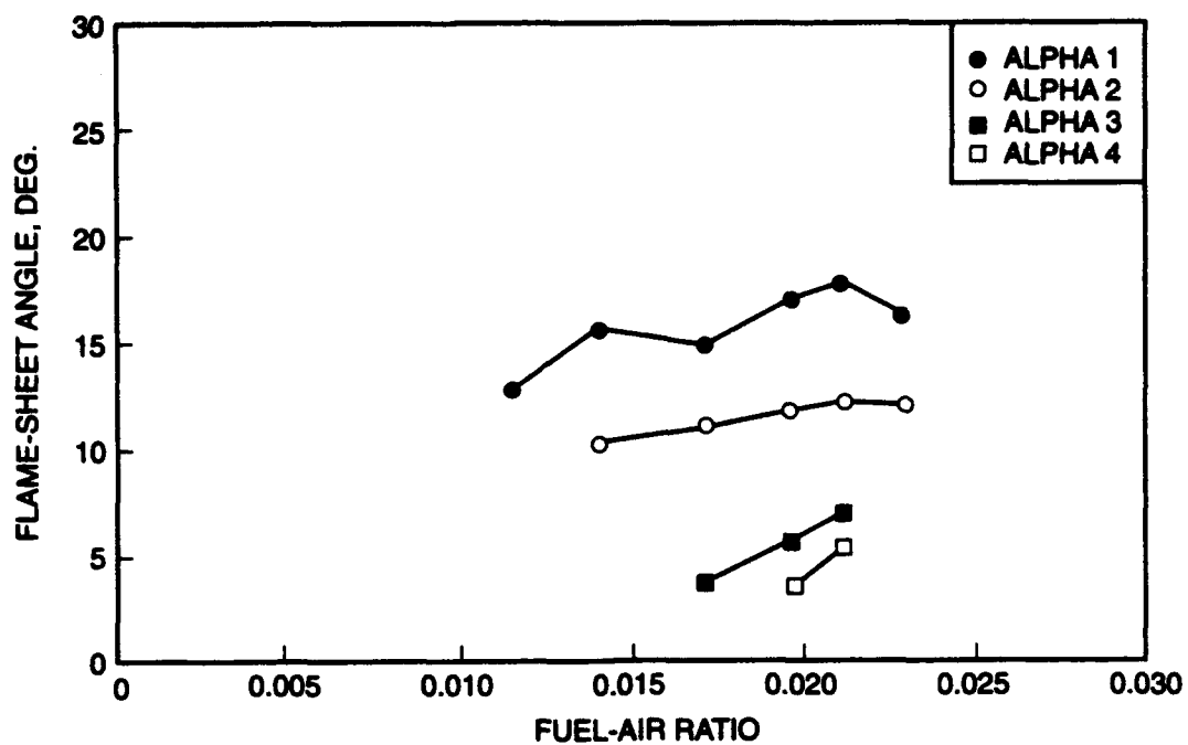
Figure 27b. Flame Angles Developed Using Convuluted Splitter, B4, W_{pri}/W_{sec} = 0.72
