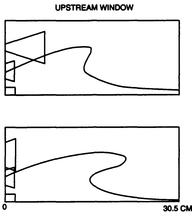
Figure C-5. Comparison of Flame Shapes Produced by Convoluted Splitters B4 (Top) and B4A1 (Bottom) — Overall F/A = 0.01 , W_{prt}/W_{sec} = 0.73
