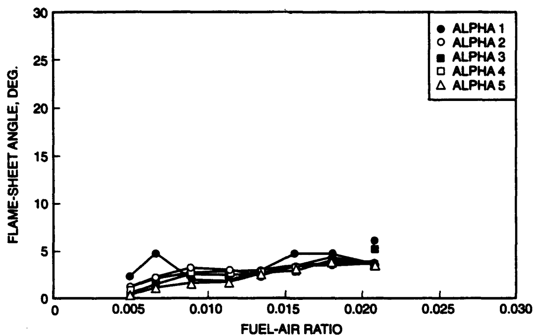
Figure 26a. Flame Angles Developed with Linear Splitter, W_{pr}/W_{sec} = 0.20
