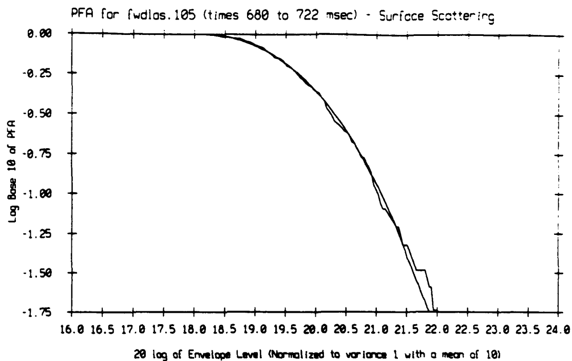
Figure 4.6: Surface Scattering Statistics fwd-las.105.
