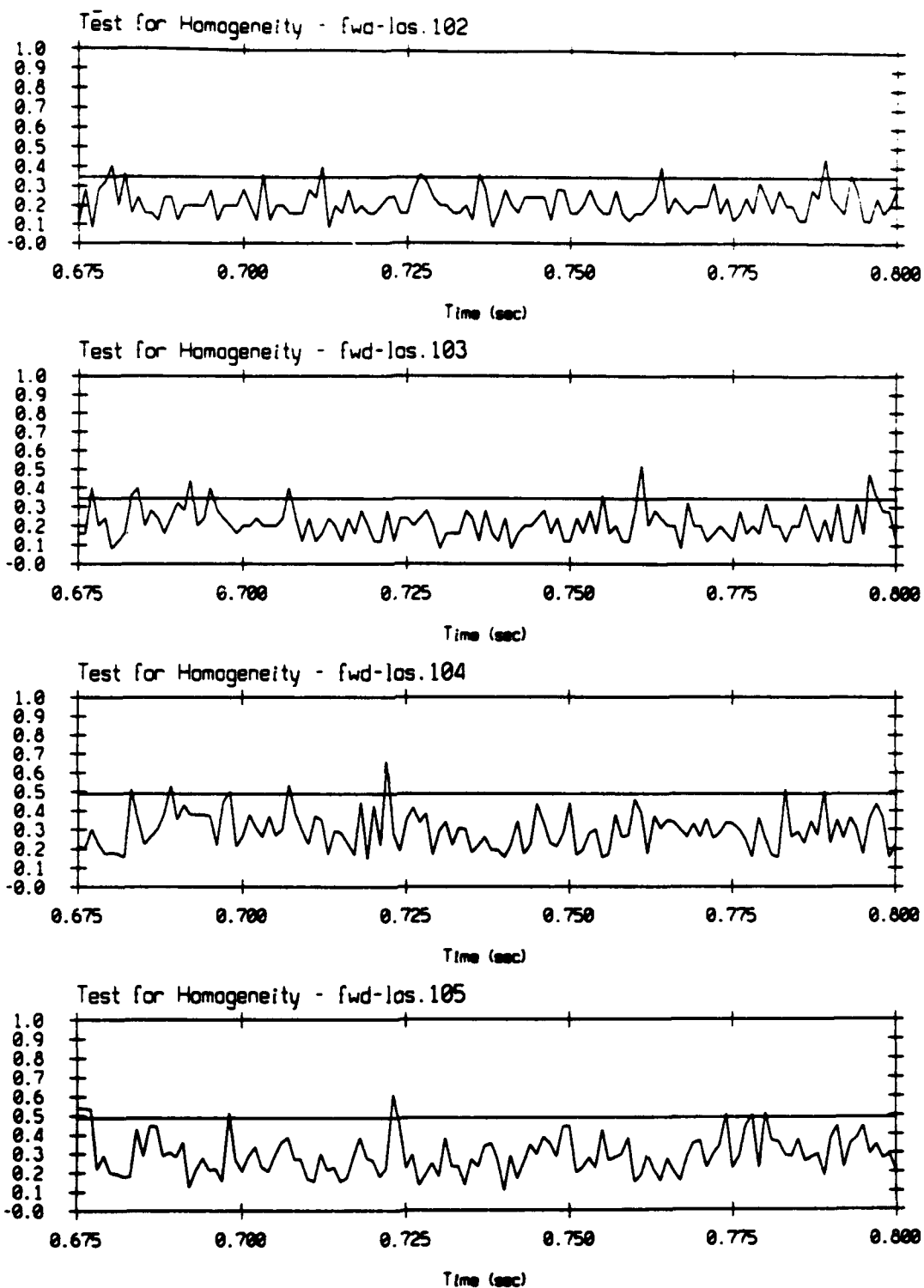
Figure 3.10: Testing for Homogeneity - fwd-las.102, 103, 104 and 105. Z_{\text{sample}} versus time (msec) is plotted. The horizontal line is Z_{\alpha} .
