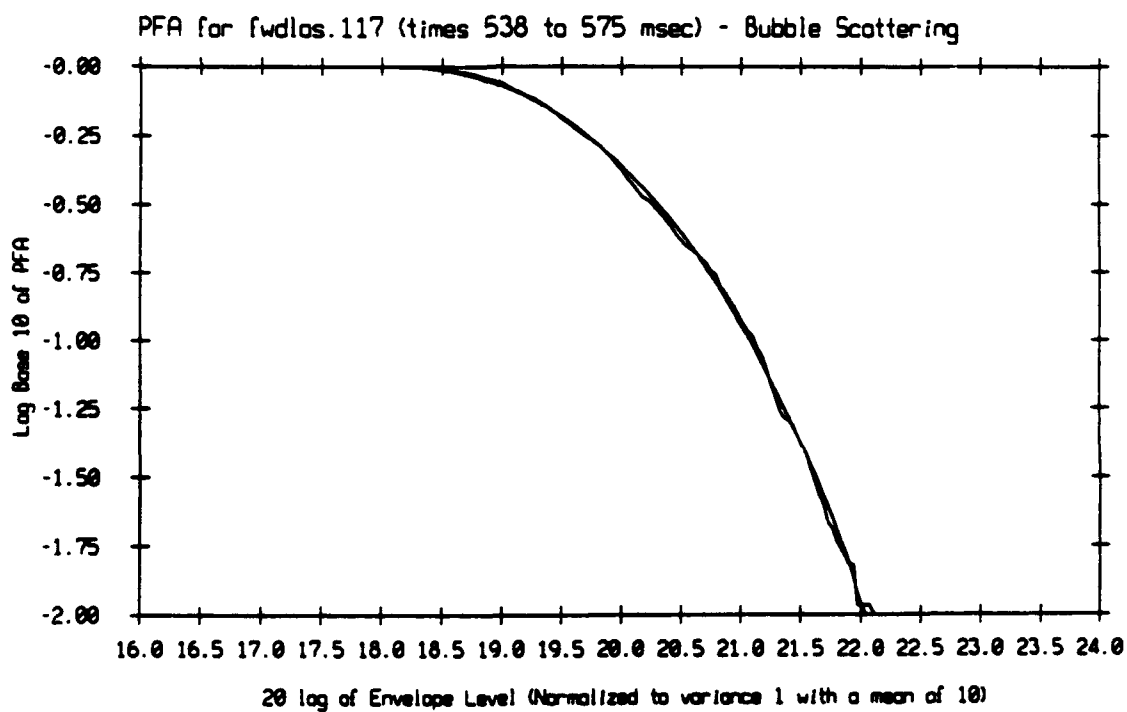
Figure 4.20: Bubble Scattering Statistics fwd-las.117.
