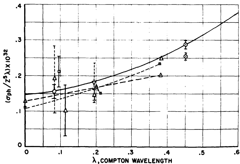
FIGURE 2. Data analysis and interpolation for the photoelectric cross section of Pb at energies > 1 Mev.
