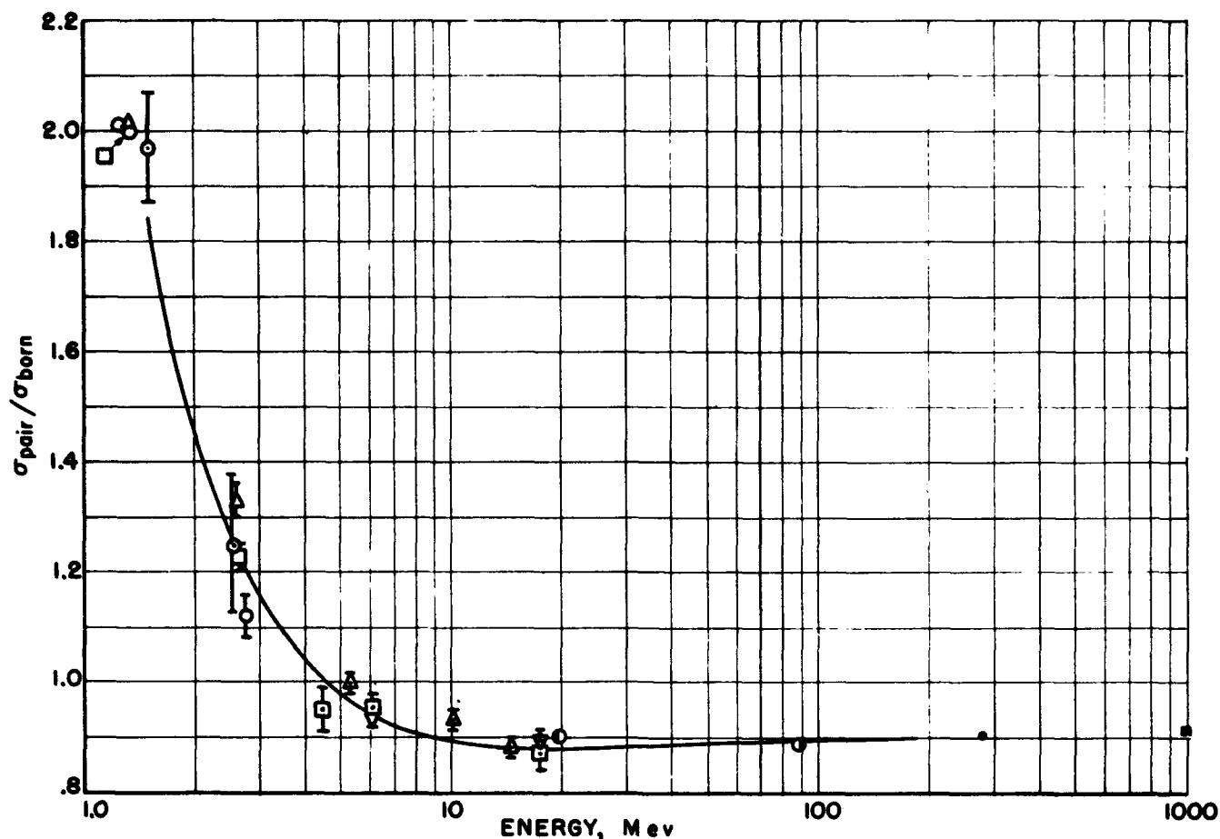
FIGURE 4. The ratio \sigma_{pair}/\sigma_{Born} for lead.
