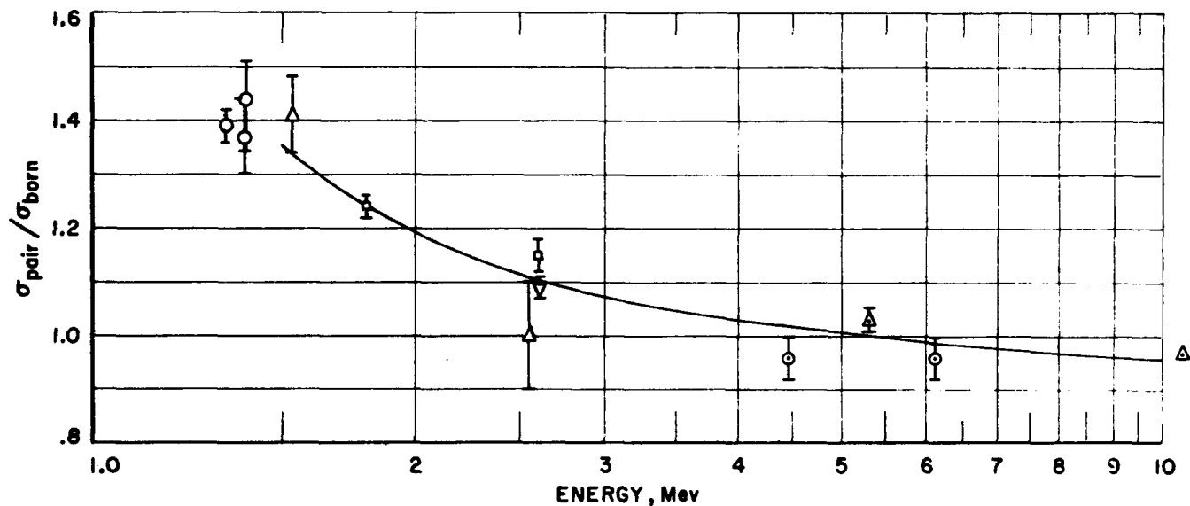
FIGURE 5. The ratio \sigma_{pair}/\sigma_{Born} for iodine.
