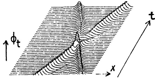
Fig. 2. Fluxon-antifluxon collision. \alpha = 0.2 , \eta = 0.22 , l = 40 .
