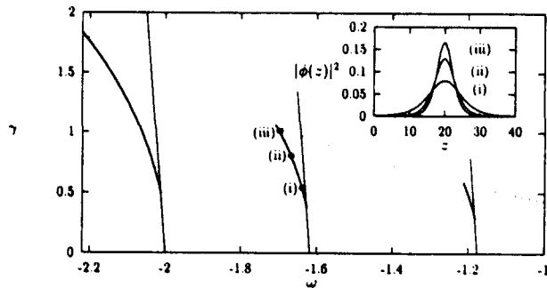
Fig. 4. Paths of travelling waves in the discrete NLS equation (2.4) for L = 40 and, from the left, (a) c = 0.01 , (b) c = 1.2 , (c) c = 1.6 . Localized ("solitary") waves bifurcate from stationary solutions (straight lines), but only seem to exist when \gamma is sufficiently small as indicated by the dotted line. The inset shows waveforms along the c = 1.2 path.
