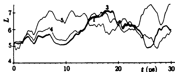
Fig. 3. Time dependence of the soliton width L(v=0) in the thermalized chain with \chi_1 = 1 \times 10^{-10} N and \chi_2 = 1 \times 10^{-12} at t_c = 0.1; 0.07; 0.04; 0.01; 0.001 ps (curves 1, 2, 3, 4, 5, respectively).
