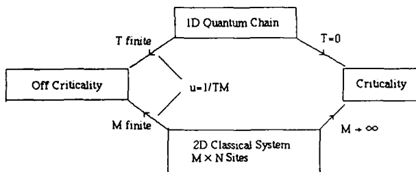
Fig. 1. Relations between finite size system and finite temperature system.
