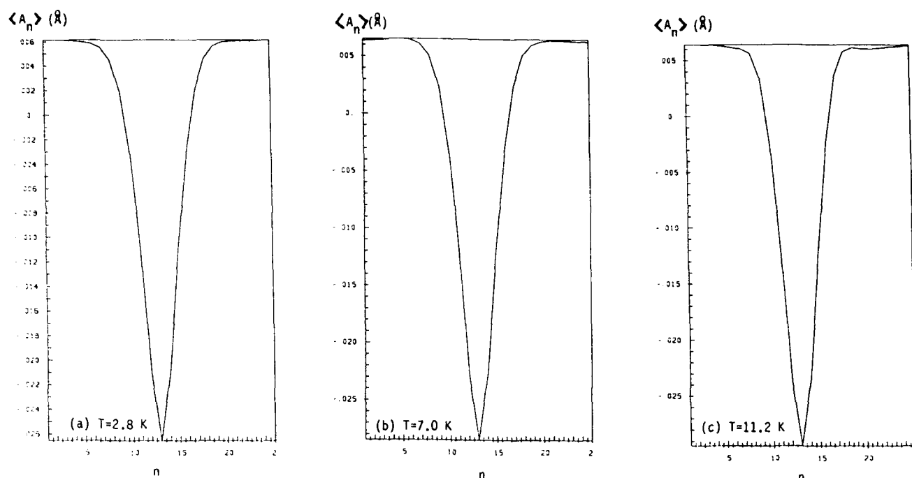
Fig. 3. Time average \langle A_n \rangle over 3 000 000 time steps (6 ns) of the lattice displacements A_n in the rotated coordinate system for the system of fig. 2 at the same temperatures.
