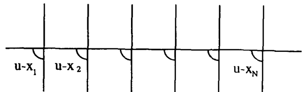
Fig. 2. Inhomogeneous lattice.
