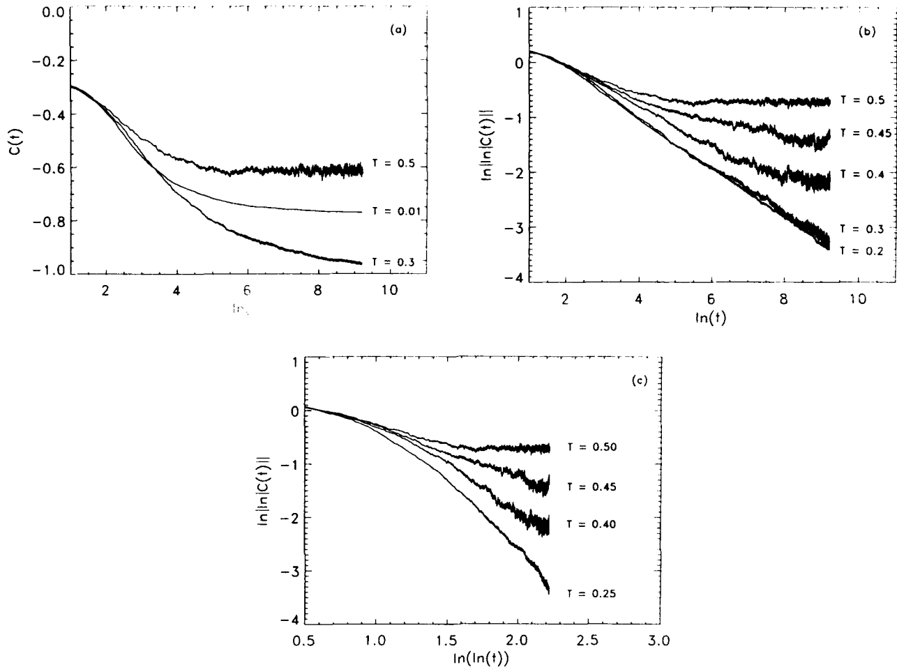
Fig. 2. The global correlation function C(t) during relaxation from random initial condition for f = \frac{1}{2} and zero disorder, \delta x_{ij} = \delta y_{ij} = 0 .
