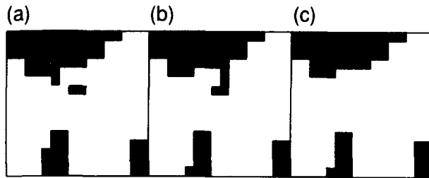
Fig. 4. Annihilation of a thermally nucleated ( T = 0.25 ) vortex-antivortex pair on a domain boundary. The plots show 16 \times 16 of the total 128 \times 128 system for three different times ( t_a < t_b < t_c , t_a - t_c \approx 2 ). The \tilde{q}_{ij} configuration is shown as in fig. 2 (left).
