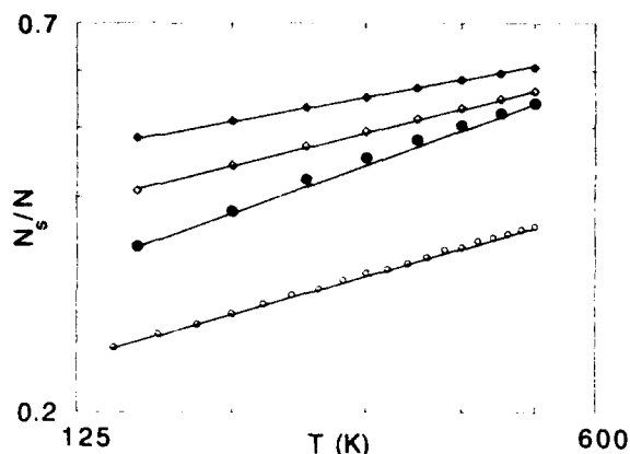
Fig. 1. Number of solitons, N_s , versus temperature, T , in logarithmic scale, for N = 64 masses. Circle: single strand model [6,1]. Bullet: homogeneous double strand model ( \epsilon = 0.022 eV, k = 15.8 N/m, \sigma = 2.7 \times 10^{-10} m). Diamond: inhomogeneous double strand model for parameter values of case (a) (empty diamond) and case (b) (full diamond).
