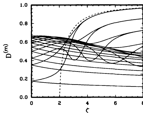
Fig. 4. Solid lines: the localization measure D^{(m)} vs. \zeta for the 21 stationary quantum states at the quantum level n = 20 , J = 1 , \omega_0 = 0 . Dashed line: ||a_1| - |a_2|| for classical local mode stationary solutions.
