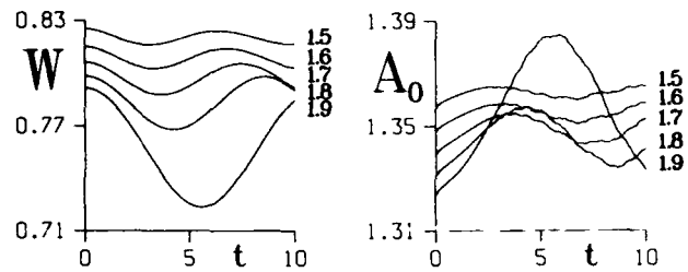
Fig. 2. Width, W , and center amplitude, A_0 , as function of time for f = 257 and L = 25.6 . \sigma = 1.5, 1.6, 1.7, 1.8, 1.9 .
