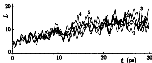
Fig. 4. Time dependence of the localization width L for the static self-trapping state in the thermalized chain with \chi_1 = 1 \times 10^{-10} N and \chi_2 = 4 \times 10^{-11} N at t_c = 0.1; 0.07; 0.04; 0.1; 0.001 ps (curves 1, 2, 3, 4, 5, respectively).
