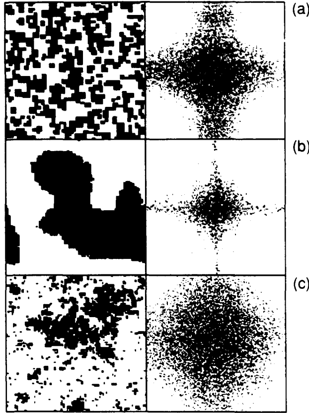
Fig. 3. The \tilde{q}_{ij} configuration (left) for the relaxed states ( t = 10^4 ) at different temperatures and the spectral power (right) |g(k)| . \tilde{q}_{ij} > 0 - black; \tilde{q}_{ij} < 0 - white. The color code for the spectral power is \log_{10}(|g(k)|^2) > 10^3 - black; 10^5 < \log_{10}(|g(k)|^2) < 10^3 - grey; \log_{10}(|g(k)|^2) < 10^5 - white. (a) T = 0.01 ; (b) T = 0.25 ; (c) T = 0.45 .
