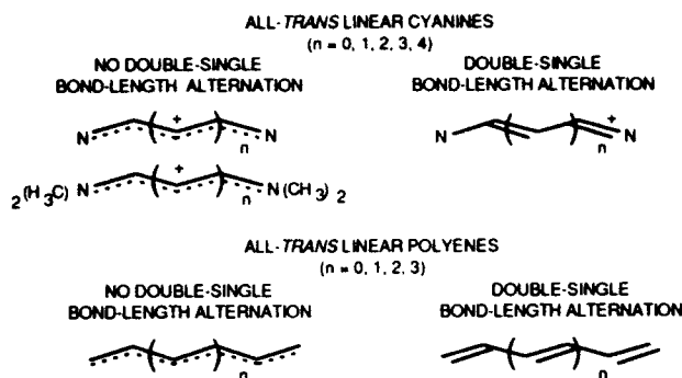
Fig. 1. Structures of the linear cyanines and polyenes with and without bond-length alternation.
