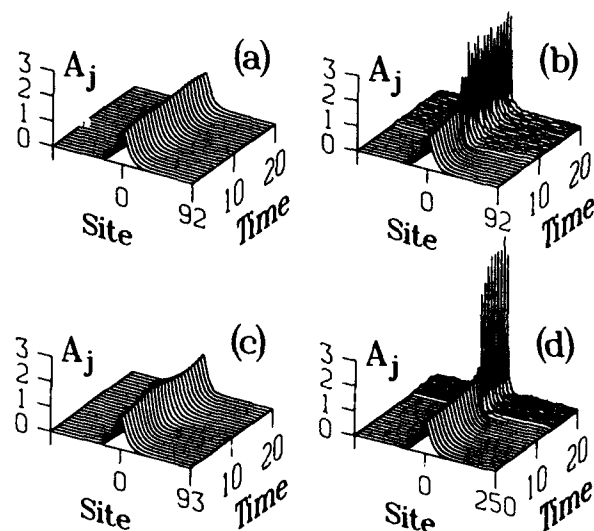
Fig. 1. Amplitude of the solution to eq. (1) and (7) with L = 25.6 . (a) \sigma = 1.90 , f = 185 , (b) \sigma = 1.95 , f = 1.85 , (c) \sigma = 1.95 , f = 191 , (d) \sigma = 2.00 , f = 501 .
