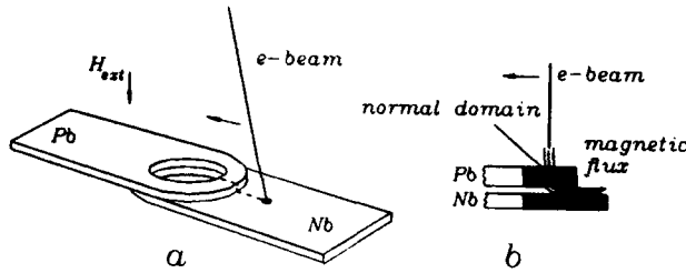
Fig. 1. (a) The magnetic flux trapping procedure in an annular junction using LTSEM. (b) The cross-section of the junction along the dashed line shown in (a) at the moment of crossing by the electron beam (the insulating SiO window is not shown).
