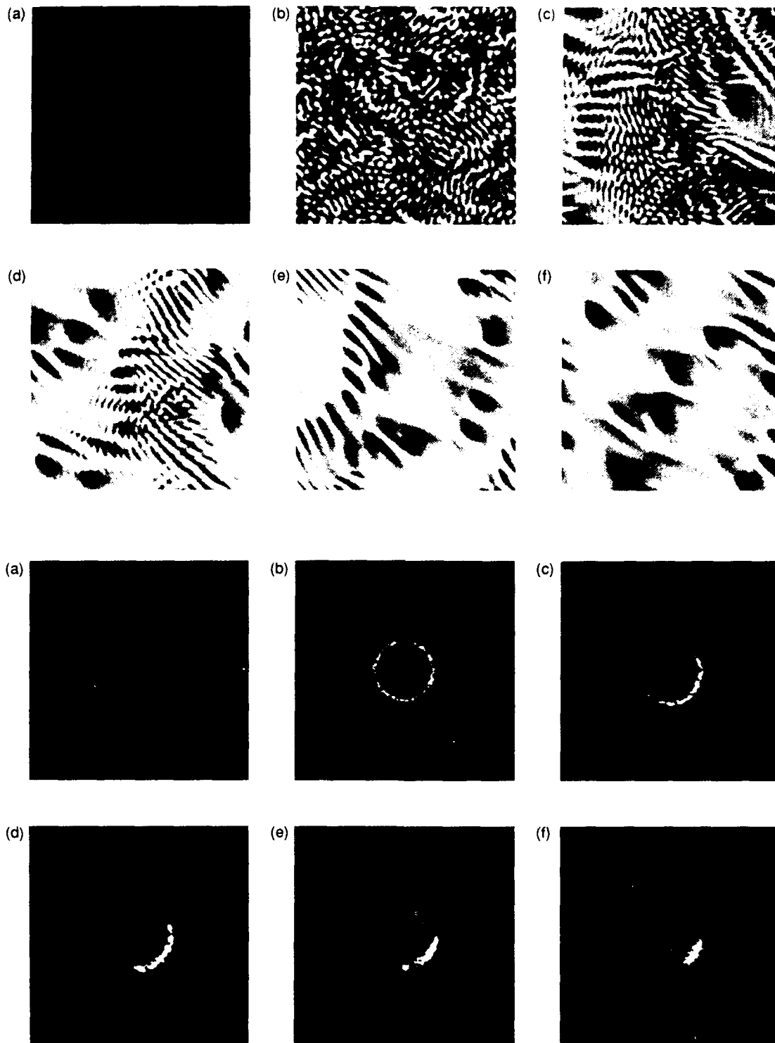
Fig. 5. (A) Frames from a movie showing a succession of transverse pattern evolutions from noise in the near-field. (B) Far-field emission corresponding to each near-field frame in (A).
