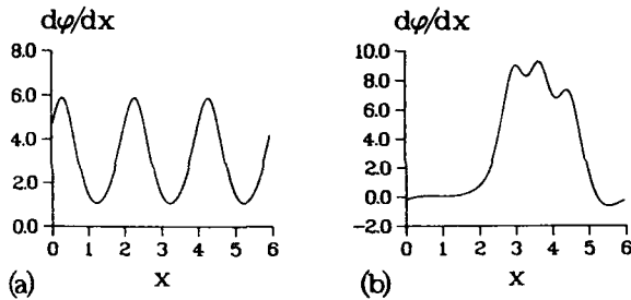
Fig. 2. The spatial distribution of the normalized magnetic field in the junction on step 3 at \gamma = 0.26 (a) and at \gamma = 0.34 (b).
