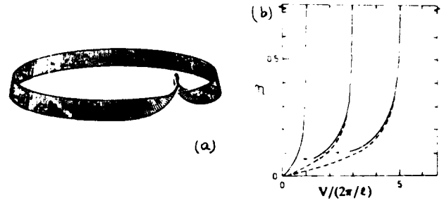
Fig. 3. (a) Equivalent pendulum array for the annular Josephson with one fluxon (from ref. [9]). (b) Schematic IV curves: Annular junction p = 1 .
