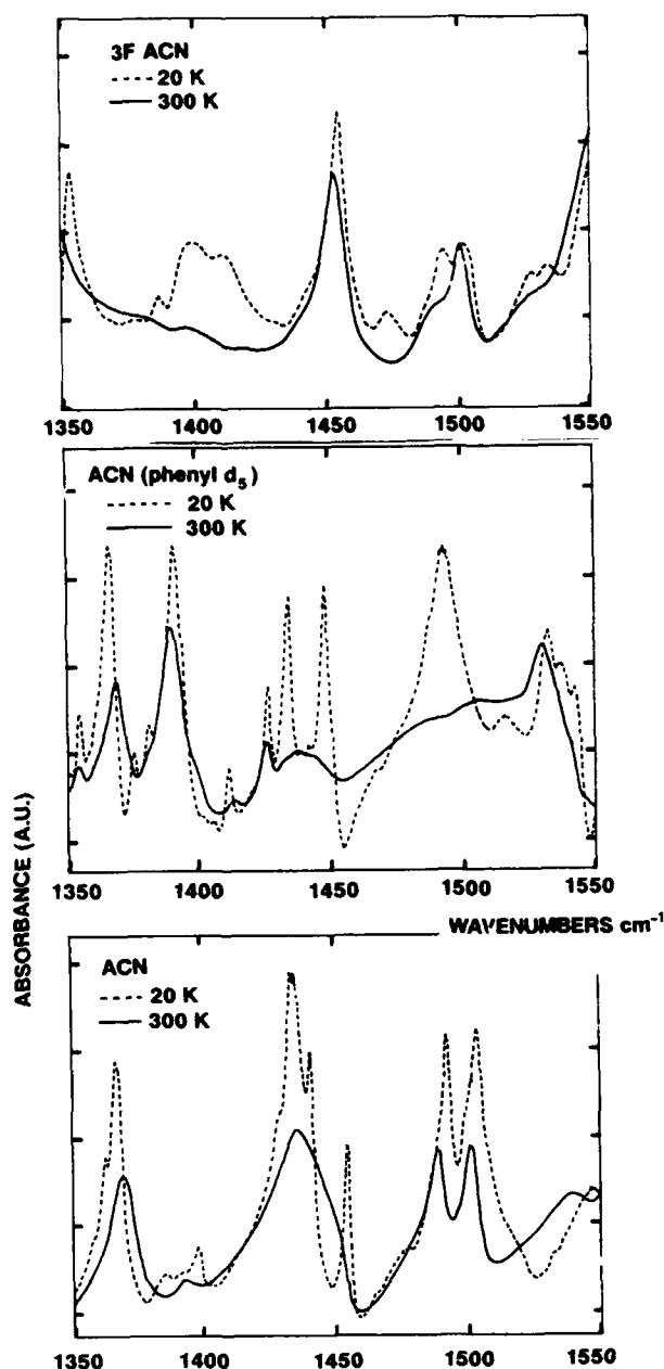
Fig. 3. Anomalous increases of intensities at 20 K in ACN, in D5 and in 3F.
