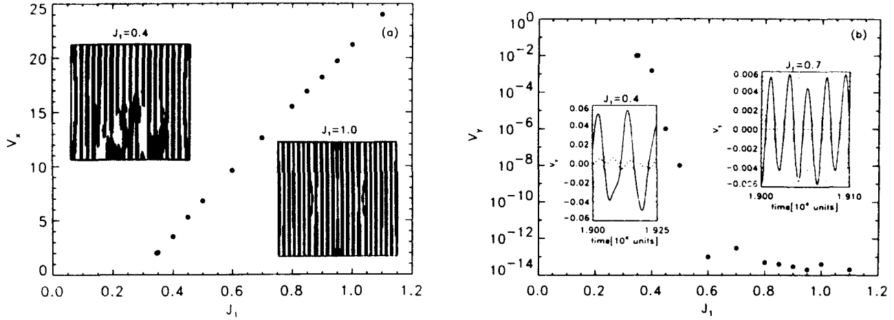
Fig. 5. The voltages across the JJA as a function of the applied bias current. (a) The longitudinal dc voltage. The insets show the \tilde{q}_{ij} configuration (color code as in fig. 2) for two characteristically different cases. The bias current is forced through the system along the horizontal axis. (b) The amplitude of the transversal voltage. Insets: time evolution of the transversal voltages, V_y (dashed), V_y^l (solid), and V_y^r (dotted).
