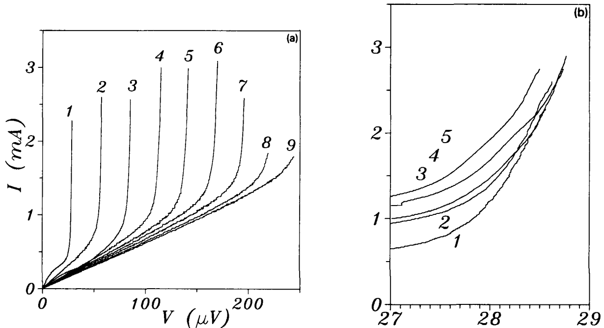
Fig. 2. (a) The I - V curves corresponding to the sequential trapping of solitons in the homogeneous annular Josephson junction using the LTSEM method. The numbers correspond to the number of solitons trapped. (b) The detailed comparison of the high-current parts of the scaled soliton steps in a magnified voltage scale (the voltage of the n th step is divided by n ).
