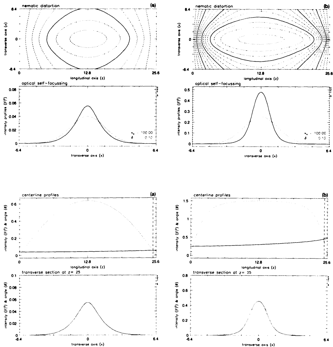
Fig. 4. Sample numerical experiments for the scalar model problem, for \alpha = 0.10, k = 100.00 . At these parameter values the critical field for the Frederiks transition has |F_{\text{cr}}|^2 \simeq (0.12)^2 . (a) Pump beam: |F_{\max}|^2 = (0.2)^2 ; (b) Pump beam: |F_{\max}|^2 = (0.5)^2 . In each case, we display contour lines for the nematic angle \theta ; the electric field intensity profiles |F|^2 vs x , at the front (dotted curve) and rear (solid curve) faces; the behavior of the electric field intensity (solid) and of the nematic (dotted) along the center beam line; and a transverse profile near the rear face for the electric field intensity (solid) and nematic angle (dotted).
