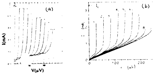
Fig. 4. (a) Experimental zero field steps for an overlap junction. (After ref. [5]). (b) Experimental n -fluxon zero field steps on an annular junction. n = 1-9 (after refs. [11,12]).
