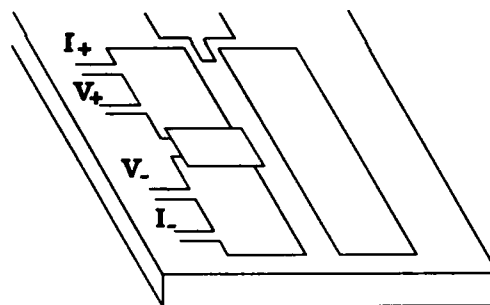
Fig. 1. Schematic drawing of the sample geometry. The coplanar resonator has its electromagnetic field confined in the gap between the two closely spaced Nb-strips. The two Josephson junctions are formed where the top and bottom films of the left strip overlap. The microstrip antenna shown at the top of the figure is used for the microwave measurements.
