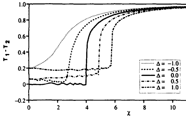
Fig. 1. Nonlinear two-waveguide with phase mismatch: space-averaged transmittance difference T_1 - T_2 = \langle |c_1|^2 \rangle - \langle |c_2|^2 \rangle versus power ( \chi ) for several phase mismatch values ( \Delta ) ( V \equiv 1 ).
