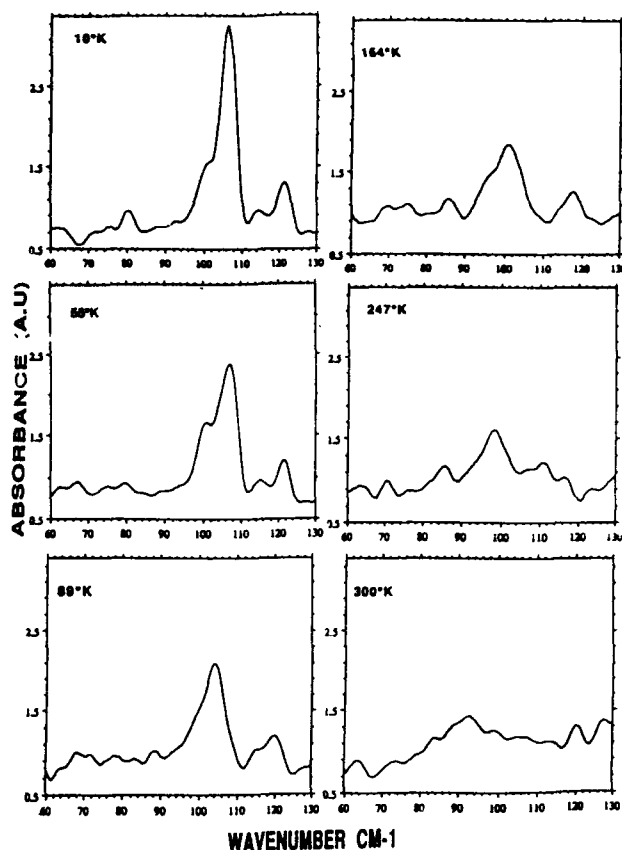
Fig. 4. Evolution of the intensity of the "H-bond strain" in ACN with respect to the temperature.
