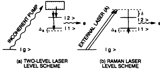
Fig. 1. Energy level diagrams depicting pumping schemes for a (a) two-level and (b) Raman laser.
