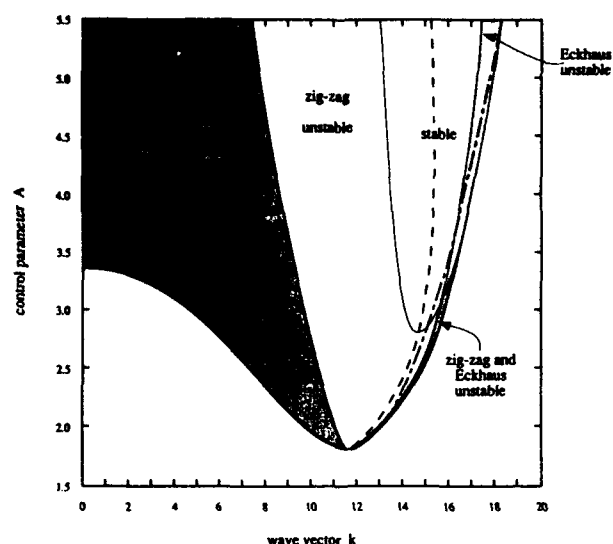
Fig. 3. Existence domain for travelling wave solutions and their associated stability properties for a Raman laser with \Omega > 0 .
