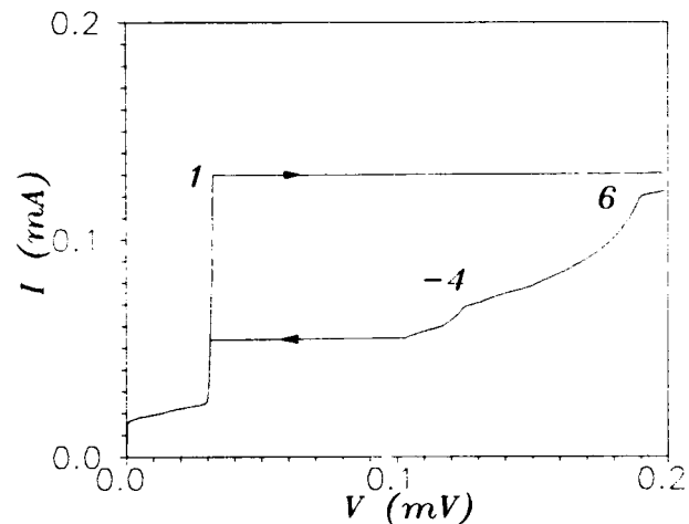
Fig. 3. The I - V curve of the junction with N = 5 inhomogeneities and n = 6 trapped solitons using the MMF method.
