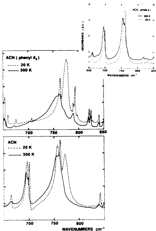
Fig. 2. Amide-V modes (or NH out-of-plane bend) in ACN and D5, showing an increase of the intensity at 20 K. The structure at about 760\text{ cm}^{-1} in the ND compound is assigned to the C-H out-of-plane bends in the aromatic ring.
