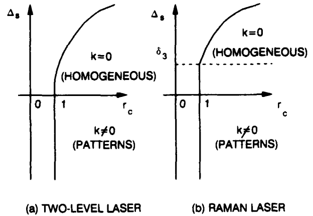
Fig. 2. Stability and instability regions for the nonlasing solution in (\Delta_s, r_c) parameter space. (a) Two-level and (b) Raman laser.
