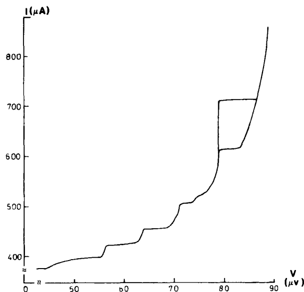
Fig. 2. Lower part of the ZFS1 for a four-junction sample (U1-4JJ). T = 4.2 K, B = 0 .
