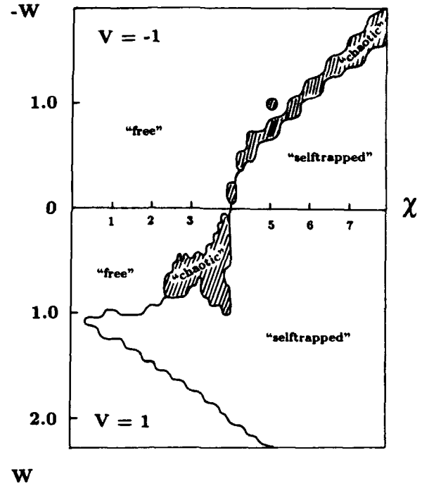
Fig. 2. Dynamical phases for the DNT system as a function of the linear coupling W and power \chi . The regimes labeled "free", "chaotic" and "self-trapped", refer to complete, chaotic and incomplete power transfer, respectively. The top half of the figure displays the case for V and W negative while the lower half is for V and W positive [7].
