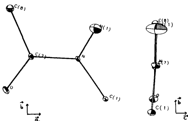
Fig. 5. ORTEP drawings of the amide group in the ACN molecule at 15 K, in the ( a , b ) molecular plane, and perpendicular. Note the large anisotropy of the H(1) ellipsoid in the c direction.
