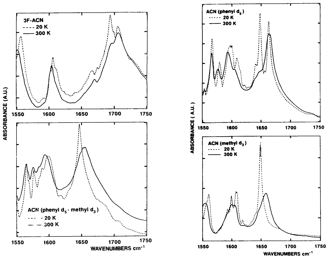
Fig. 1. Amide-I modes in four derivatives of ACN: the D5 and 3F compounds exhibit an anomalous mode like pure ACN, with a very small energy shift in the range 300–20 K. On the contrary, the D3 and D8 compounds display a classical behaviour without anomaly.
