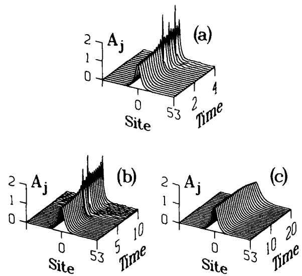
Fig. 5. Amplitude of the solution to eq. (1) with f = 107 , \sigma = 2 and L = 25.6 . The amplitude of the initial condition, given by eq. (7), is reduced by a factor (a) 1.000, (b) 0.994, (c) 0.993.
