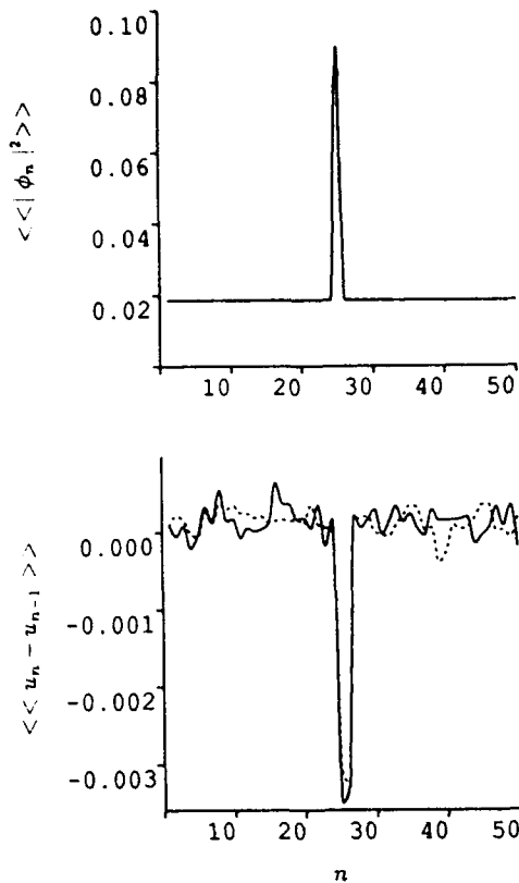
Fig. 2. Plot of the thermally averaged probability (upper) and displacement differences (lower) determined from the MC simulations (solid line) and the LD (broken line). N=50 , J = 1.549 \times 10^{-22} J, \kappa = 13 N/m, \chi = 62 pN.
