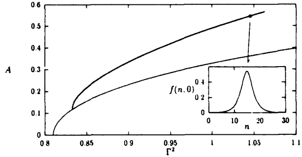
Fig. 3. Discrete sine-Gordon breather bifurcating from the simple solution (2.3) for L = 30 and \omega = 0.9 . A = \max f(n, t) .
