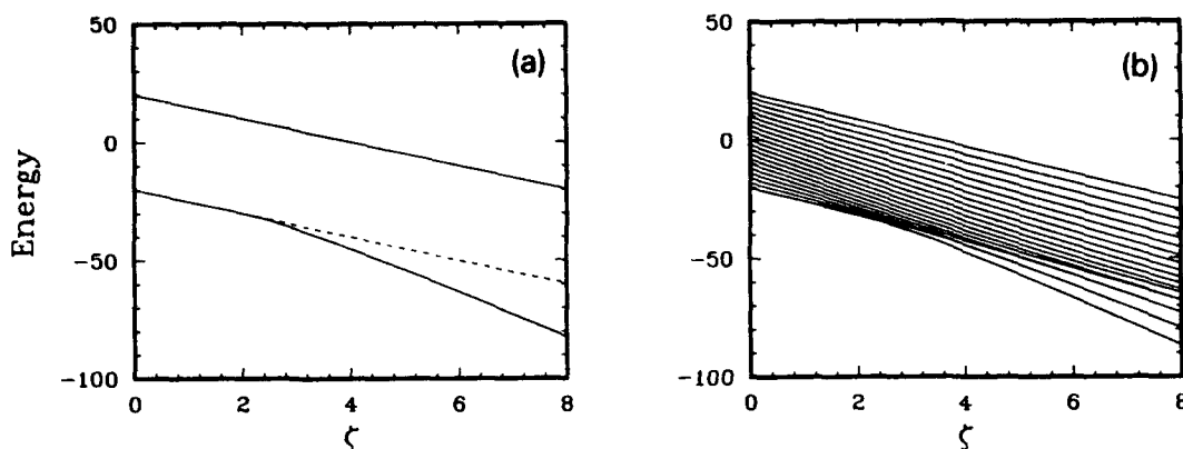
Fig. 1. Quantum and classical transitions. (a) The energies of stationary solutions of eq. (1) vs. \zeta for N = 20 , J = 1 , and \omega_0 = 0 . The dashed curve indicates that the symmetric stationary solution is unstable above \zeta = 2 . (b) Quantum energy levels vs. \zeta for the quantum level n = 20 , J = 1 and \omega_0 = 0 .
