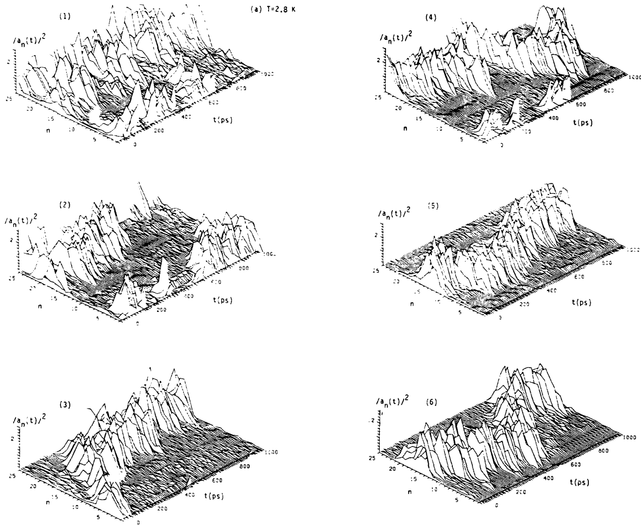
Fig. 2. Evolution of the excitation probability |a_n(t)|^2 from an initially randomly distributed amide-I quantum as function of site n and time t in cyclic chains of 25 units and with symmetric interaction, using the |D_1\rangle ansatz state and Davydov's model for temperature effects. Each subfigure (1–6) shows every 5 000th of 500 000 time steps each ( \tau = 2 \text{ fs} ). (a) T = 2.8 \text{ K} ; (b) T = 7.0 \text{ K} ; (c) T = 11.2 \text{ K} .
