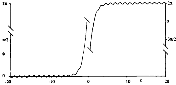
Fig. 2. Travelling kink for the DSG equation, c = 0.316228 , \Gamma = 1 .
