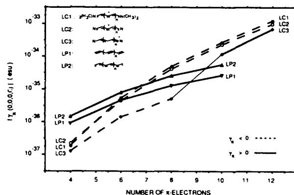
Fig. 2. Calculated |\gamma_\pi(0; 0, 0, 0)| 's for the five sets of molecules shown in fig. 1.
