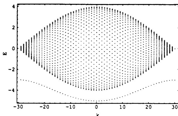
Fig. 5. Quantum energy levels for the DNLS equation.
