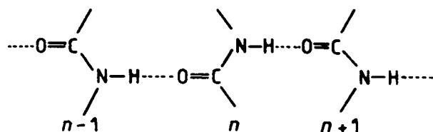
Fig. 1. Schematic picture of a hydrogen bonded channel in a protein.
