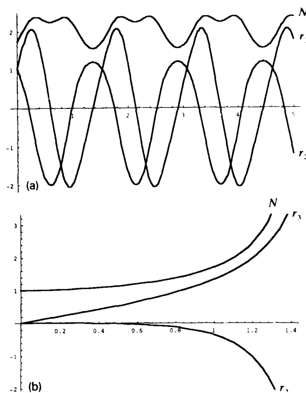
Fig. 1. Solution of eqs. (14) with (a) \gamma = 2 , \beta = 1 , \epsilon = 0.5 , N(0) = 1.732 , r_2(0) = 1 , r_3(0) = 1 , r_1 = 1 ; (b) \gamma = -1 , \beta = 1 , \epsilon = 1 , \alpha = 0.5 , N(0) = 1 , r_2(0) = 0 , r_3(0) = 0 , r_1 = 1 .
