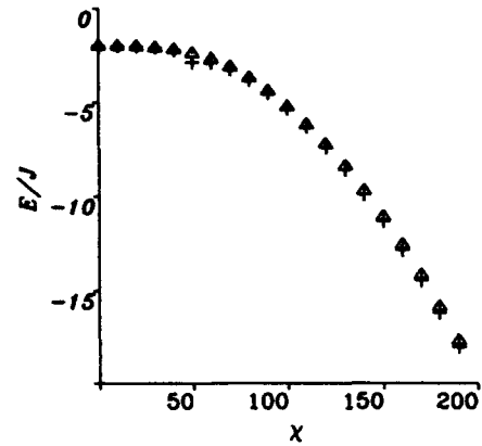
Fig. 1. Variation with \chi of the energy of minimum energy excited states determined with semiclassical Davydov model (triangles) and with the full quantum mechanical model (crosses). N=50 , J = 1.549 \times 10^{-22} J, \kappa=13 N/m.
