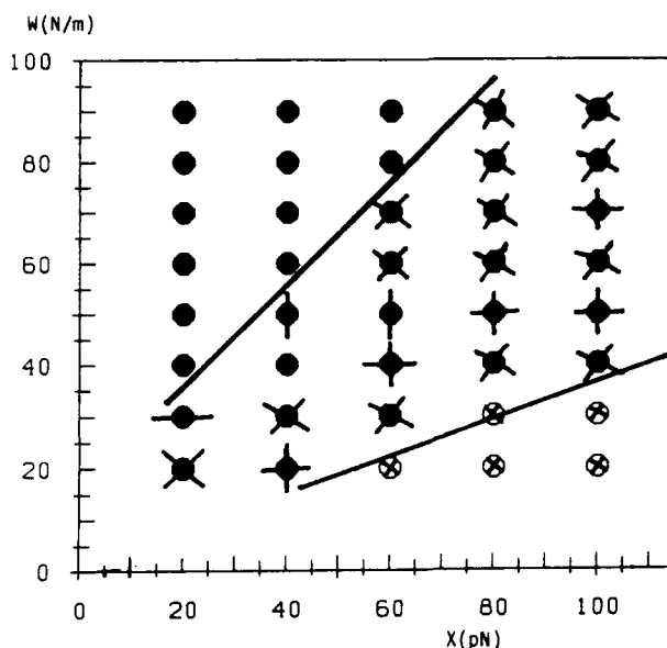
Fig. 4. Survey of the (X, W) parameter space at T = 300 K using Davydov's temperature model and the |D_1\rangle ansatz state together with a mass of 3M = 342m_p (initial excitation at site 49, time step 0.15 fs, chains of 50 units, crossed open circles: pinned soliton, horizontally dashed black circles: pinning or reflection after roughly 40 sites, vertically dashed black circle: slowly dispersive solitary wave, horizontally crossed black circle: soliton which becomes pinned after a few sites, diagonally crossed black circle: moving soliton which becomes pinned after interaction with the shock wave and then slowly disperses, black circle: travelling soliton).
