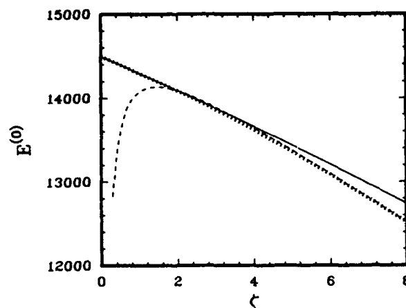
Fig. 2. E^{(0)} vs. \zeta : exact value (—), small \gamma perturbation theory (---) and small J perturbation theory (·····). The parameters \omega_0 = 3000 and J = 100 and the quantum level n = 5 used here are realistic for modeling carbon-hydrogen stretch vibrations in molecules.
