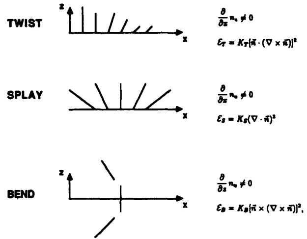
Fig. 3. Schematic of the “twist”, “splay”, and “bend” elastic distortions of the nematic.
