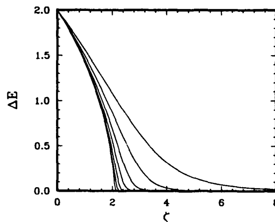
Fig. 3. Computed splitting \Delta E between the two lowest QDST energy levels for a given n vs. \zeta for (from right to left) n = 6, 12, 25, 50, 100, 200 and 400 , J = 1 and \omega_0 = 0 .
