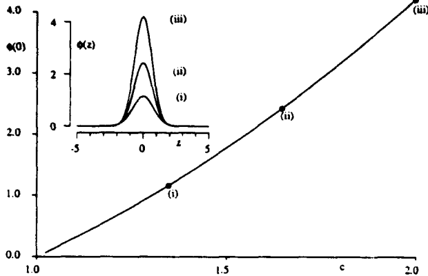
Fig. 1. Travelling waves for the case V'(q) = q + q^2 .
