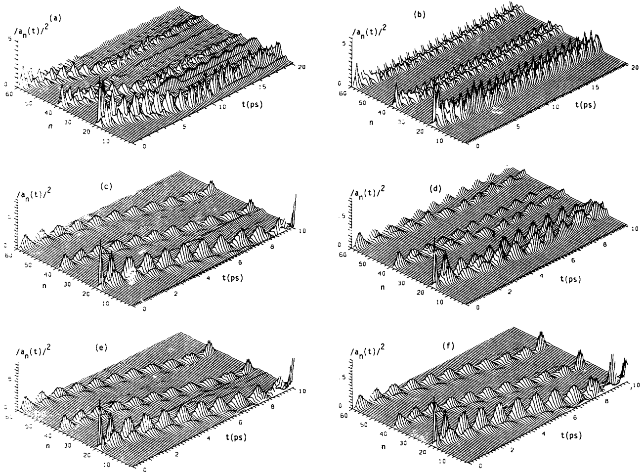
Fig. 5. Time evolution of |a_n(t)|^2 in the |D_1\rangle ansatz state at 300 K using Davydov's model for temperature effects and a localized initial excitation ( a_{10,1}(0) = 1 , all other a 's equal 0.005, then normalized to 1, all three chains are shown: chain 1: n = 1-20 , chain 2: n = 21-40 , chain 3: n = 41-60 , time step: 0.25 fs) for different values of W and X :
