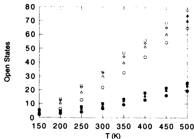
Fig. 2. Number of open states of hydrogen bonds versus temperature, T , with life-times: 5–20 psec (open symbols), longer than 20 ps (full symbols). Homogeneous chain (circles), inhomogeneous chain with prevalence of bases of strong type (triangles), homogeneous type (diamonds), and weak type (squares).
