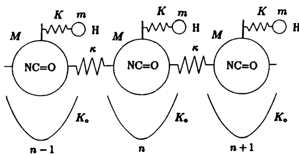
Fig. 1. Schematic representation of the chain model of hydrogen-bonded PGs.
