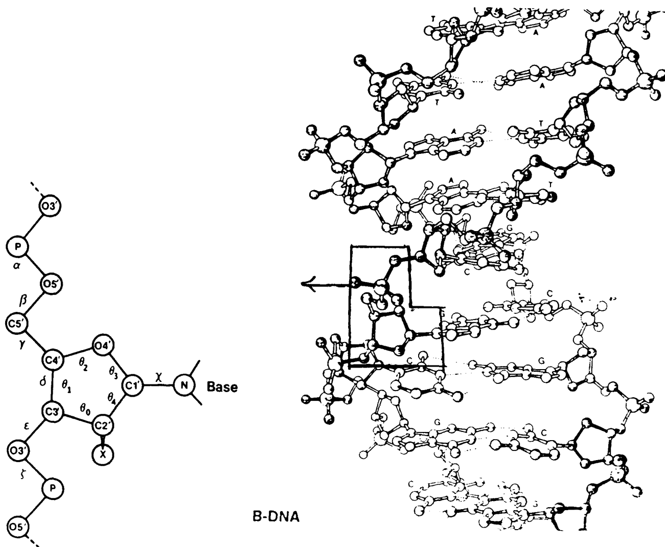
Fig. 1. IUPAC nomenclature for backbone torsion angles, ribose endocyclic torsions, and the glycosidic torsion. The backbone torsion \delta is defined by the four atoms O3'-C3'-C4'-C5' , while the endocyclic ribose torsion about the same bond, \theta_1 , is defined by C2'-C3'-C4'-O4' . The proper definition of \chi is O4'-C1'-N1-C2 for pyrimidines and O4'-C1'-N9'-C4 for purines.
