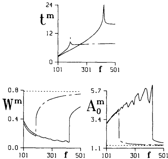
Fig. 4. t^m , W^m and A_0^m (defined in text) as function of f with L = 25.6 . (---) \sigma = 1.95 and (—) \sigma = 1.99 . Initial values of W^m and A_0^m are shown as dashed lines.
