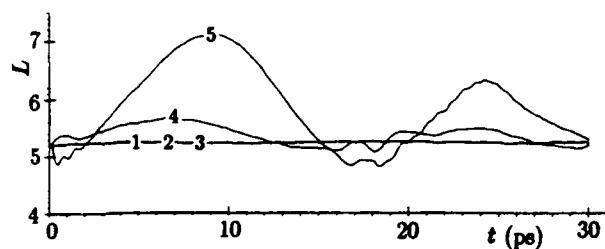
Fig. 2. Time dependence of the soliton width L(v=0) in the thermalized chain with \chi_1 = 1 \times 10^{-10} N and \chi_2 = 0 at t_c = 0.1; 0.07; 0.04; 0.01; 0.001 ps (curves 1, 2, 3, 4, 5, respectively).
