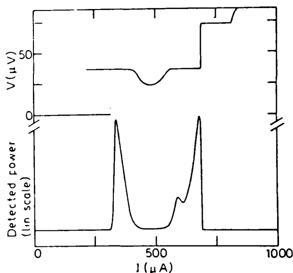
Fig. 6. IV curve a and half harmonic microwave power. Experiments after ref. [24].
