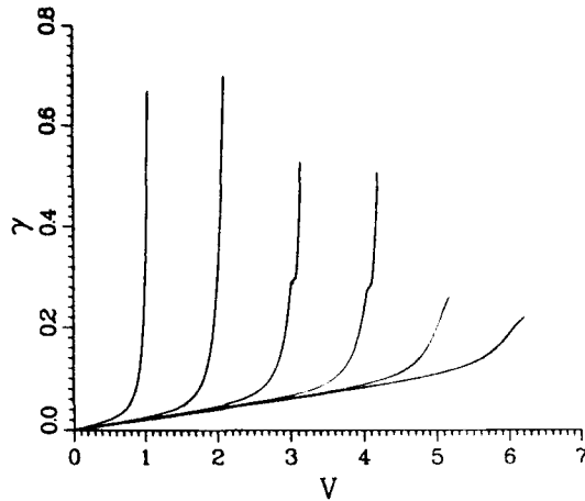
Fig. 1. The calculated I - V curves of the annular Josephson junction with different numbers n = 1, \dots, 6 of trapped solitons.
