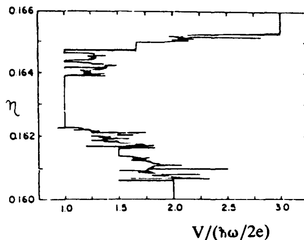
Fig. 5. Numerical calculation of phase locking steps of an IV curve. \Omega = 0.16 , \alpha = 0.5 , \eta_1 = 1.05 . After ref. [22].
