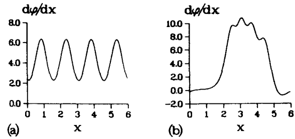
Fig. 3. The spatial distribution of the normalized magnetic field in the junction on step 4 at \gamma = 0.26 (a) and at \gamma = 0.34 (b).
