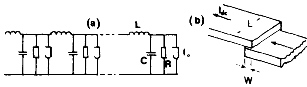
Fig. 1. Equivalent diagram (a) and schematic drawing of a long Josephson junction.
