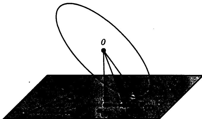
Figure 29: In this figure, the shaded area is \mathcal{E} = e_{(0)} + \text{span}\{d_{(0)}, d_{(1)}\} . The ellipsoid is a contour on which the energy norm is constant. After two steps, CG finds e_{(2)} , the point on \mathcal{E} which minimizes \|e\|_A .
