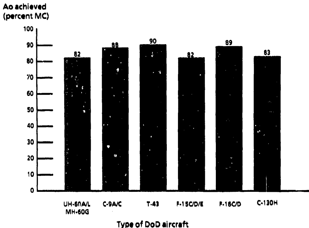
FIG. 2-2. SAMPLE DoD ACHIEVED AIRCRAFT AVAILABILITIES
