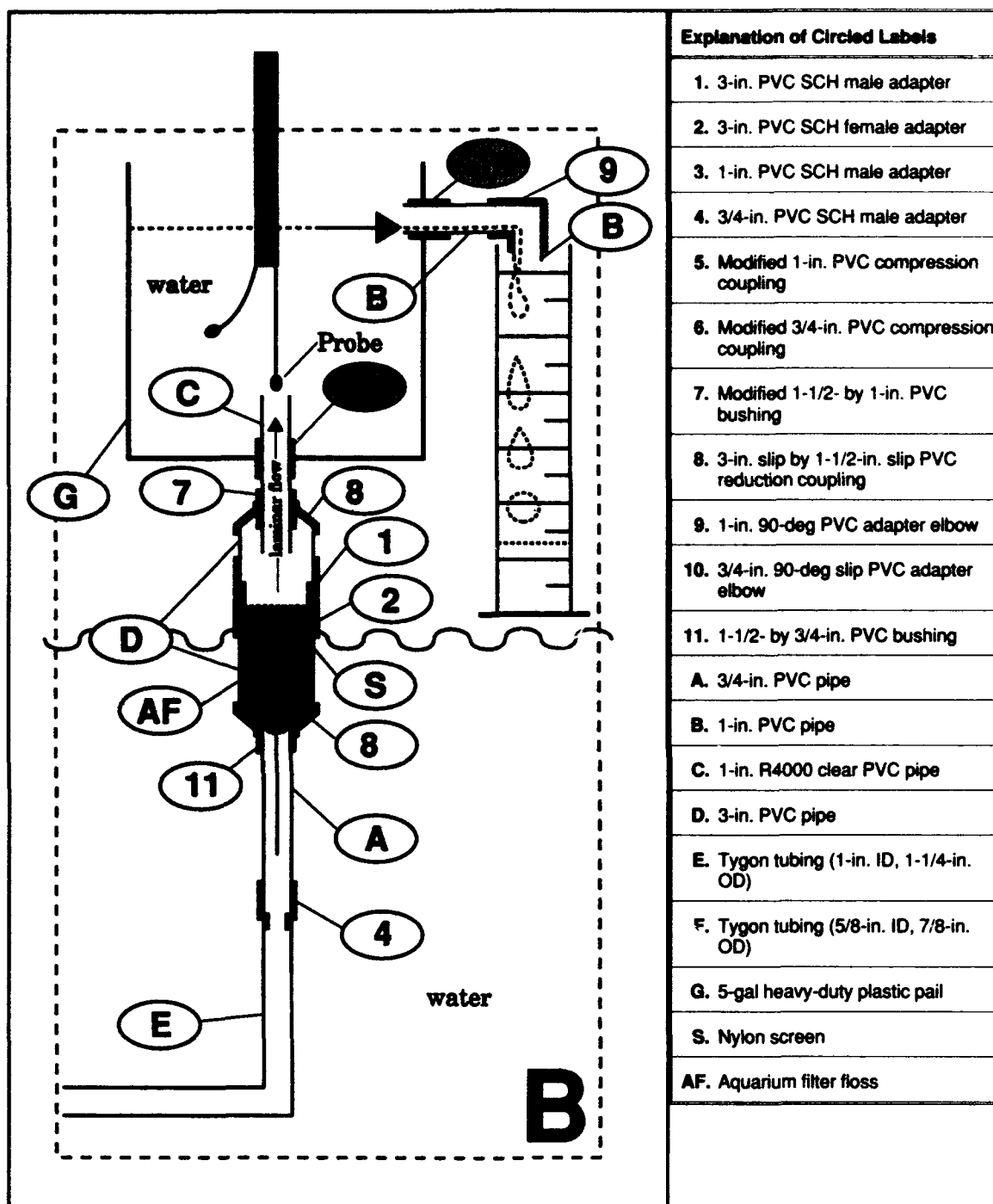
Figure 3. Details of Figure 1 (dashed outline box B) giving components for construction. Laminar flow is achieved at the point where the sensor thermistor (probe) is positioned. Careful increase of the bore of 7 (1-1/2- by 1-in. PVC bushing) allows snug fit of C (1-in. clear PVC pipe) which must pass through bushing. It is fused in place with PVC plumbing cement. All PVC slip fittings are fused with PVC plumbing cement. Modifications of 5 are presented in Figure 4
