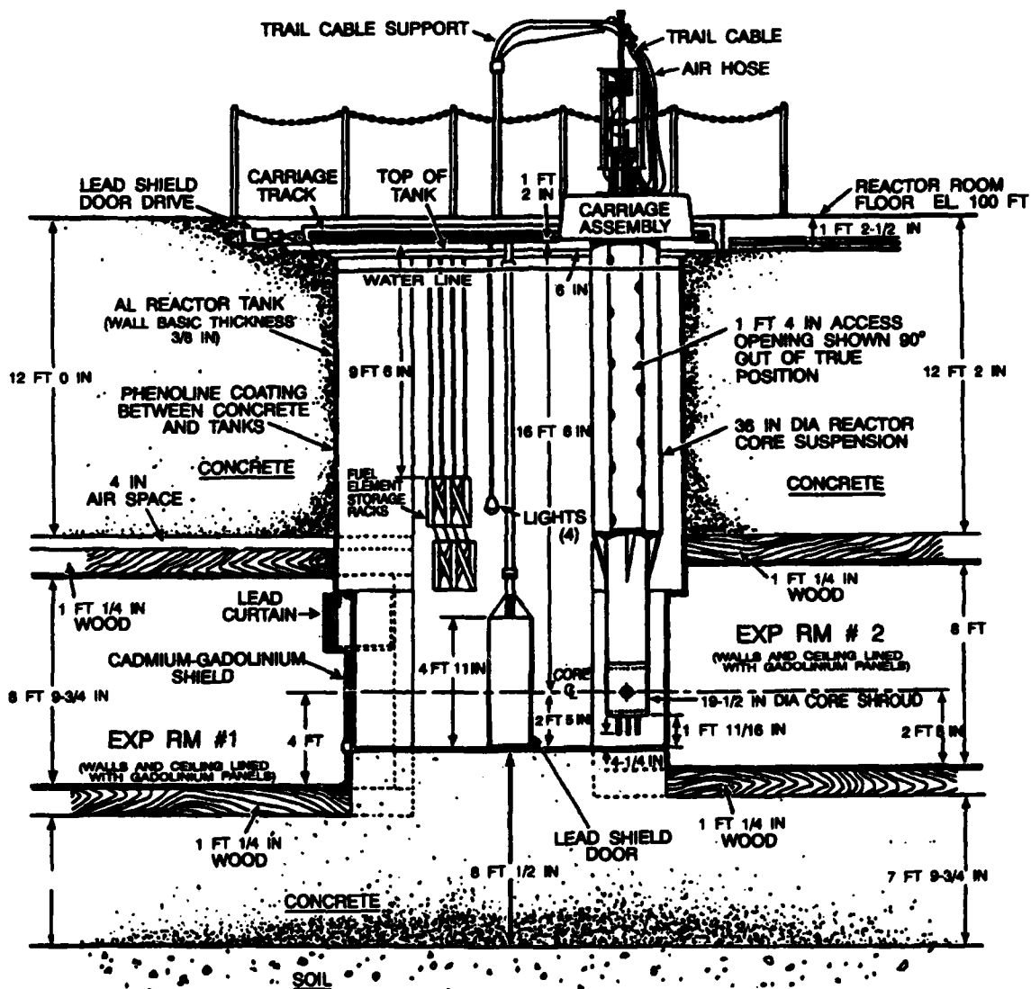
Figure 5. Side view of reactor and exposure facilities.
