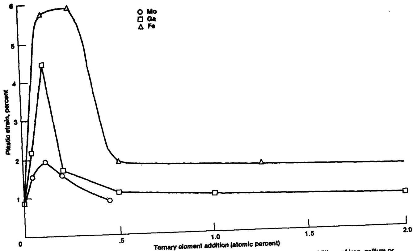
Figure 35.—Room temperature tensile ductility of <110> single crystal NiAl with microalloying additions of iron, gallium or molybdenum (ref. 62).
