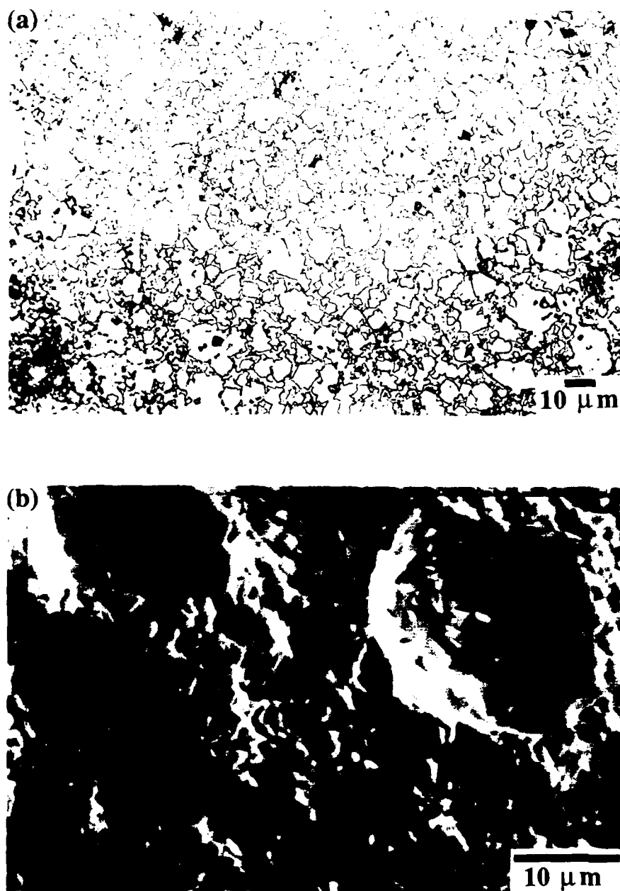
Figure 13 (a) Optical and (b) SEM micrographs of SLS sintered (WC-12 wt.% Co)-20 wt.% Co-10 wt.% Ni sample.
