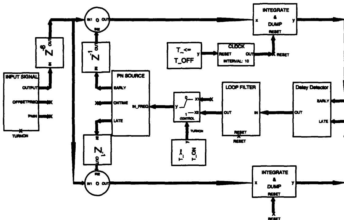
FIGURE 3 DELAY LOCK LOOP MODEL
