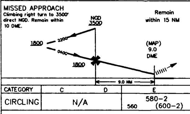
d. Approach to Pegasus Ice Runway 32G.
