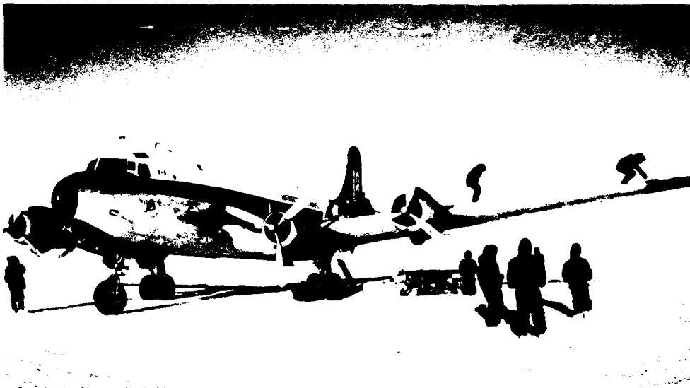
Figure 13. Antarctic Airways DC-4. Some 31 years after the DC-4 began flying to McMurdo, and almost 50 years after the first flight of its prototype, the same type of aircraft opened commercial service to Antarctica. A DC-4 of Antarctic Airways (ANI/Borek) flew between Punta Arenas and Patriot Hills, carrying climbers and tourists. (Photo by Charles Swithinbank, 22 November 1987.)
