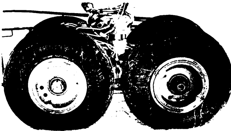
Figure 41. Wheels of the Ilyushin Il-18D. The eight 3-ft-diameter main wheels (930 x 305 mm) carry about the same gross weight as the four larger main wheels of the C-130. The standard inflation pressure is 114 lb/in. 2 (85 lb/in. 2 in the 700-x250-mm nosewheels). In principle, side-by-side wheels are preferable to wheels in tandem on a snow runway, since multiple passes of a wheel over soil or snow tend to cause progressive damage and rutting. (Photo by photographer's mate Craig Peterson, USN, November 1990.)
