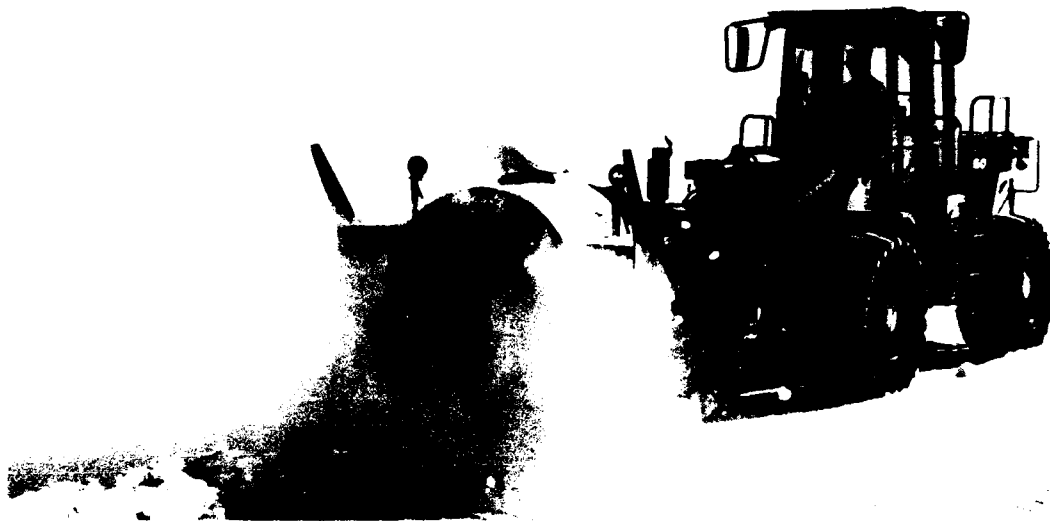
a. Single-stage, all-mechanical Blanchet with axial rotation. This unit concentrates a very heavy load on the front of the tractor when it is in the raised position.
