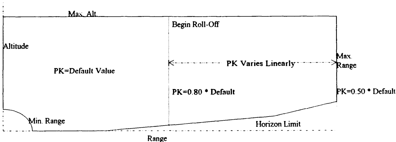
Figure 3 - Missile Lethality Envelope With P_K Roll-Off Enabled
