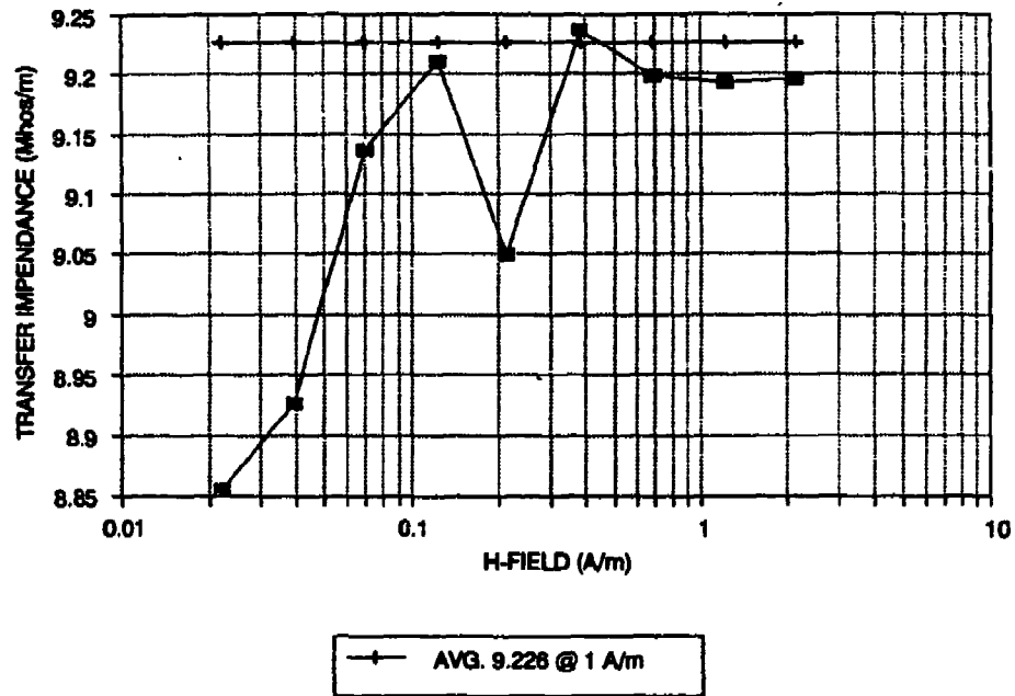
Figure B9. Calibration blue loop and DMM @ 19.8kHz 3/24/93 50-ohm termination HP-3468 PA 84147.
