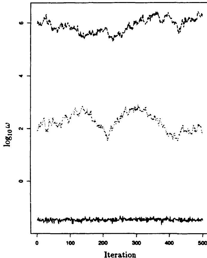
Figure 5.1: Three parallel Gibbs sampler series of \log_{10} \omega
