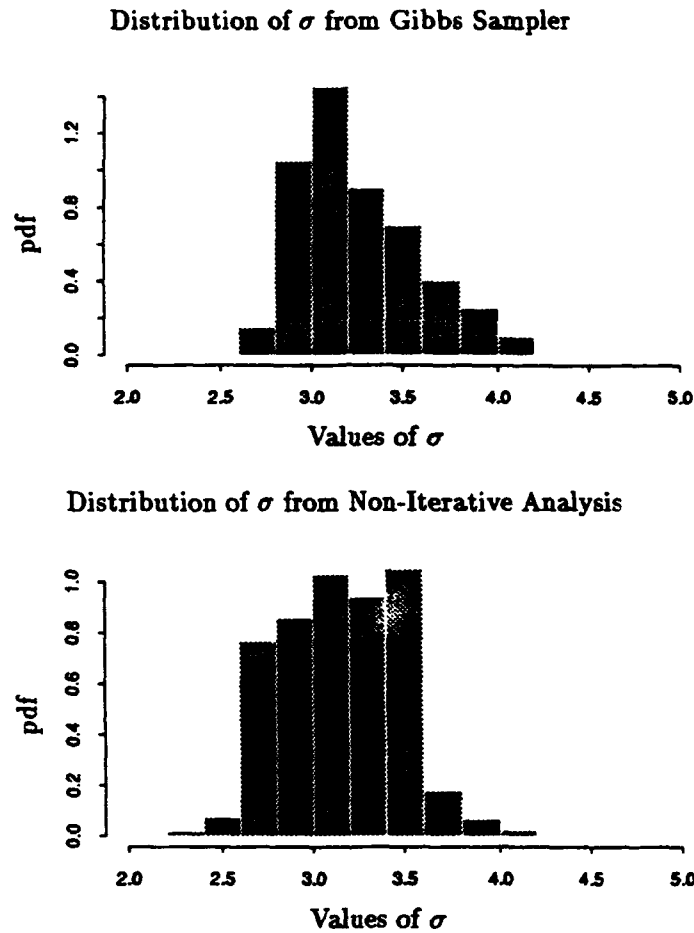
Figure 3.1: Posterior Distribution of \sigma
