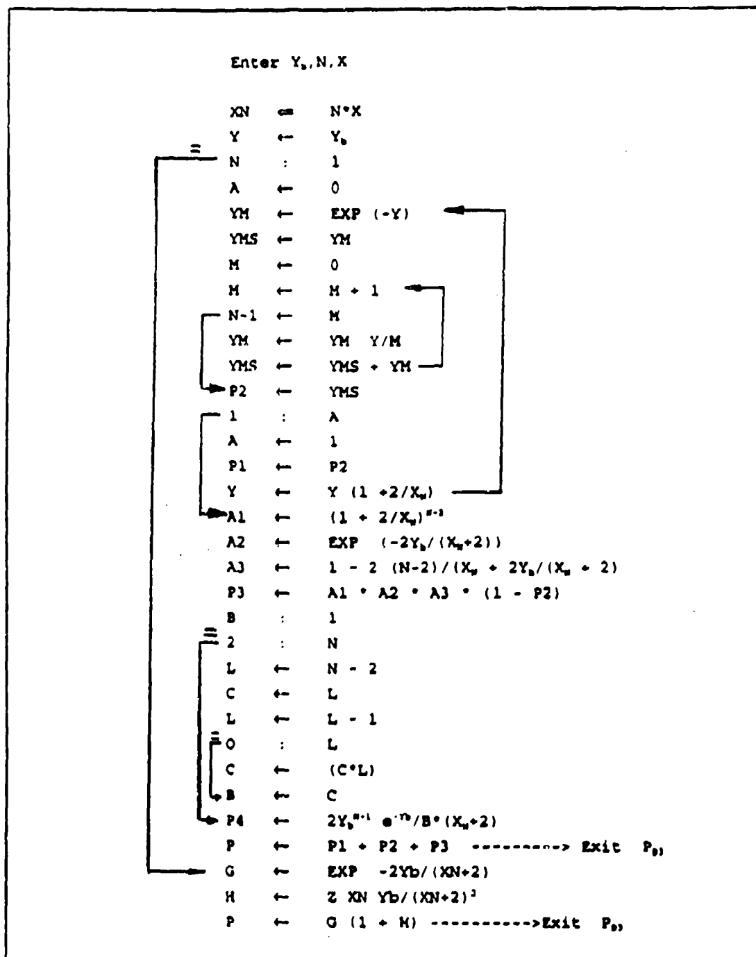
Figure 21: Algorithmic program for Swerling 3 Target, P_D ,
