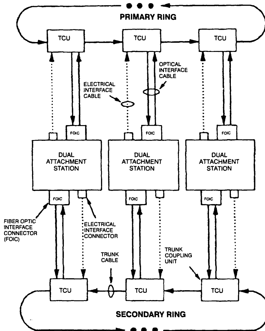
Figure 11. SAFENET topology.
