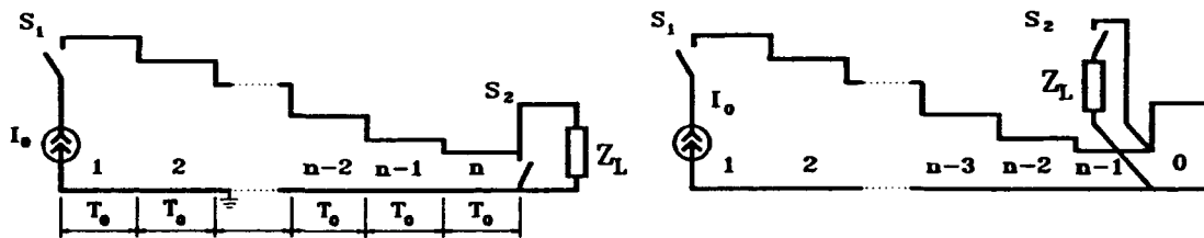
Fig.2. SFL and DSFL analogues with inductive energy
