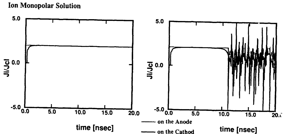
Fig. 9 Simulation of ion current density in ion injected diode.
