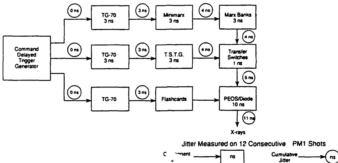
Figure 13. We have measured the switch jitter for all PM1 components.
