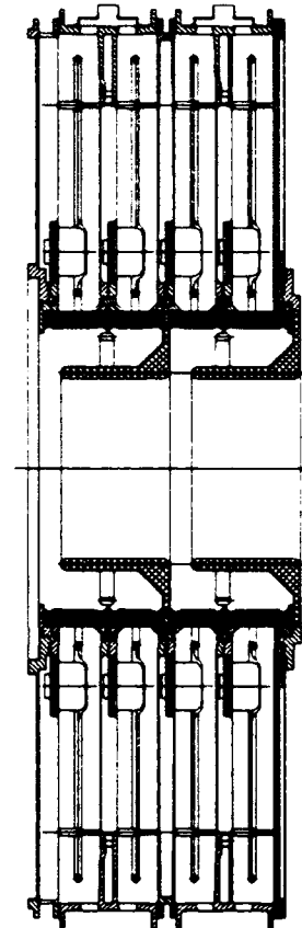
Figure 3 Schematic cross section of an accelerator unit.
