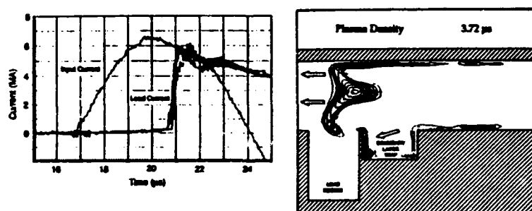
Fig. 2 Plasma trap catches boundary layer and improves switching performance.
