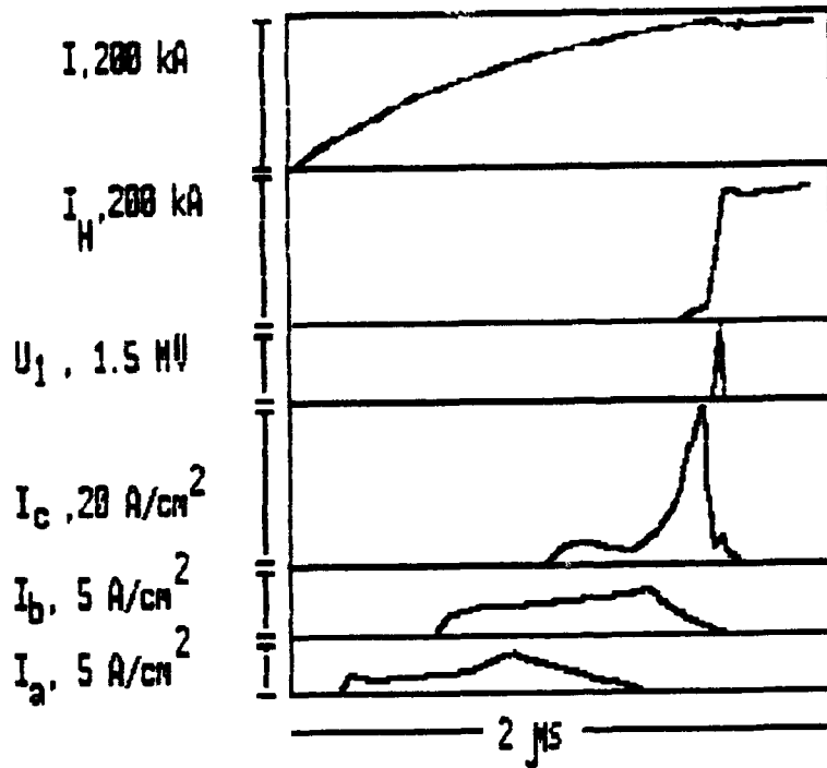
FIG.2-b Oscilloscopes: total current- I_0 , load current- I_H , PCIS voltage- U_1 , currents to the anode- I_a, I_b , I_c .
