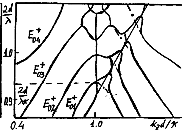
Fig.2 Dispersion characteristics
