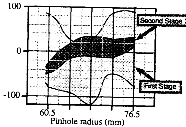
Fig. 8 Emittance plot of radial beam divergence in the first and second stage of two stage diode
