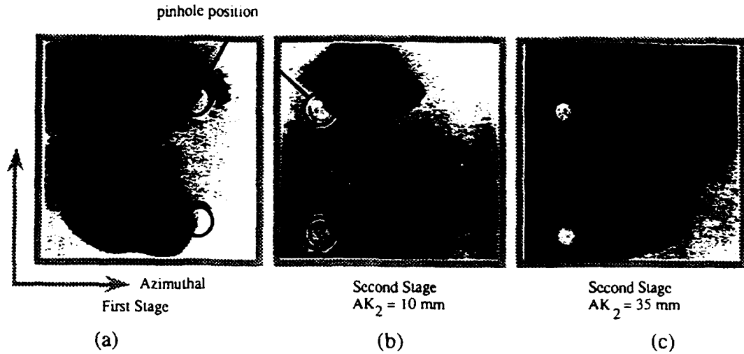
Fig. 7 Ion damages in the first (a) and second (b) stage at stable ion diode condition. (c) is the damage of untable condition
