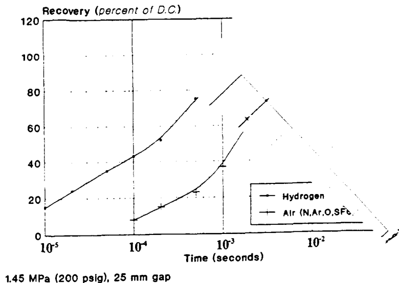
Figure 1. Recovery Curves for Common Gases
