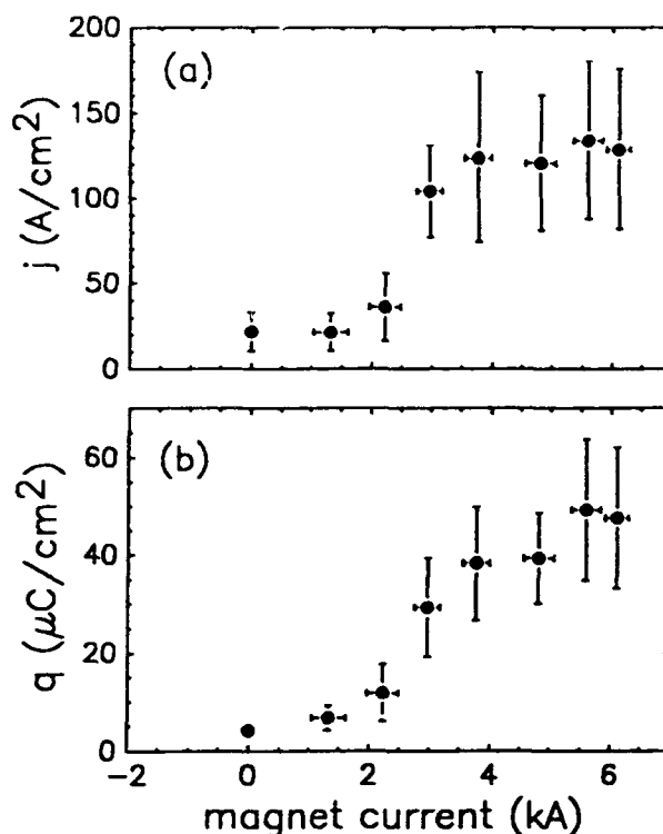
Fig. 4: Average (a) maximum ion current density and (b) integrated ion charge density obtained from the Faraday cup at r = 129 mm.
