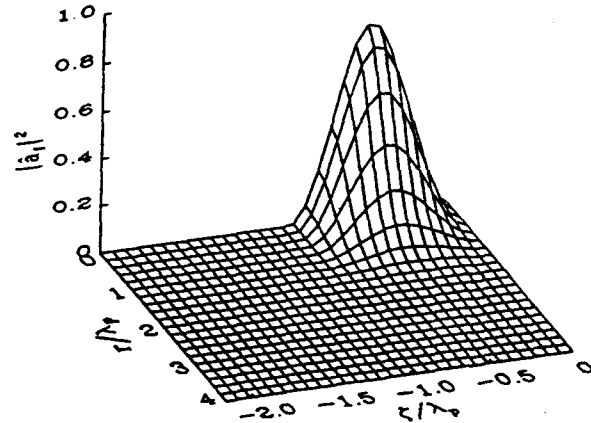
Fig. 2. Normalized laser intensity |\hat{a}_f|^2 in the speed of light frame (\zeta, \tau) at \tau = 0 for the parameters a_0 = 0.9 , L = r_L = \lambda_p = 0.03 \text{ cm} and \lambda = 1 \text{ }\mu\text{m} . The plasma flows from right to left.
