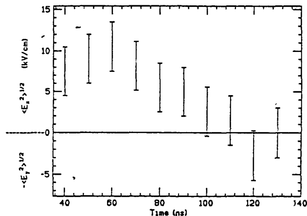
Fig. 2. Mean amplitude of the electric field \langle \epsilon_x^2 \rangle^{1/2} inferred as a function of time. Here, the plasma density was assumed to be 10^{15} cm -3 and the Doppler broadening was so chosen to provide an agreement between the calculated widths and the measured ones for each time instant. For the data point at 120 ns the width for the x -polarization was smaller than for the y -polarization (parallel to the anode and perpendicular to the applied magnetic field B_z ), which is inconsistent with the assumption of a one-dimensional field in the x -direction. For this point the same analysis is used to obtain a field in the y -direction with an amplitude \langle \epsilon_y^2 \rangle^{1/2} , as shown in the Figure.
