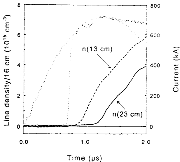
Figure 6: Average densities along lines of sight beyond the initial switch region.
