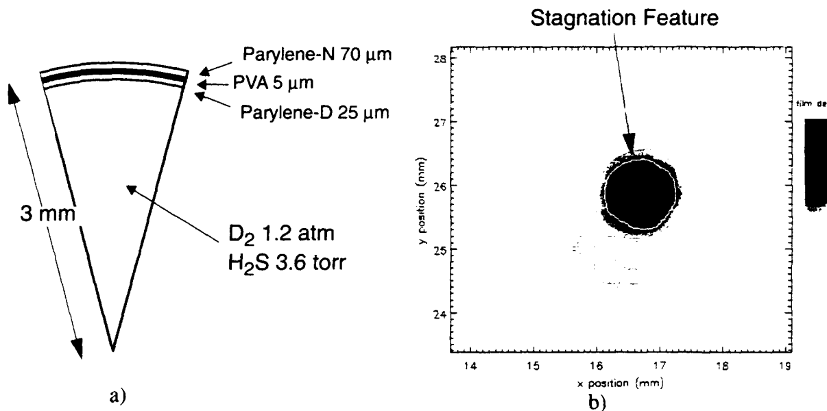
Figure 4. a) Pie diagram of a direct-drive exploding pusher target fielded on PBFA II and b) time-integrated x-ray image of the imploded target as viewed through a \sim 2 keV x-ray filter in the coordinate system of the film plane. Note the prominent central stagnation feature.
