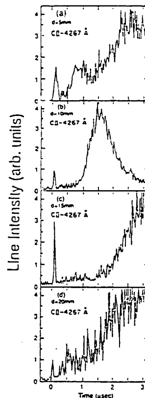
Fig. 7. Time dependent intensity of the CII 4267 \text{\AA} line measured at radial distances of 5, 10, 15, and 20 mm from the anode. The figure shows the early rise in the line intensity during switch operation followed by a secondary rise at times \geq 0.5 \mu s.
