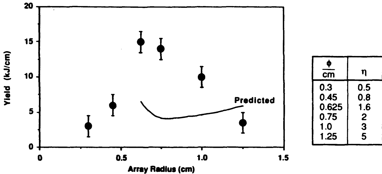
Figure 6. A comparison between the measured aluminium K-shell x-ray yields and those predicted by a 1D MHD code that only has kinetic energy input.
