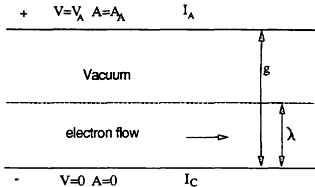
Figure 1. Schematic of a MIFL.
