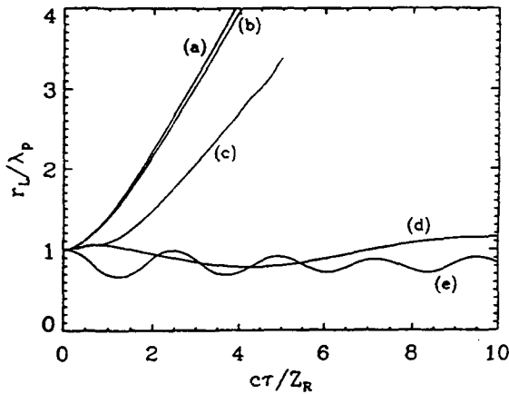
Fig. 1. Laser spot size r_L/\lambda_p (at \zeta = -L/2 ) versus propagation distance, c\tau/Z_R , for (a) vacuum diffraction, (b) pulse with L = \lambda_p/4 , (c) pulse with L = \lambda_p , (d) a shaped pulse and (e) a channel-guided pulse.
