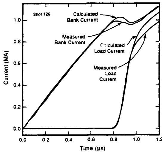
Figure 5. Comparison of magnetically enhanced ion erosion model with ACE 2 radial POS shot 126. 1 The interferometrically observed electron density at mid-gap was approximately 6 \times 10^{14} / \text{cm}^3 . The values v_T = 10^6 \text{ cm/s} , n_i = 7 \times 10^{14} / \text{cm}^3 , and Z = 2 were used in eq. (3).
