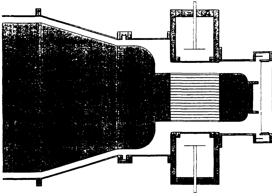
Figure 8. PEOS and pinched beam diode configuration.
