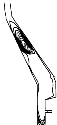
Fig. 3. Poloidal magnetic flux lines for the CT of Fig. 2 — 3 \mu s later.
