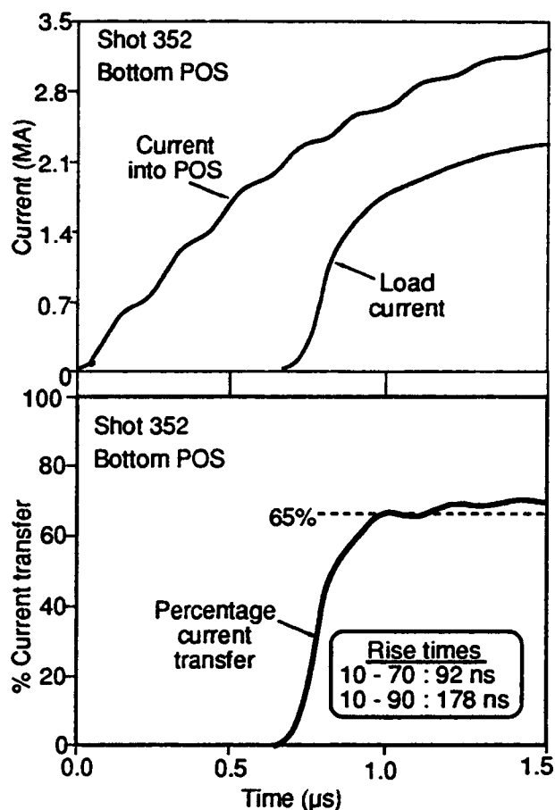
Fig. 4. ACE 4 summed current waveforms for the poor symmetry case.
