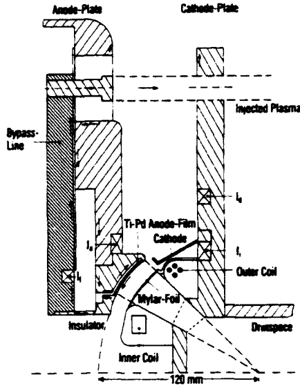
Fig. 1. Schematic diagram of the KALIF B appl. -extractor diode
