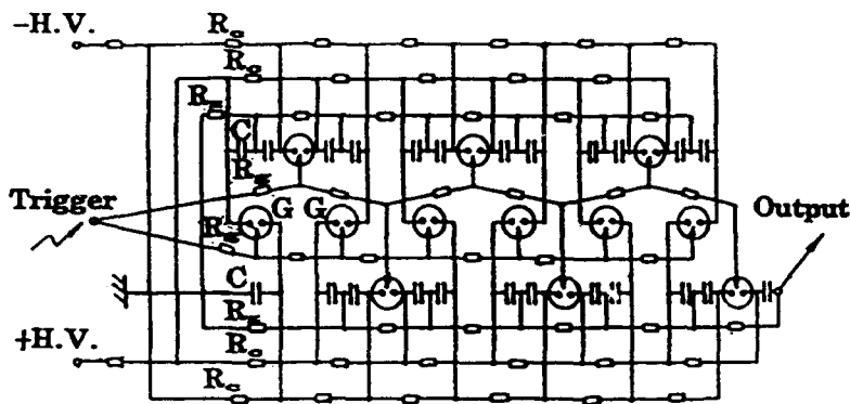
Fig.2 The circuit diagram of Marx generator C-capacitors G-spark gap switches R_c -charge resistors R_g -grounding resistors R_t -trigger resistors
