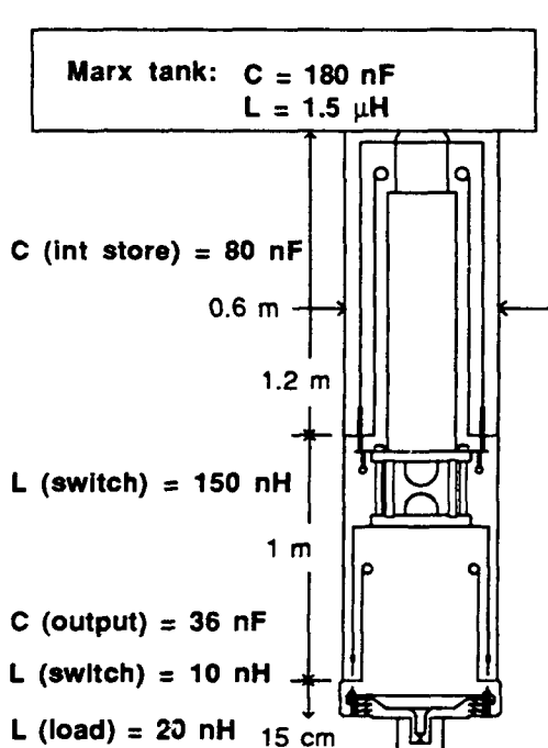
Figure 4: Schematic of the purpose built pulser showing the quadriaxial and triaxial capacitors.
