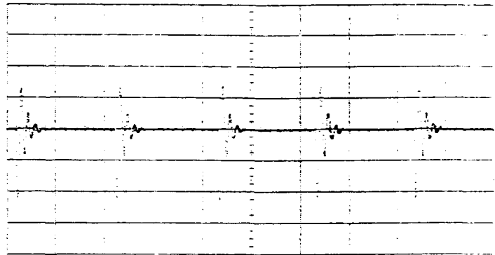
Figure 6. Current from a 5-Pulse Burst into a Resistive load. 10kA/div. vert., 50 \mu s/div. horiz.
