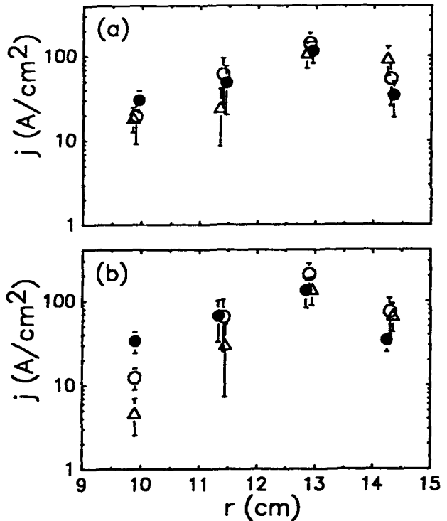
Fig. 7: Current density profiles for (a) solid and (b) perforated anodes, and 3 B-field configurations (o: inner coil I = 6 kA, outer coil I = 6 kA; ●: I_{in} = 6 , I_{out} = 3 kA; Δ: I_{in} = 3 , I_{out} = 6 kA).
