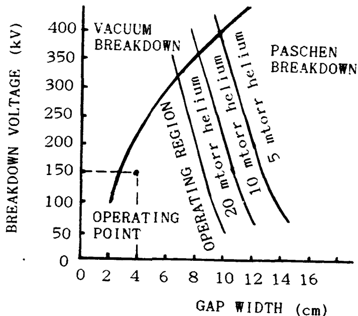
Fig. 2, Low-pressure breakdown voltage in the plasma accelerating region as a function of gap width
