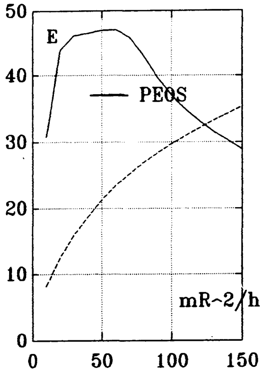
Fig.6 Liner kinetic energy E (kJ) as a function of ratio \alpha=mR^2/h ( \mu\text{g}\cdot\text{cm} ).
