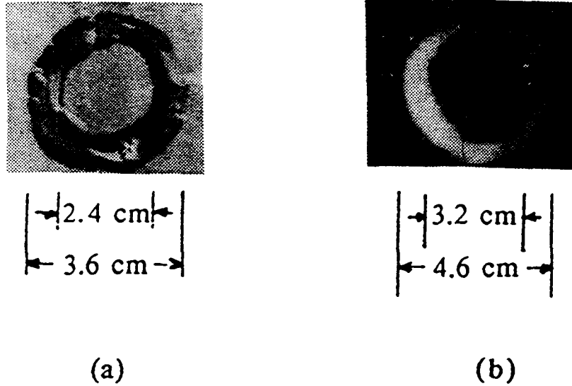
Fig. 3: (a) Witness foil of a 13-MeV, 78 kA-beam with \beta_{\perp} = 0.05 . (b) X-ray pinhole photograph of a 10-MeV, 80-kA beam with \beta_{\perp} = 0.07 .
