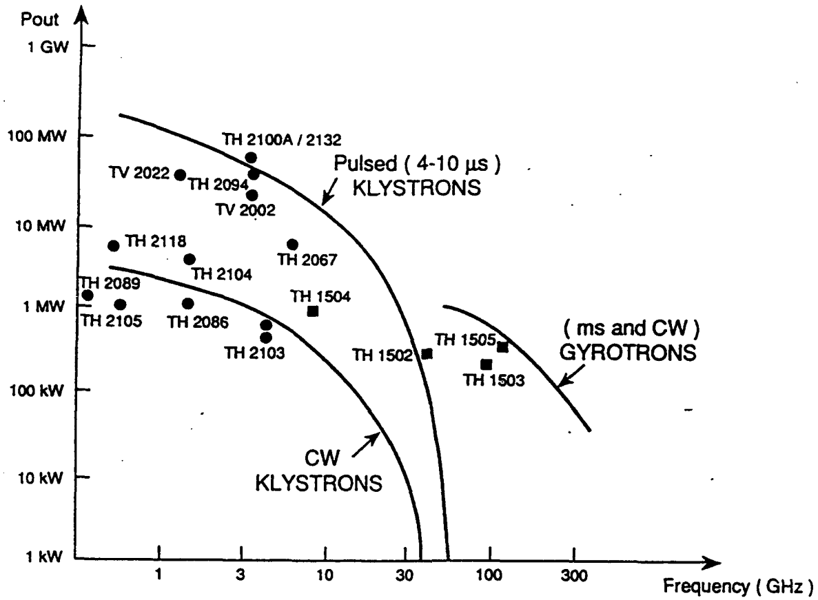
Fig.1 PRESENT TECHNOLOGY FOR PULSED AND CW HIGH POWER μW TUBES
