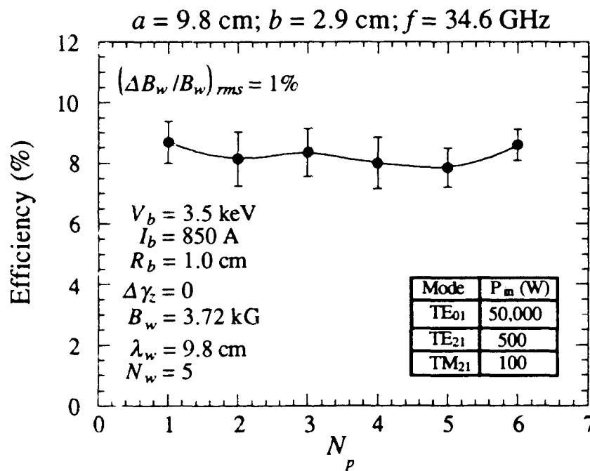
Fig. 2 Variation in the efficiency as a function of N_p for a 1% rms wiggler error.
