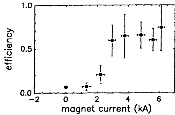
Fig. 6: Diode efficiency I_i/I_{tot} inferred from radially-weighted peak j_m(r) data.
