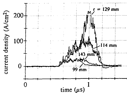
Fig. 3: Faraday cup signals at four different radii.
