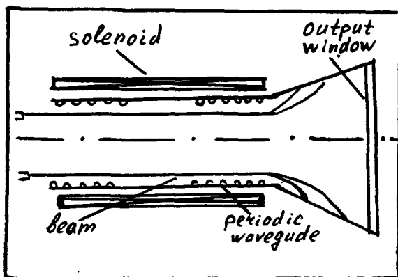
Fig.1 Two-sectional MWCG
