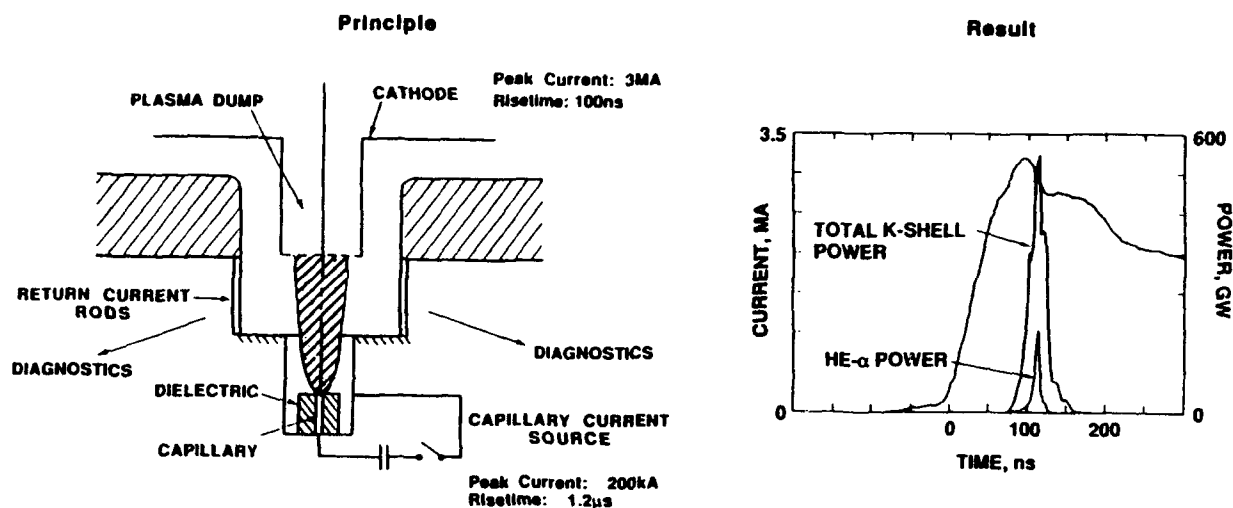
Figure 4. A schematic of the NRL NaF capillary discharge source fielded on Double-EAGLE. The plots show the measured K-shell and He- \alpha power pulse overlaid on the current waveform. This source produces 130 GW in the sodium pump line.
