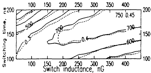
Fig. 8. Marx-output energy transfer efficiency (dashed line) and output pulse voltage (solid) vs gas switch inductance and trigger time of water switches. Load impedance 1.2 Ohm.
