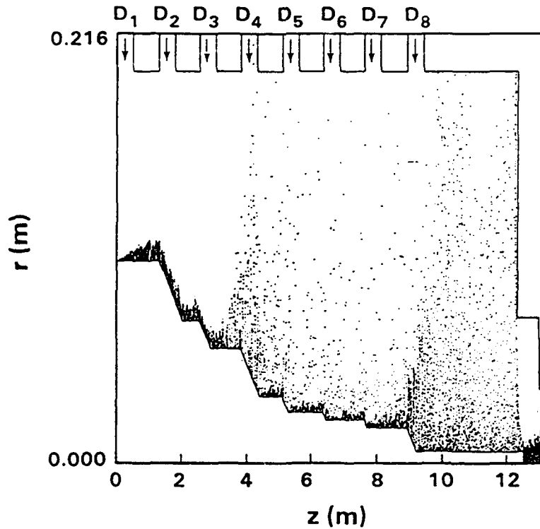
Fig. 1: Simulations showing magnetic insulation of SMILE.
