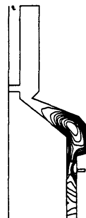
Fig. 6. Poloidal magnetic field contours for a CT trapped in a 60° self-similar compression cone.
