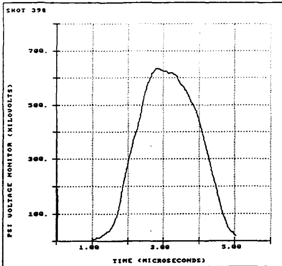
Fig.4a. Diode voltage with final diode configuration. Voltage exceeds 650 kV for 1 μs.
