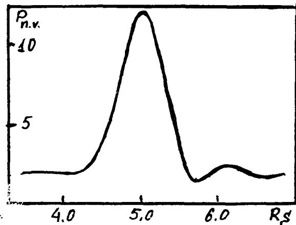
Fig.6 The dependence of output power from beam's radius.
