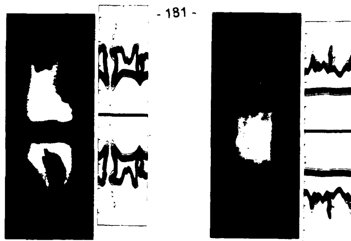
Fig. 4 Visible image and 2D MHD mass distribution for two direct drive experiments. 4.2 mg load (left figure) disrupts during implosion; 12.6 mg load (right figure) retains cylindrical symmetry throughout implosion; 2D MHD simulations reproduce observed scale of instabilities.
