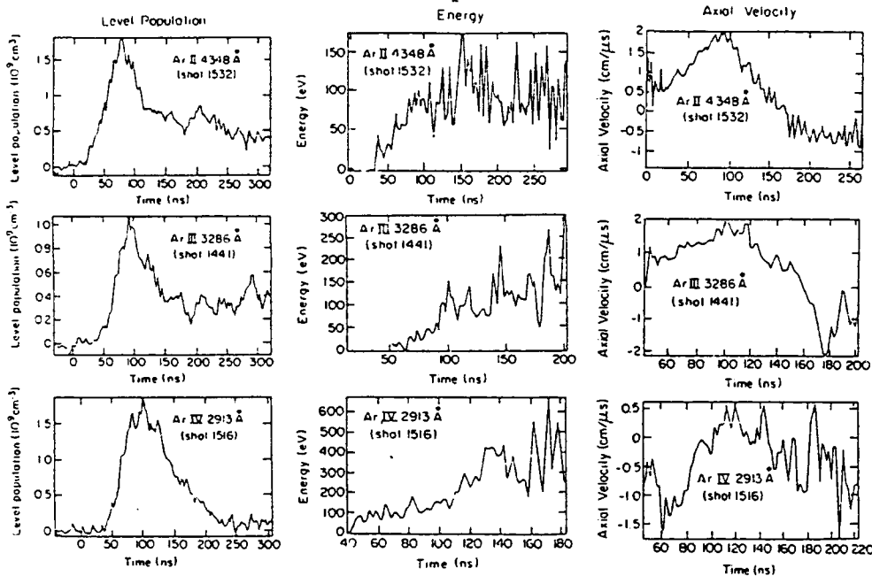
Fig. 6. Time dependent spectral observations of ArII, ArIII, and ArIV at 5 mm from the anode obtained from the 4348 \text{\AA} , 3286 \text{\AA} , and 2913 \text{\AA} lines, respectively. t = 0 is the start of the upstream current. (a) Time dependent absolute level populations of the above particles. (b) Time dependent mean kinetic energies obtained from the Doppler broadenings of the above particles. (c) Time dependent axial velocities obtained from the Doppler shifts of the above particles.
