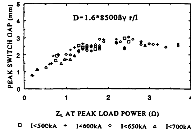
Fig. 6. Switch gap calculated at peak power, assuming the switch is at critical current, versus load impedance with the 10 cm diam cathode. The gap is independent of conduction current and, above the critical impedance, is fixed to 2.5-3 mm.
