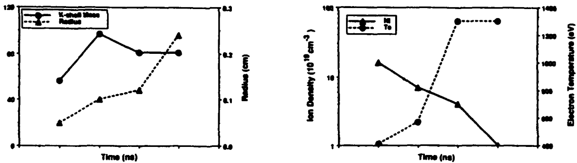
Figure 7. The measured k-shell radiating mass ( m_k ), plasma radius ( r_k ), electron temperature ( T_e ) and ion density n_i for a 15 mm diameter aluminium array.
