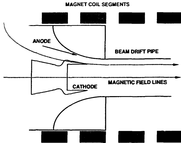
Fig. 5. Final diode configuration with the tapered anode. This configuration is used for all subsequent RKA development. Fig. 4. Redesigned diode showing cathode with contoured shape to match the fringing magnetic field curvature so as to reduce electron backstreaming and to converge the electron beam for maximum transmission into the drift pipe.
