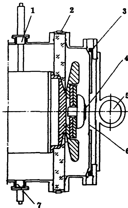
Fig.8 The diode and laser oscillator 1. resistance divider 2. current shunt 3. Rogowski coil 4. carbon felt cathode 5. laser cell 6. anode foil 7. capacitance divider
