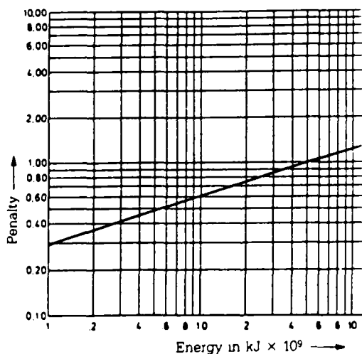
Figure 5: Penalty for quantity of energy present in the flammable material in process (ILO 1988:62)
