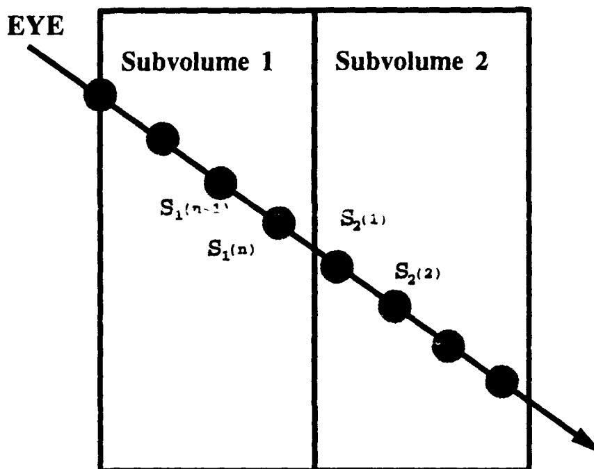
Figure 3: Correct Ray Sampling.
