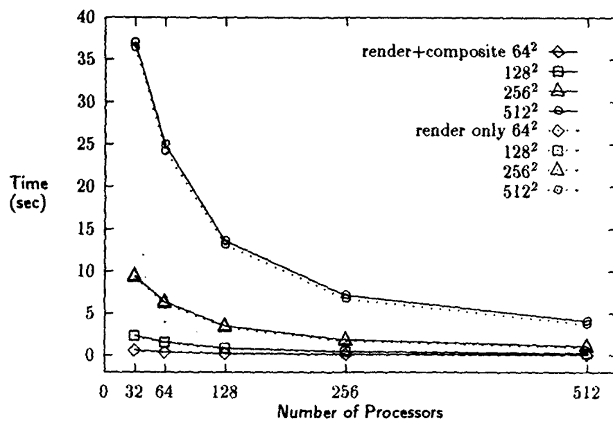
Figure 7: CM-5 Times for the Head Data Set.
