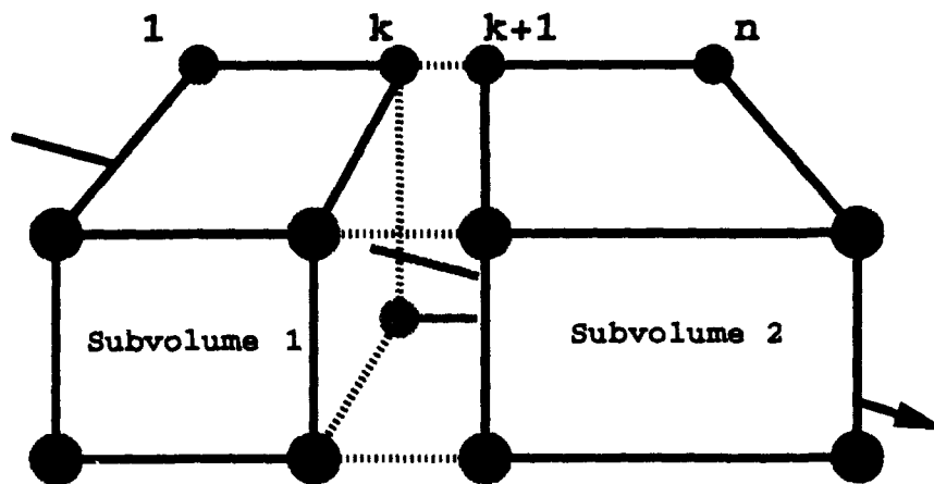
Figure 2: Volume Boundary Replication.
