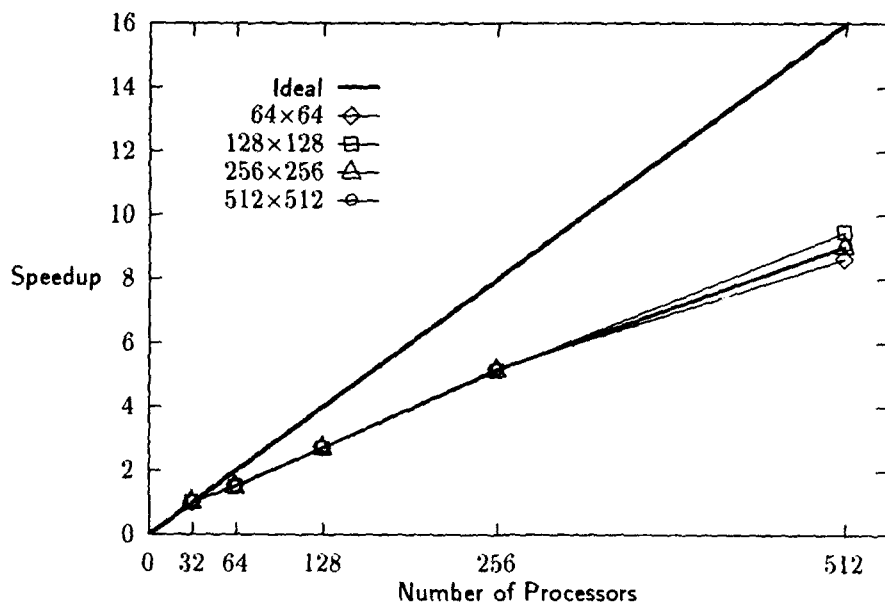
Figure 8: CM-5 Speedup for the Head Data Set.
