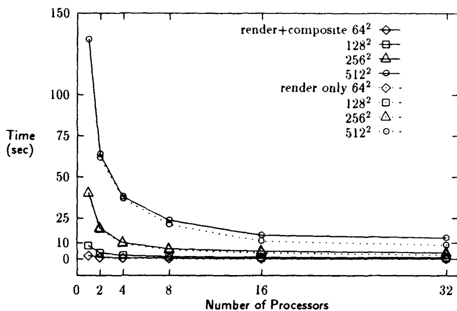
Figure 14: PVM Results on the Head Data Set.
