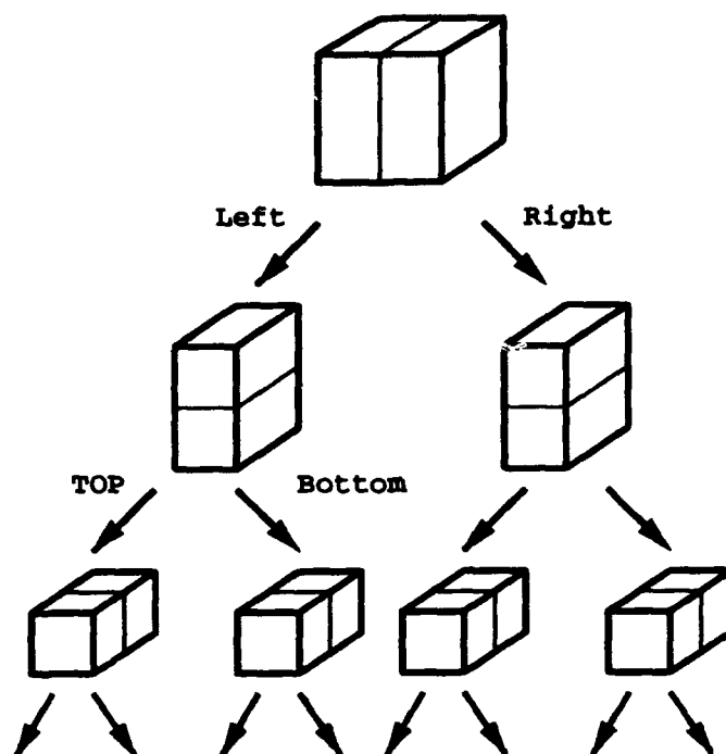
Figure 1: k-Dtree Subdivision of a Data Volume
