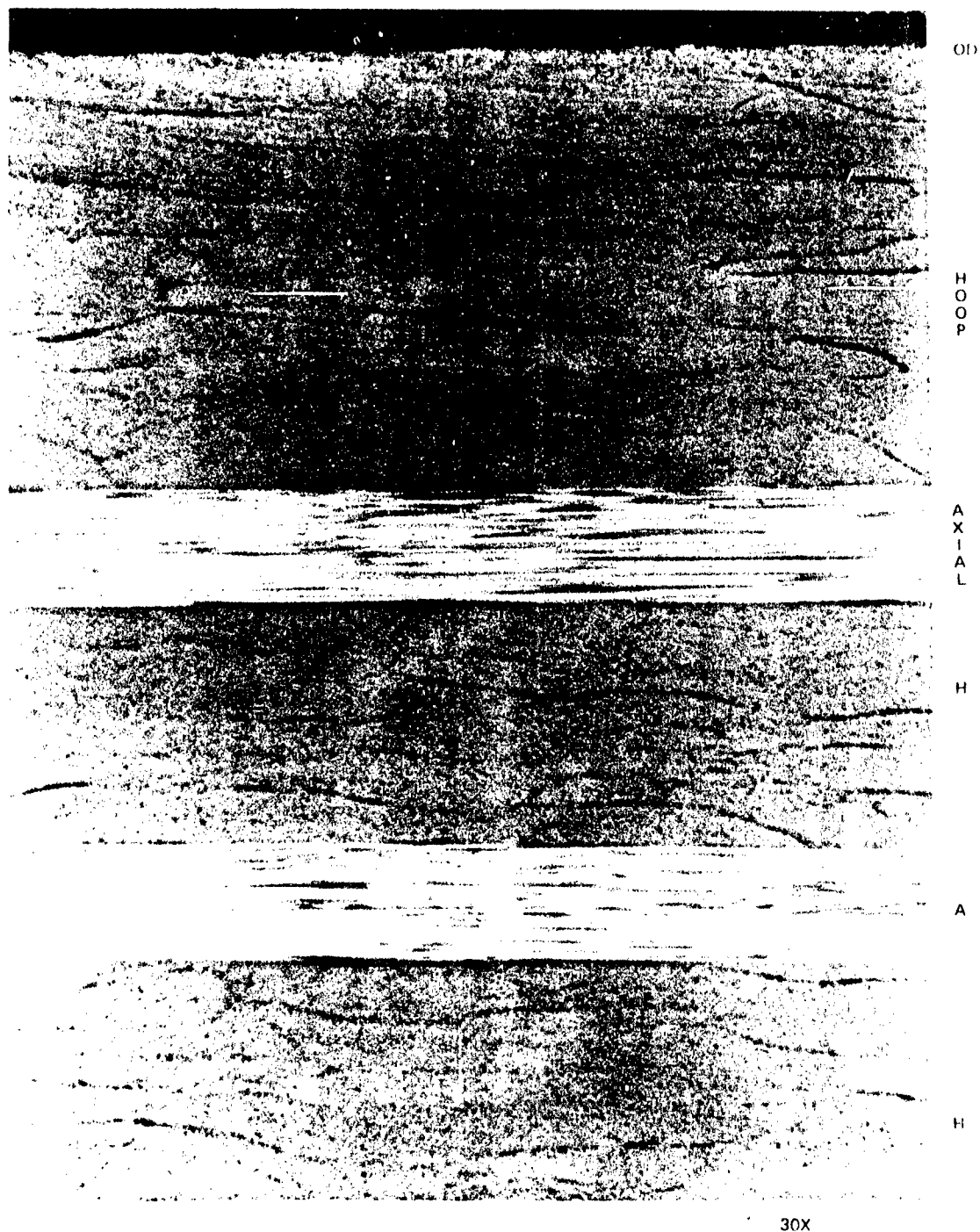
Figure 51. Typical quality of the composite in the last five laminae under the exterior surface of the composite in the AUSS Mod 2 hull; the hoop winding on the exterior surface is 0.048-inch thick.
