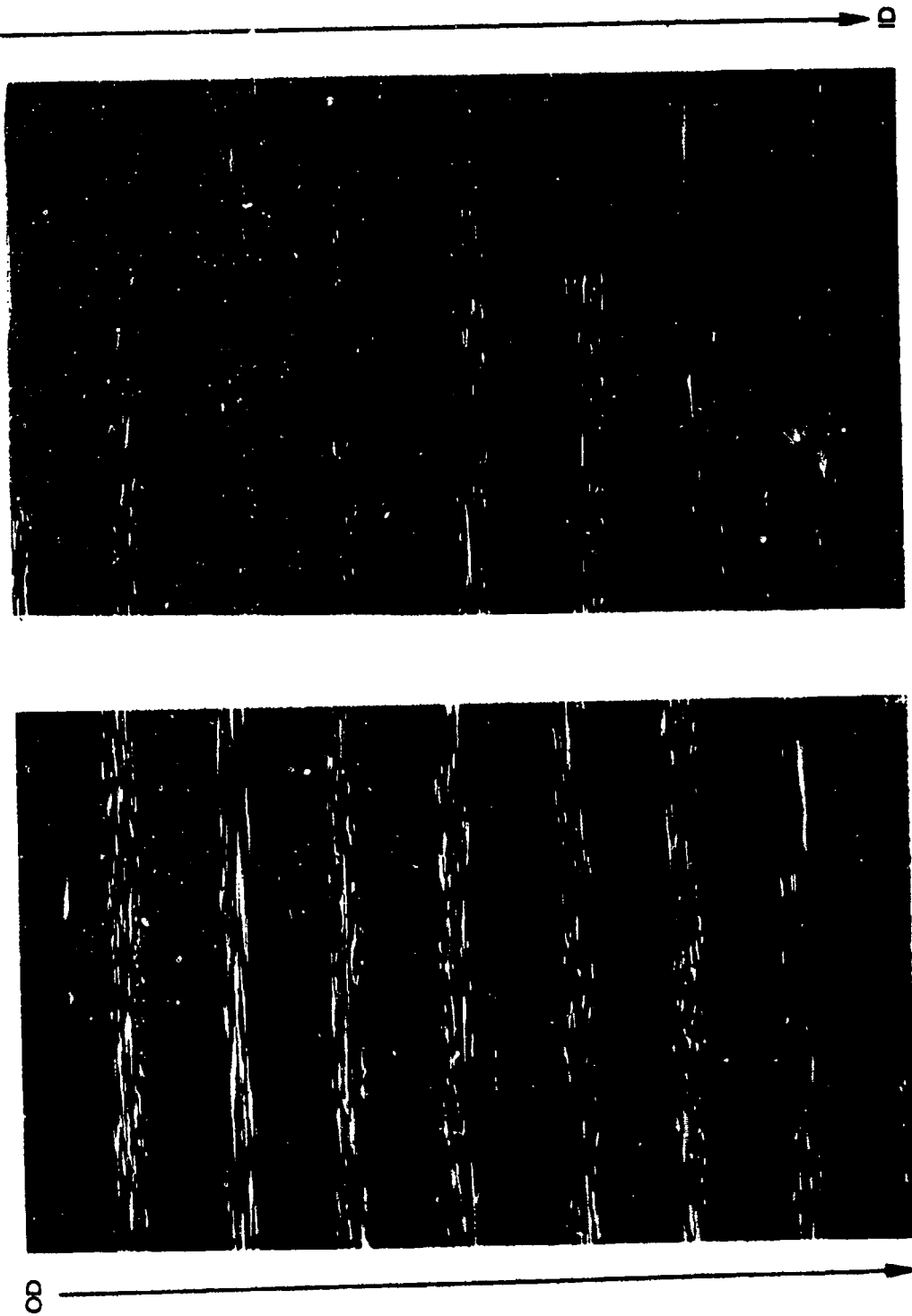
Figure B-4. Cross-section of model-scale GFRP cylinder under 20 X magnification; average layer thickness is 0.024 in hoop and 0.124 in axial.
