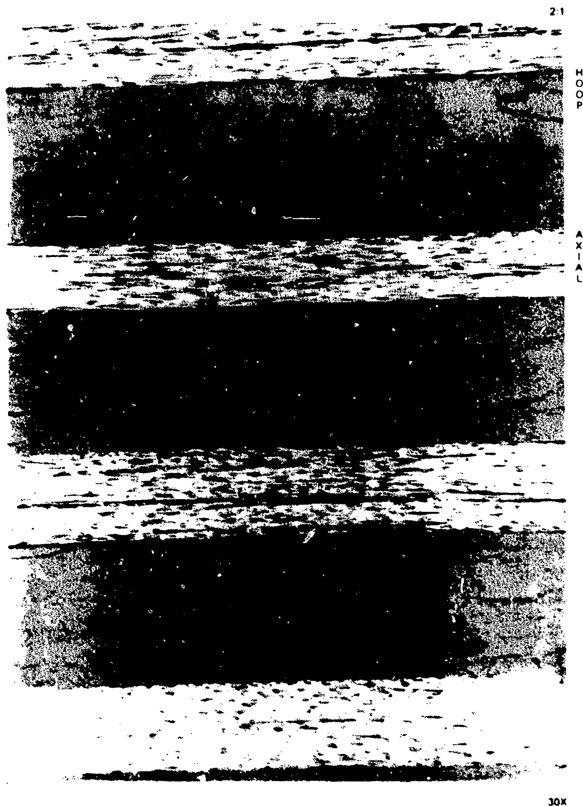
Figure 48. Typical quality of the composite in the AUSS Mod 2 hull. the construction of the composite in the 1 to 2.5 inch thickness interval displays a 2:1 ratio of hoop to axial-oriented fibers. The alternating hoop and axial oriented laminas are 0.027 and 0.0136 inch thick, respectively.
