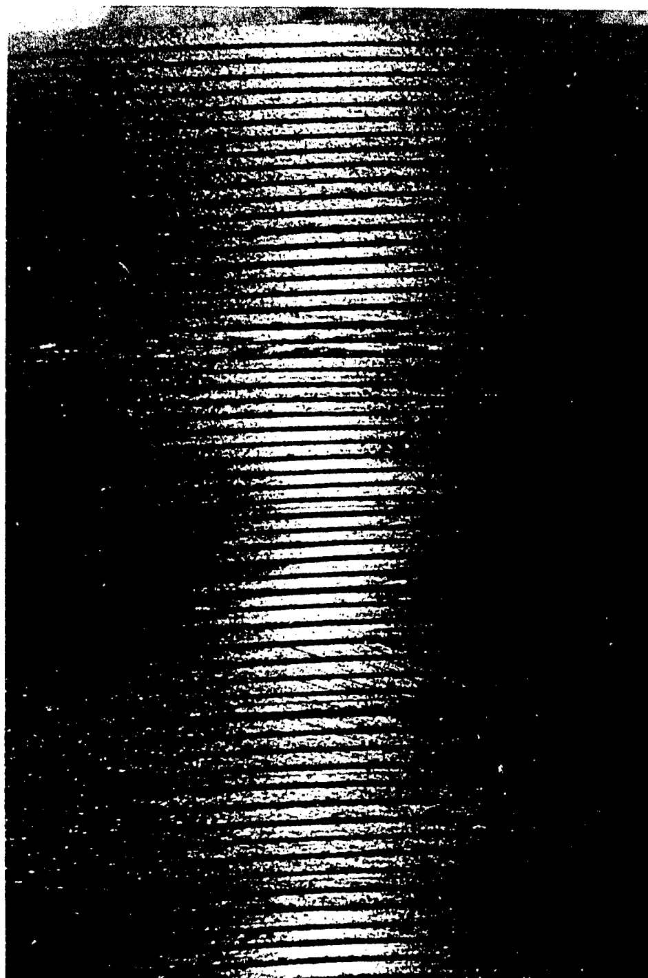
Figure 52. Overall view of the wall cross-section in AUSS Mod 2 hull. Note the uniformity and circularity of the individual hoop laminae in the composite indicating the high quality of fiber winding procedure employed by Martin Marietta Energy Systems to fabricate the cylinder.
