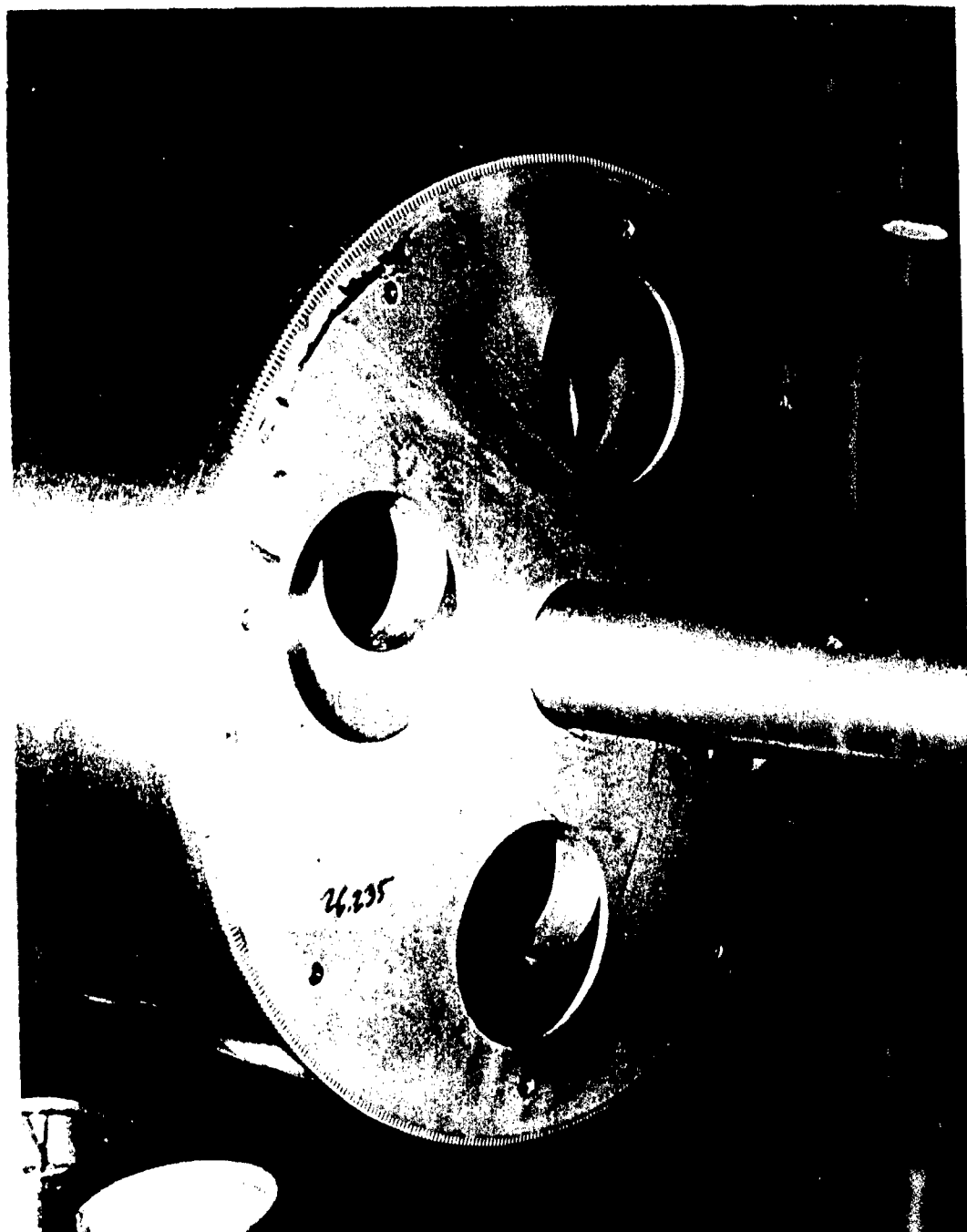
Figure 36 shows wheels at the ends of cylindrical mandrel serve as attachment points for the lead mounted films. Several sets of pinwheels with different diameters are employed during the winding process. As the thickness of the wound layer increases, pinwheels with larger diameters are used for the purpose of pinwheels with smaller diameter.
