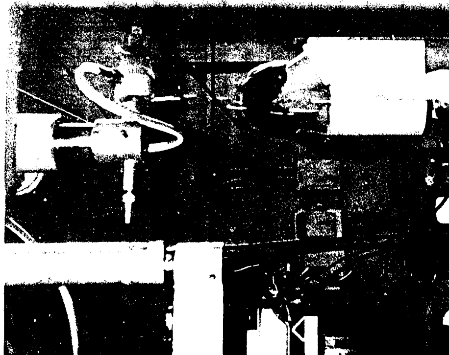
Figure 53. Set up for sonic scanning of the full-scale AUSS cylinder by transmitted acoustic energy. Jets of water are used to couple the acoustic signal with the surfaces of the cylinder
