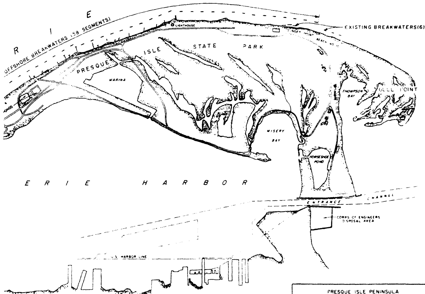
BREAKWATER PLAN
