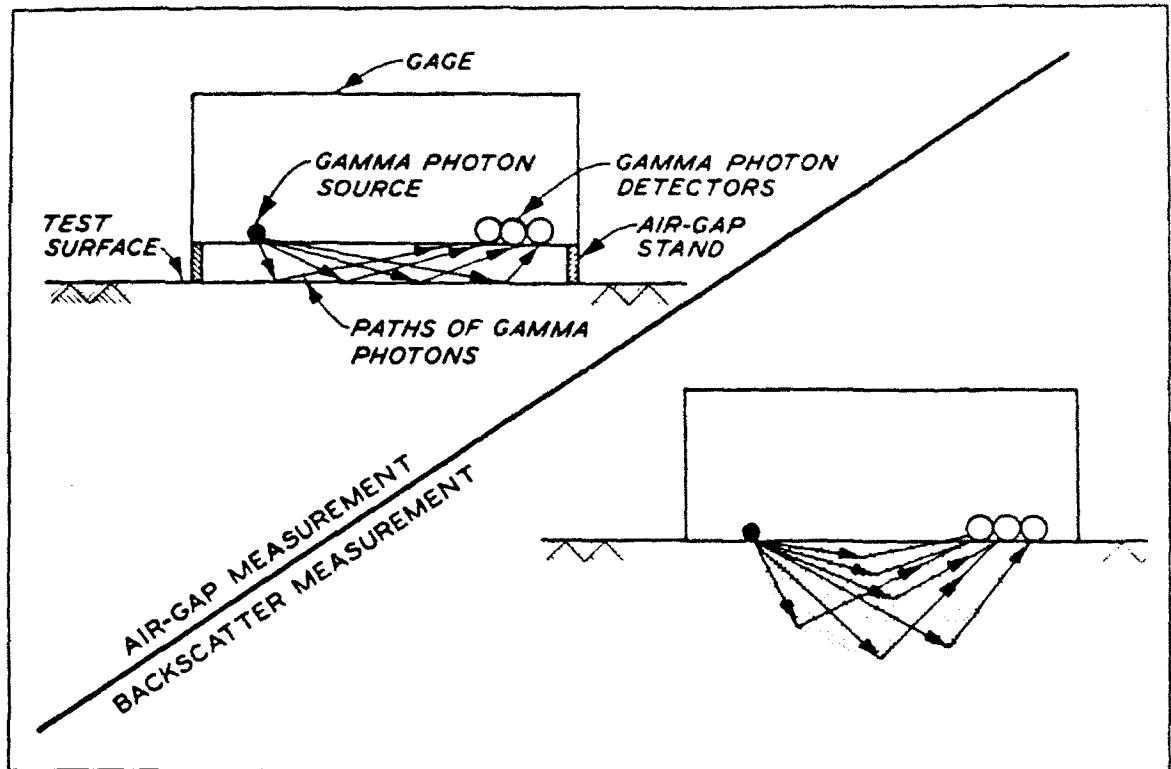
Figure 3. Air-gap versus backscatter density measurement
