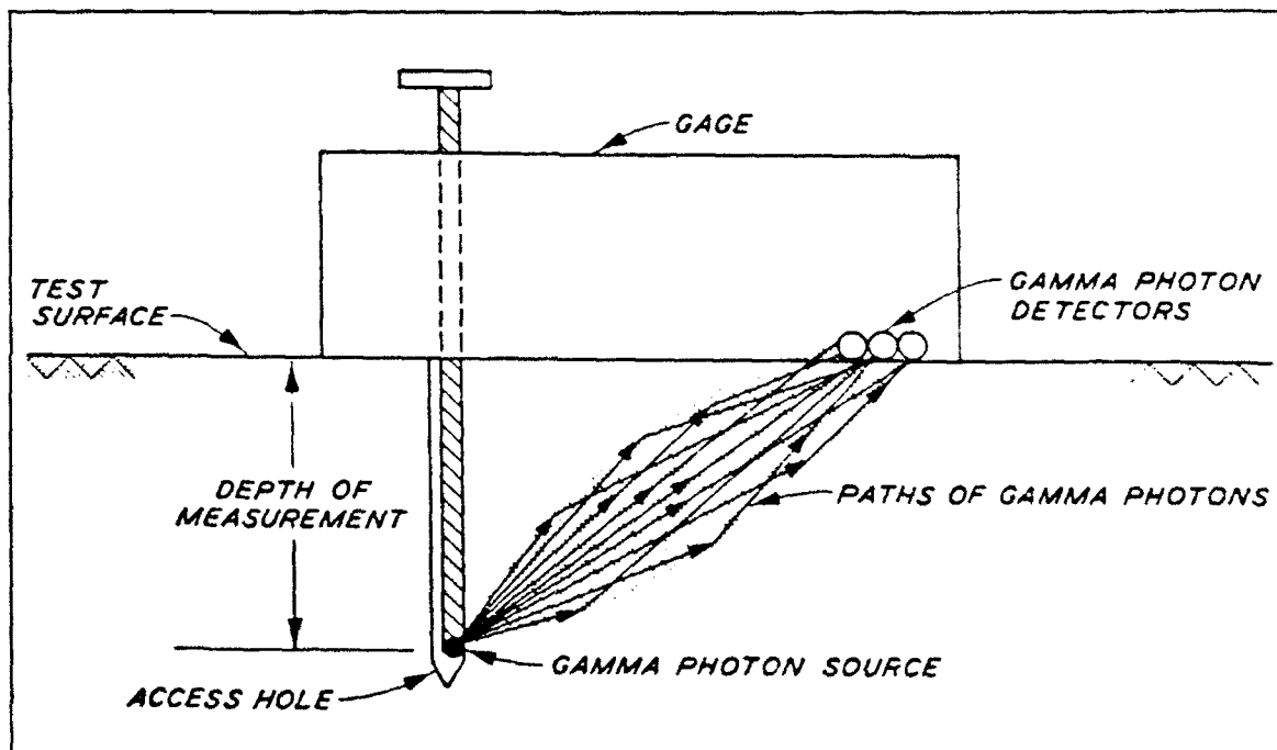
Figure 1. Direct transmission density measurement
