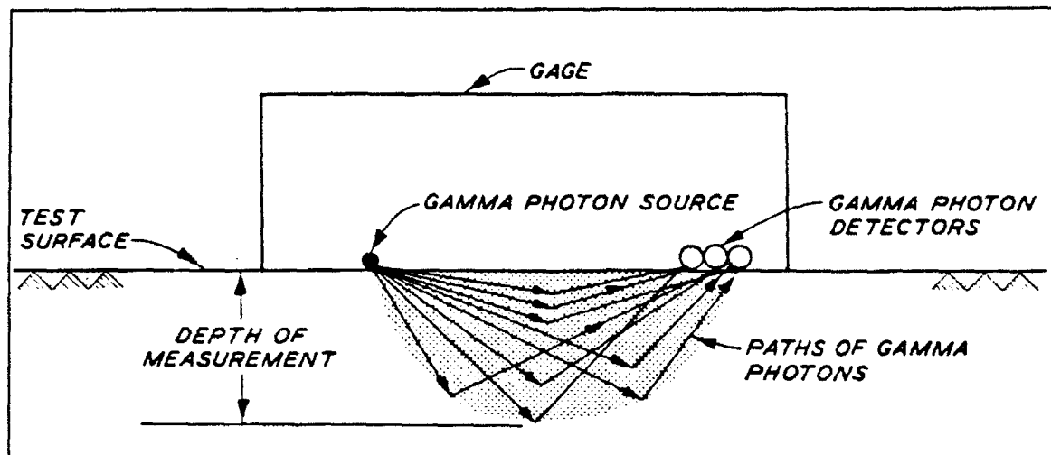
Figure 2. Backscatter density measurement
