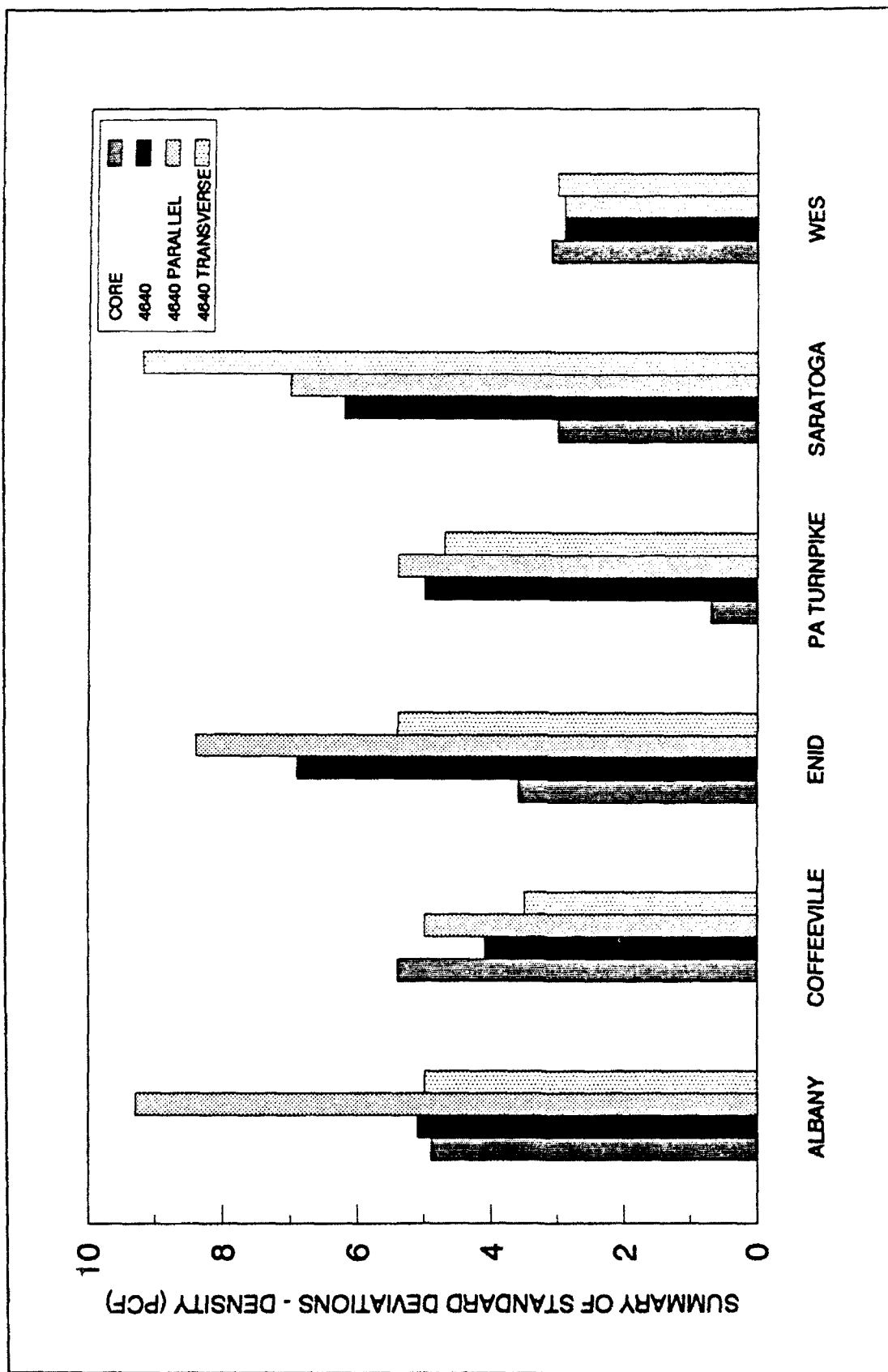
Figure 6. 4640 Gauge - Standard Deviations of Densities
