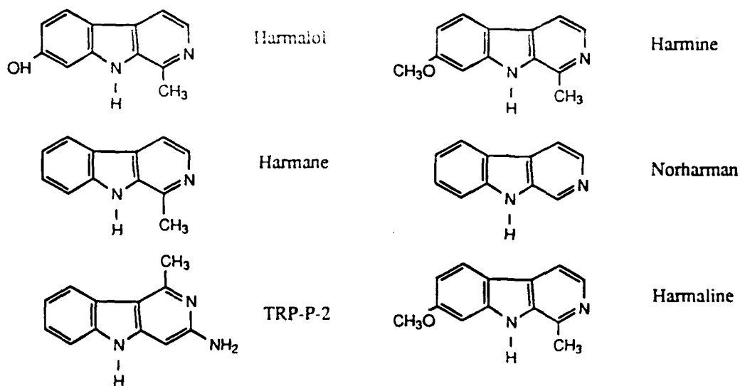
Figure 3. Chemical structure of harmaline and related compounds.
