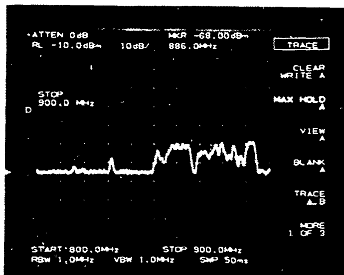
(b) Radio Telephone Spectrum
