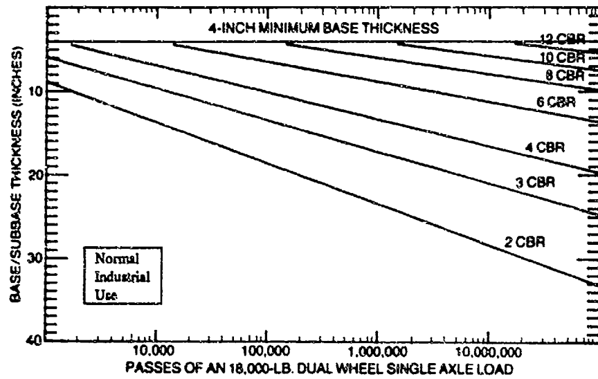
(a) Design Curves for 18 kip ESAL's
