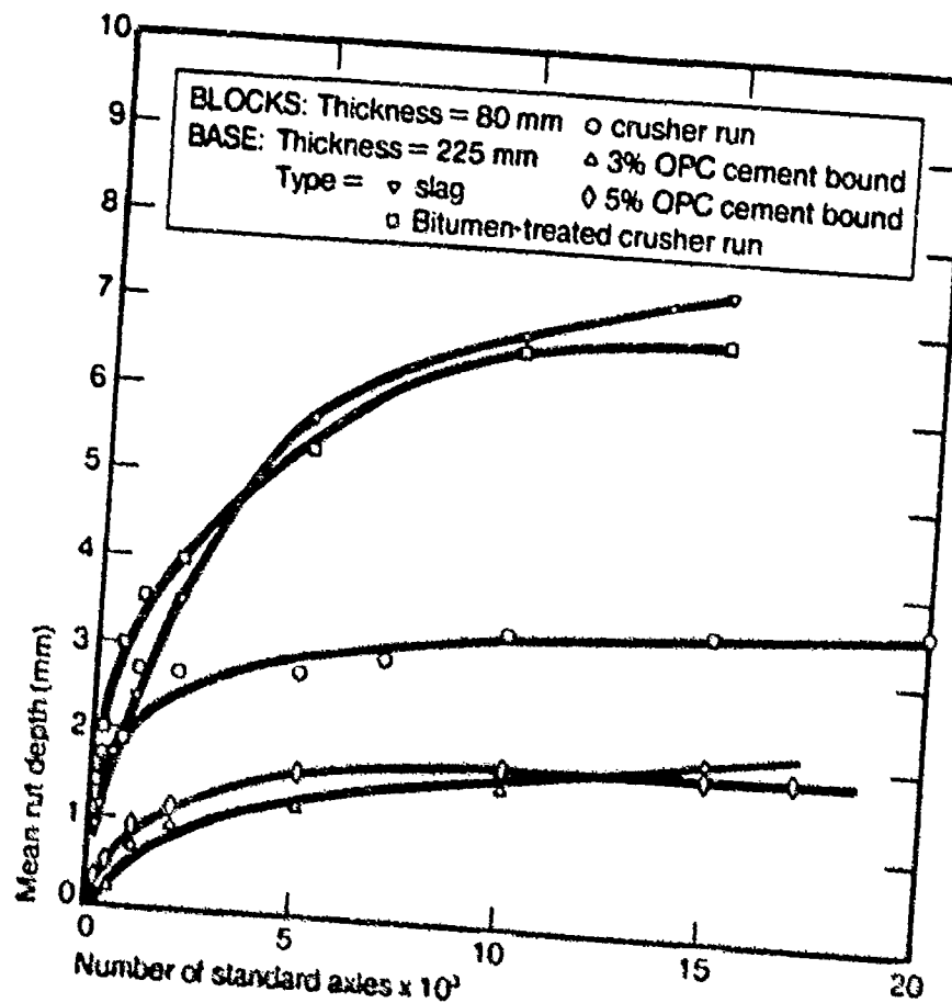
Figure 3.1. The Effects of the Type of Base Course on the Performance of CBP Under Traffic, OPC = Ordinary Portland Cement (Shackel [1])
