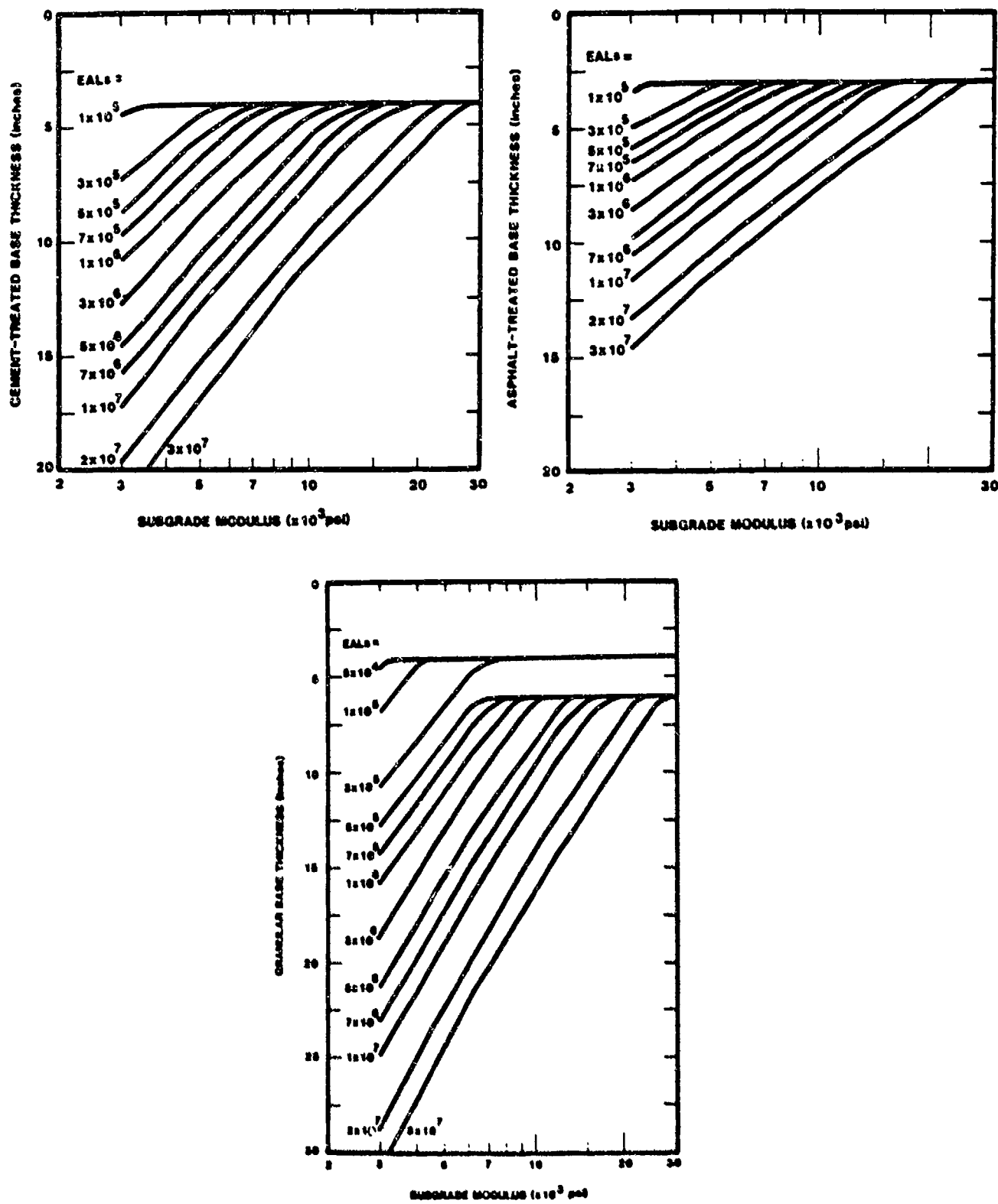
Figure 3.4. Base Thickness Design Curves (Rada [5])
