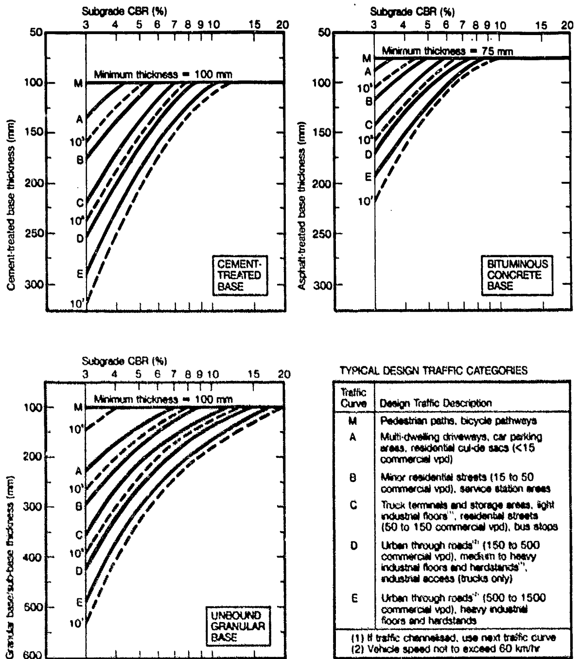
Figure 3.2. NCMA CBP Structural Design Curves (Shackel [1])
