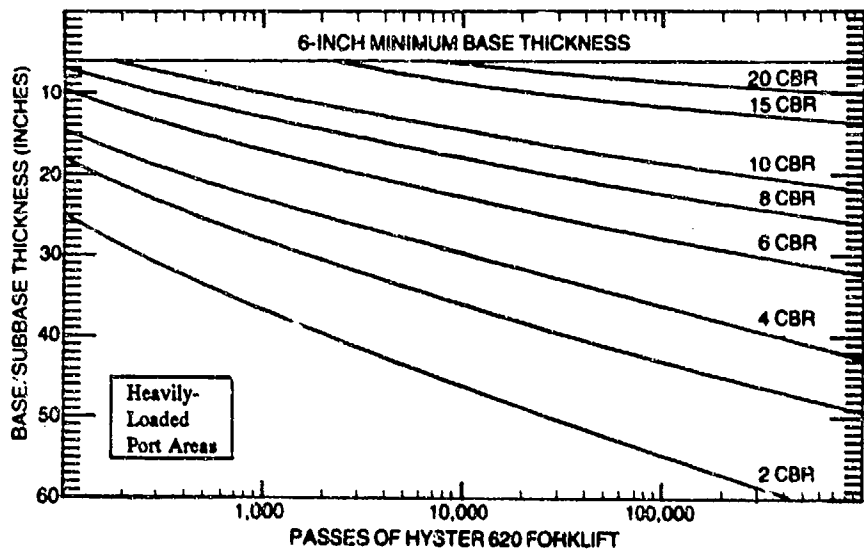
(b) Design Curves for Hyster 620 Forklift
