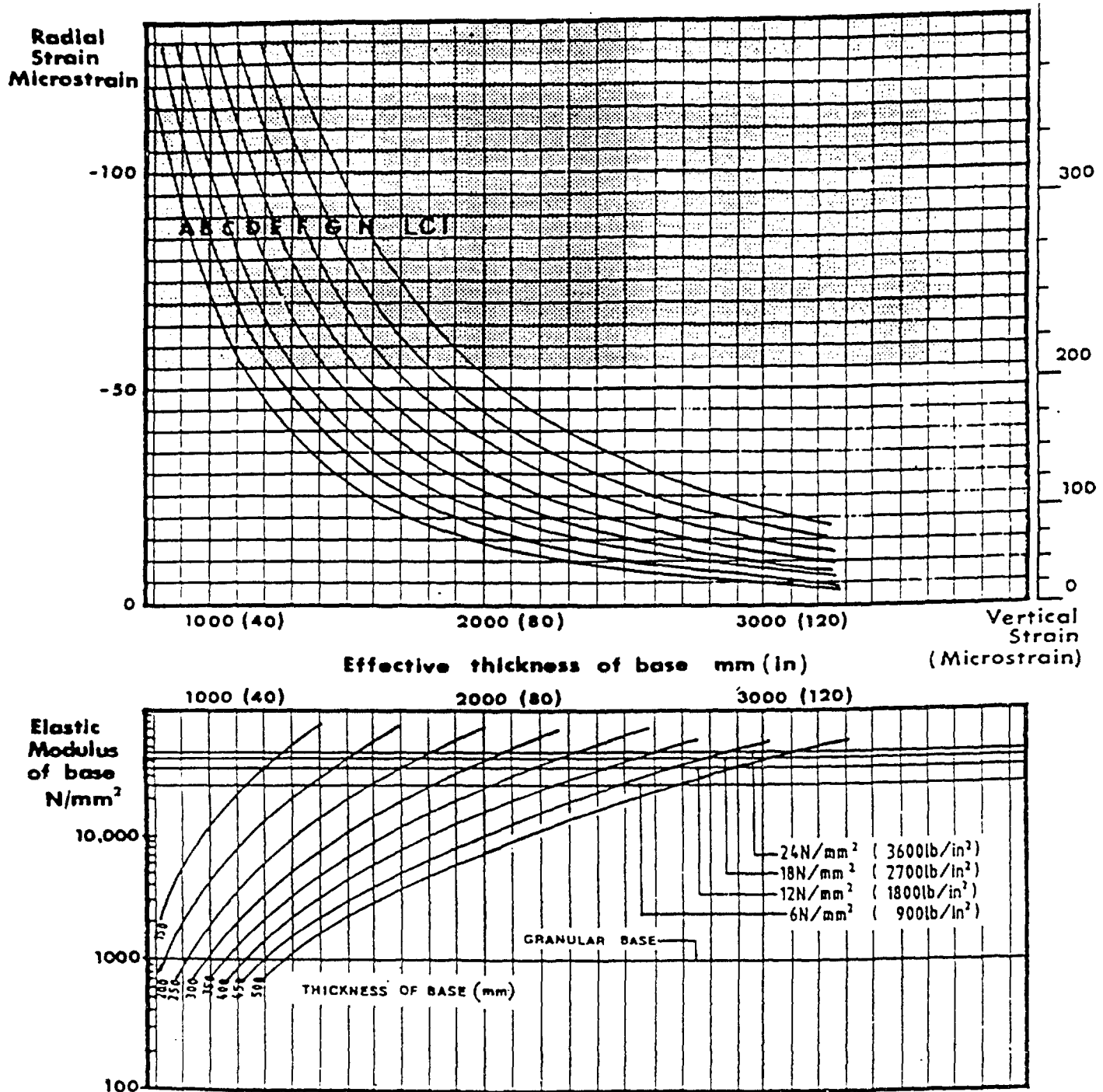
Figure 3.5(b). Design Curves for 10% CBR Subgrade and 12 inch Subbase (CPI [17])
