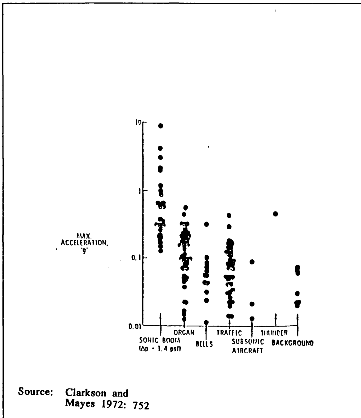
FIGURE IV-3 Response of Cathedral Windows to Transient Pressure
