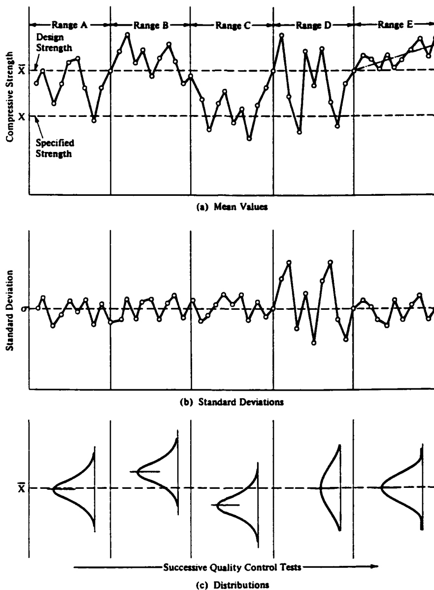
Figure 32 Control charts for mean and standard deviation.
