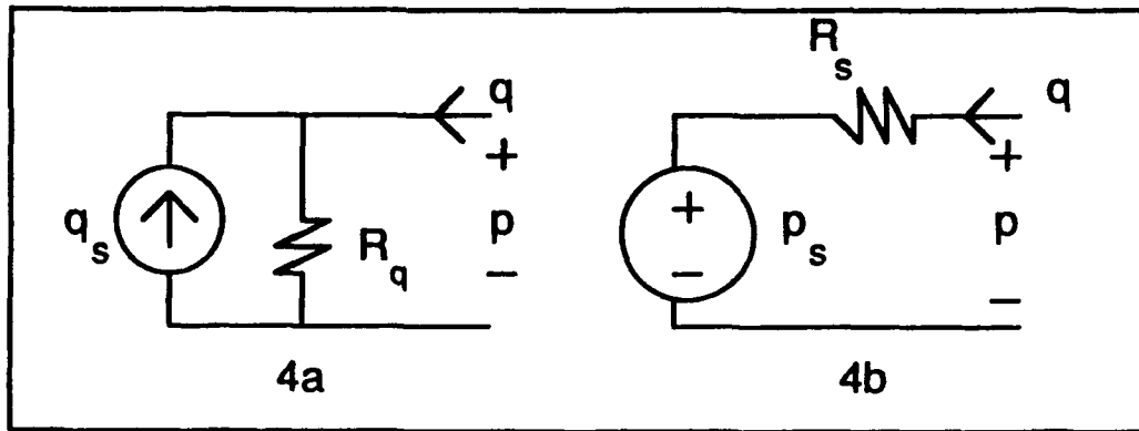
Figure 2.4: Alternative source arrangements for the development of the Flow source ↔ Pressure source transformation.
