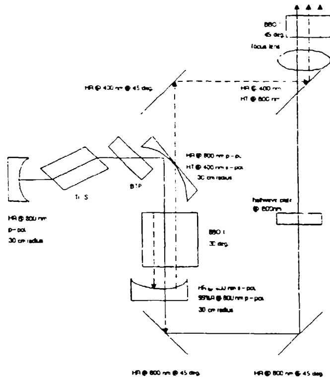
Figure B-4. External type I sum-frequency mixing.
