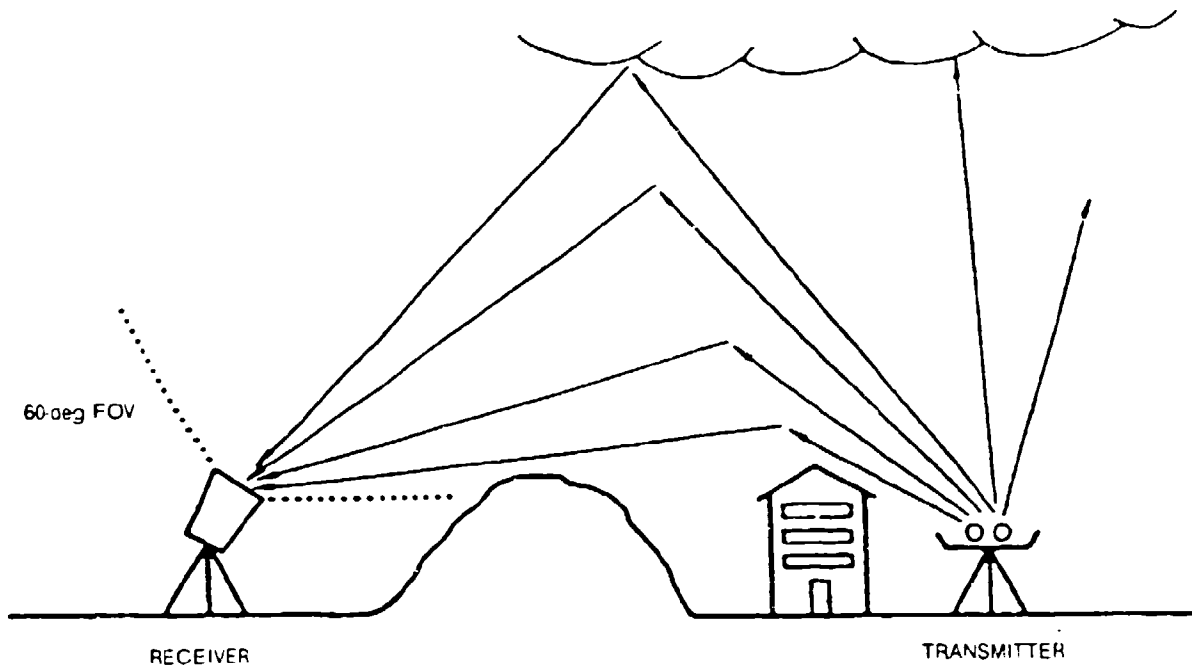
Figure J-1. UV Comm configuration.
