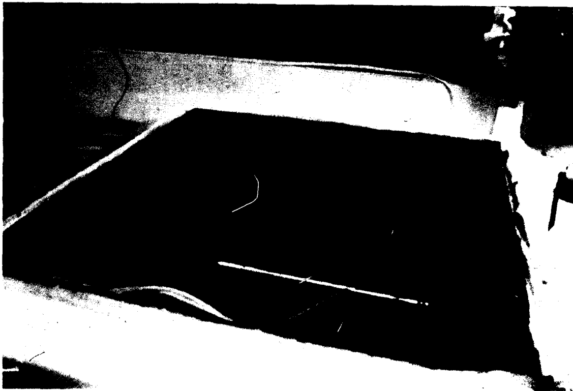
FIGURE 12- CLOSE-UP VIEW OF THERMAL ENCLOSURE
