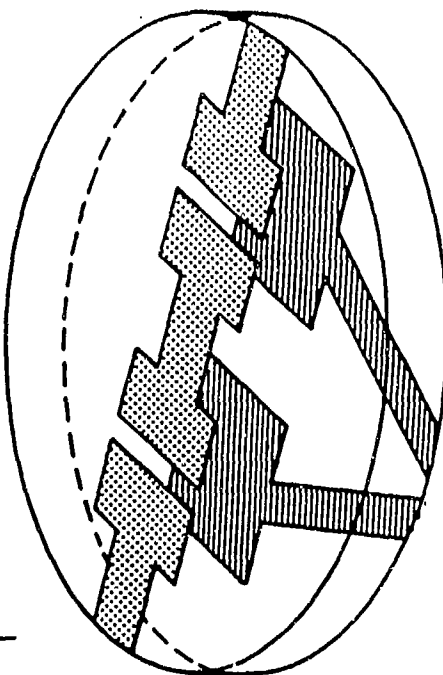
Four-pole filter electrode arrangement
