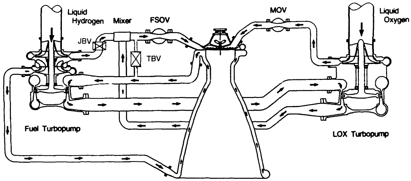
Figure 7. Split-Expander Cycle
