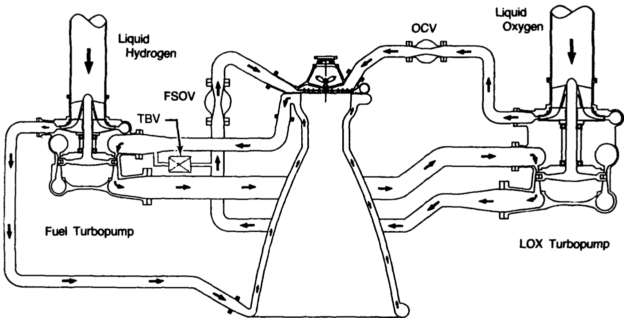
Figure 5. Full-Expander Cycle
