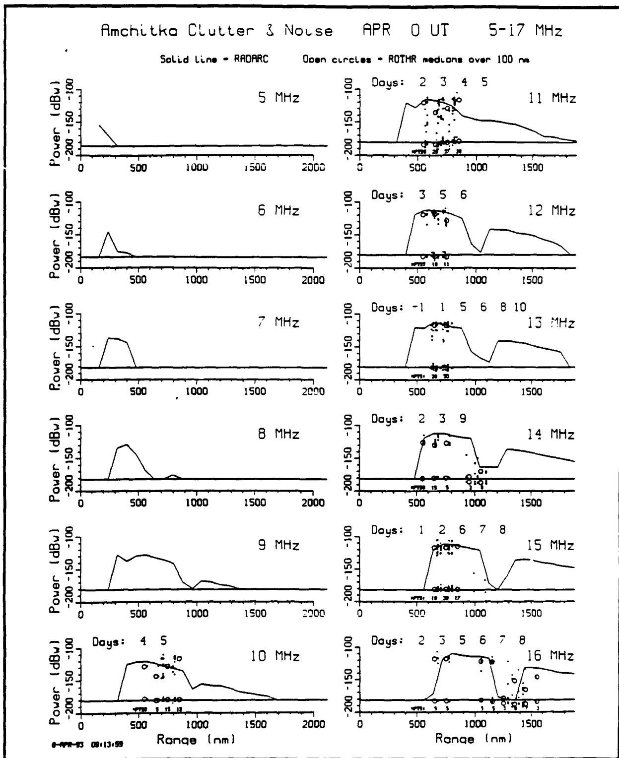
Figure 5.4. Radar backscatter power vs. range. Dots are ROTHF data points (peaks and noise) from Amchitka. Circles are medians of data points over 100 nm intervals. Solid lines are RADARC predictions (version 2.0). Data is for April 1991, 0 UT (local daytime), 5-17 MHz, 0 to 10 degrees with respect to boresight. Each subplot is a 1 MHz band.
